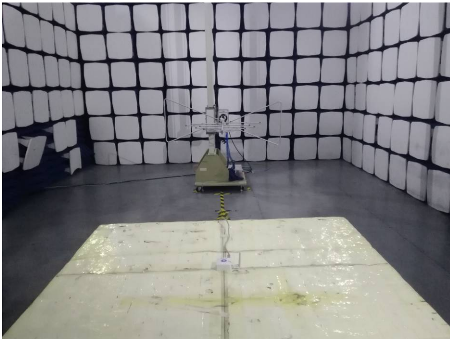
Radiated emission 30MHz~1GHz Powered by POE
