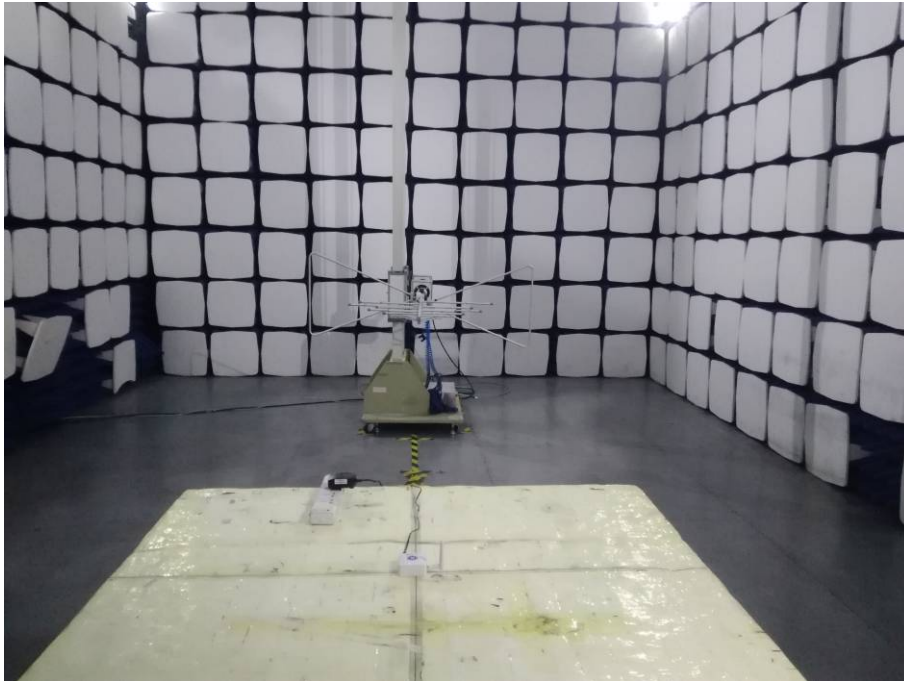
Radiated emission 30MHz~1GHz Powered by USB
