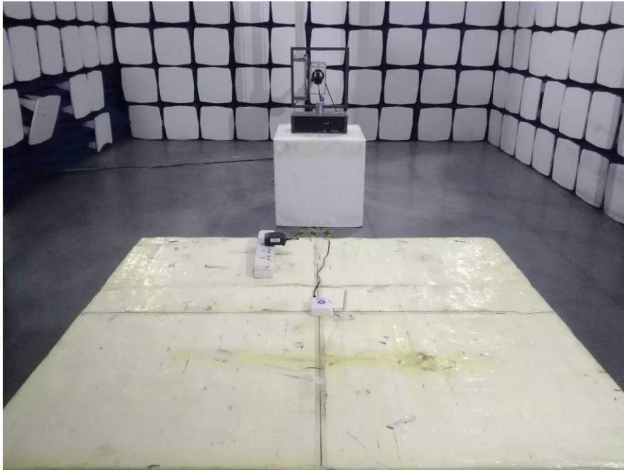
Radiated emission 30MHz Powered by USB
