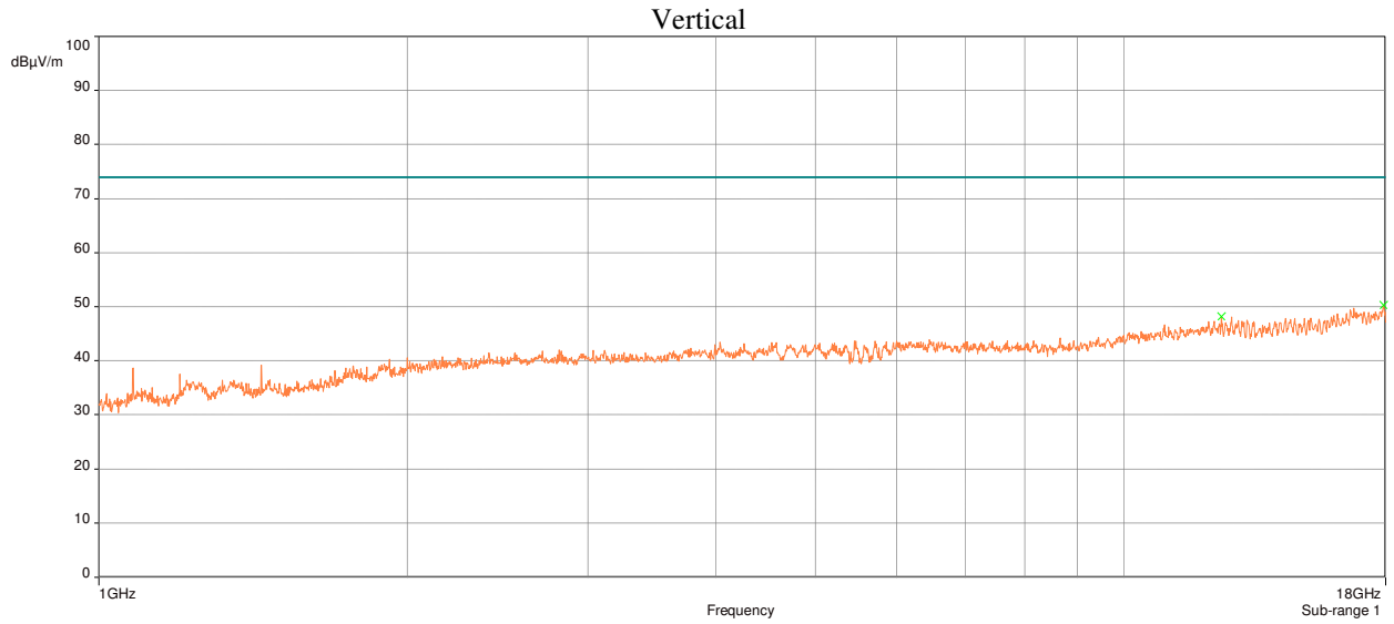
Plot 18: Radiated Spurious Emissions Requirements, 802.11a, Mid Channel UNII-2, Peak
