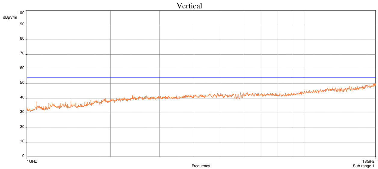
Plot 33: Radiated Spurious Emissions Requirements, 802.11a, High Channel UNII-3, Average
