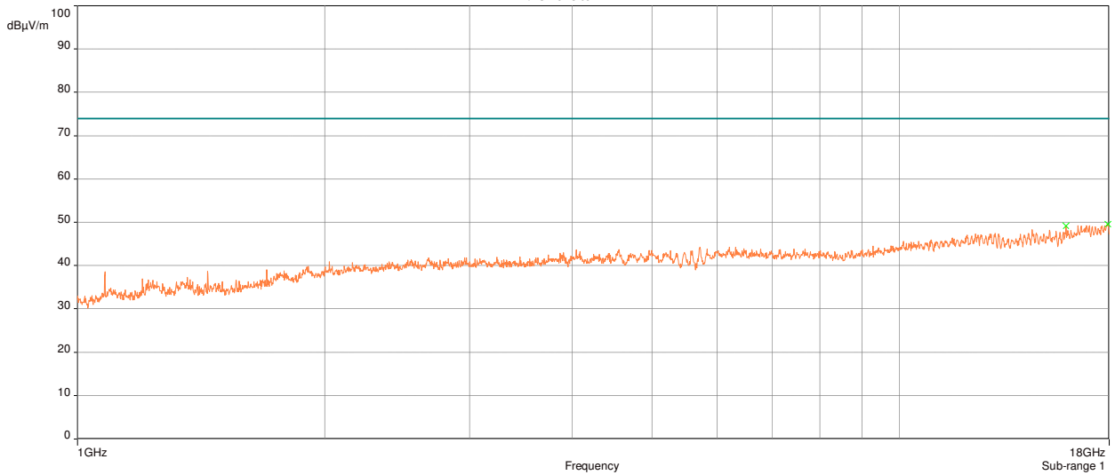
Plot 24: Radiated Spurious Emissions Requirements, 802.11n, Mid Channel UNII-2, Peak
