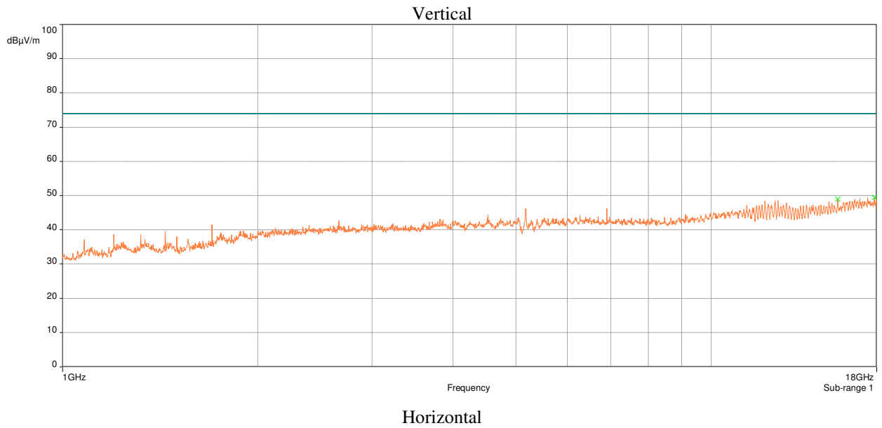
Plot 10: Radiated Spurious Emissions Requirements, 802.11n, Low Channel UNII-1, Peak
