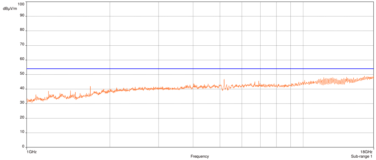
Plot 11: Radiated Spurious Emissions Requirements, 802.11n, Low Channel UNII-1, Average
