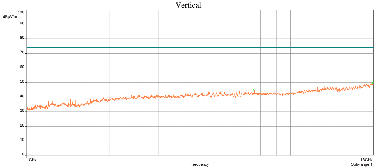
Plot 38: Radiated Spurious Emissions Requirements, 802.11n, High Channel UNII-3, Peak
