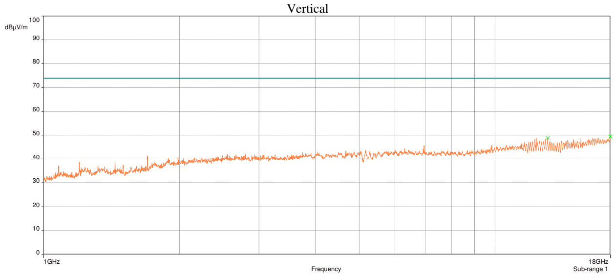
Plot 6: Radiated Spurious Emissions Requirements, 802.11a, Mid Channel UNII-1, Peak
