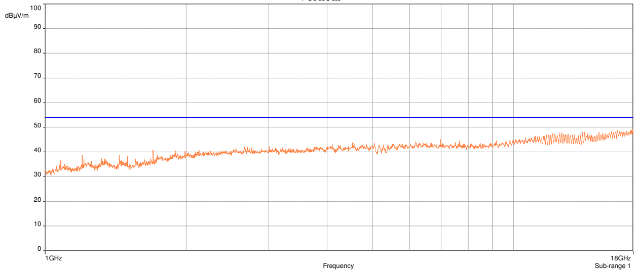
Plot 15: Radiated Spurious Emissions Requirements, 802.11n, High Channel UNII-1, Average
