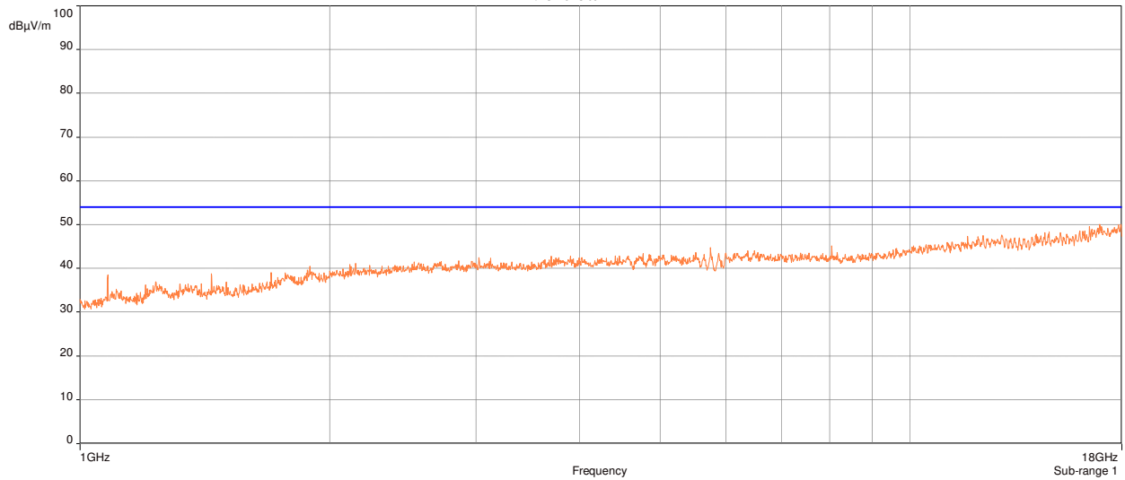
Plot 29: Radiated Spurious Emissions Requirements, 802.11a, Low Channel UNII-3, Average
