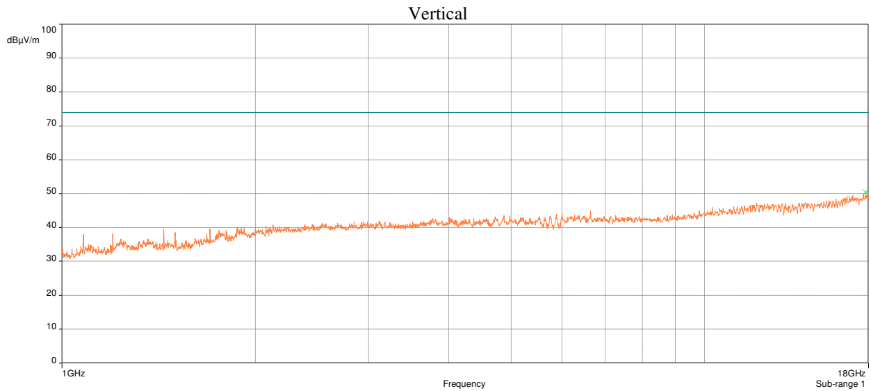
Plot 32: Radiated Spurious Emissions Requirements, 802.11a, High Channel UNII-3, Peak
