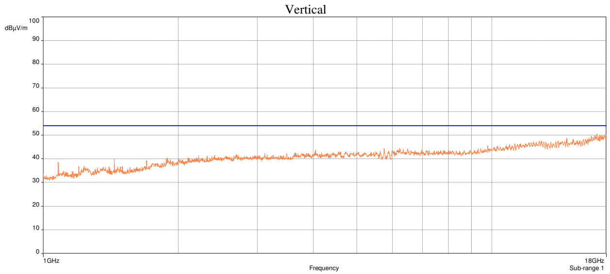
Plot 31: Radiated Spurious Emissions Requirements, 802.11a, Mid Channel UNII-3, Average
