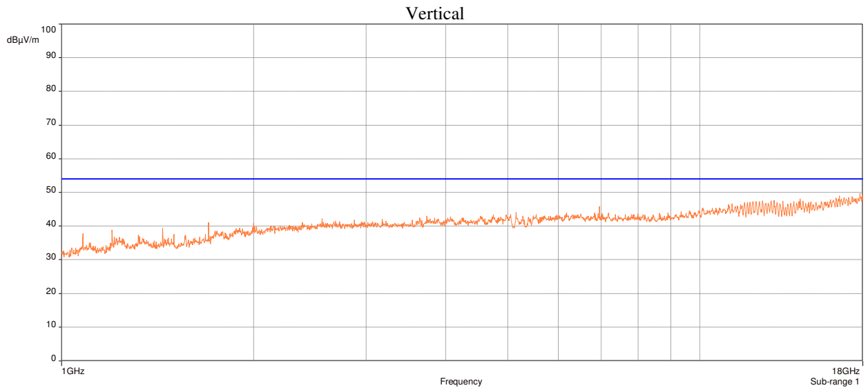
Plot 7: Radiated Spurious Emissions Requirements, 802.11a, Mid Channel UNII-1, Average
