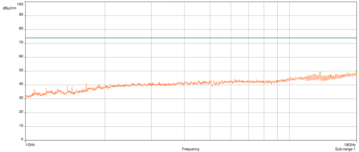
Plot 4: Radiated Spurious Emissions Requirements, 802.11a, Low Channel UNII-1, Peak
