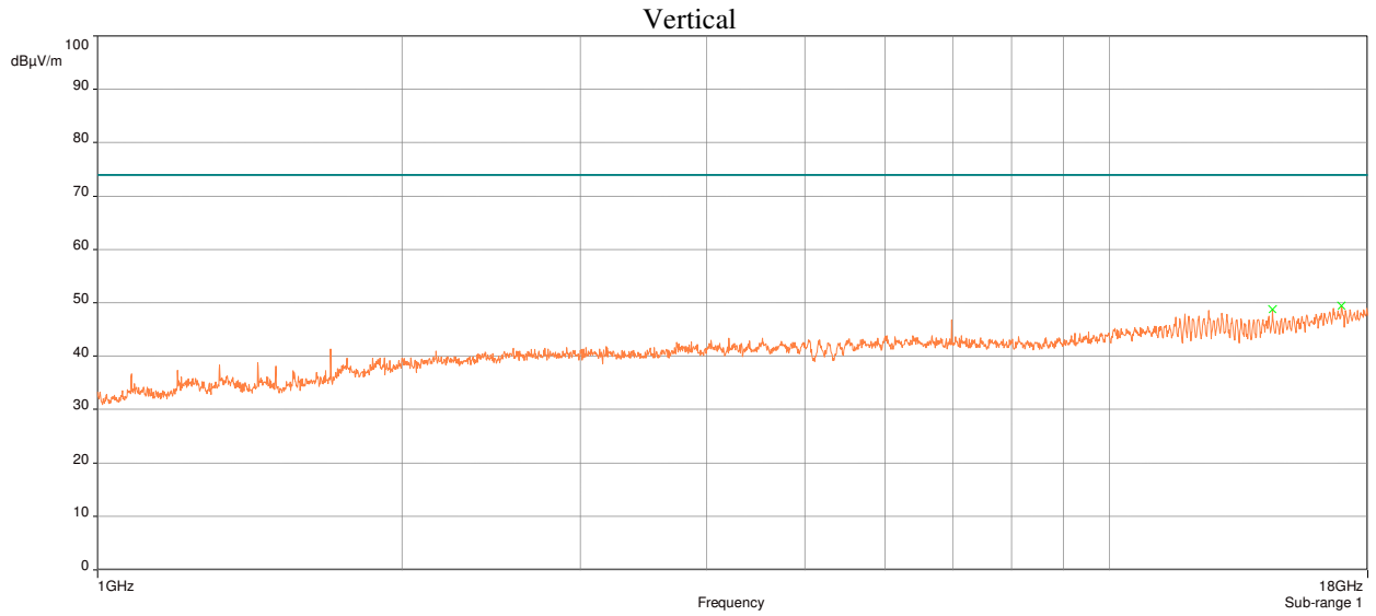
Plot 8: Radiated Spurious Emissions Requirements, 802.11a, High Channel UNII-1, Peak
