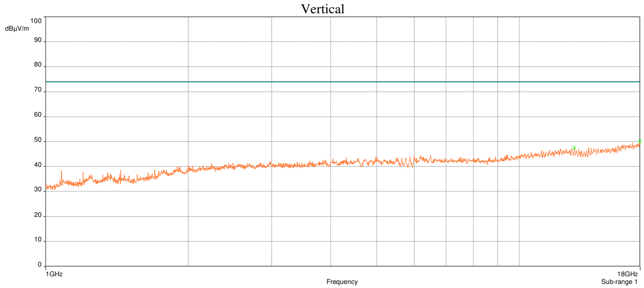
Plot 36: Radiated Spurious Emissions Requirements, 802.11n, Mid Channel UNII-3, Peak
