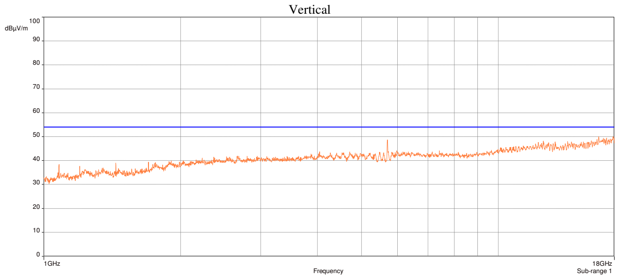
Plot 21: Radiated Spurious Emissions Requirements, 802.11a, High Channel UNII-2, Average
