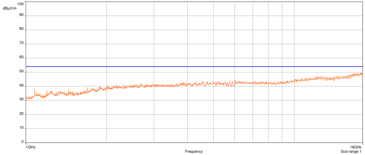
Plot 39: Radiated Spurious Emissions Requirements, 802.11n, High Channel UNII-3, Average
