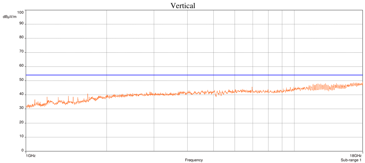
Plot 13: Radiated Spurious Emissions Requirements, 802.11n, Mid Channel UNII-1, Average
