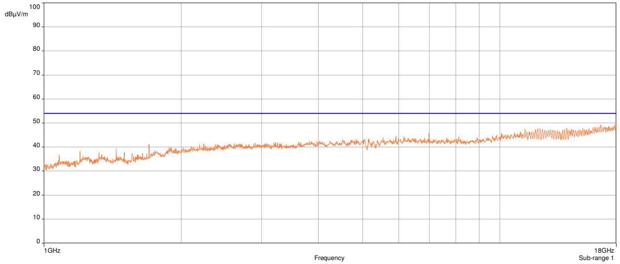
Plot 9: Radiated Spurious Emissions Requirements, 802.11a, High Channel UNII-1, Average
