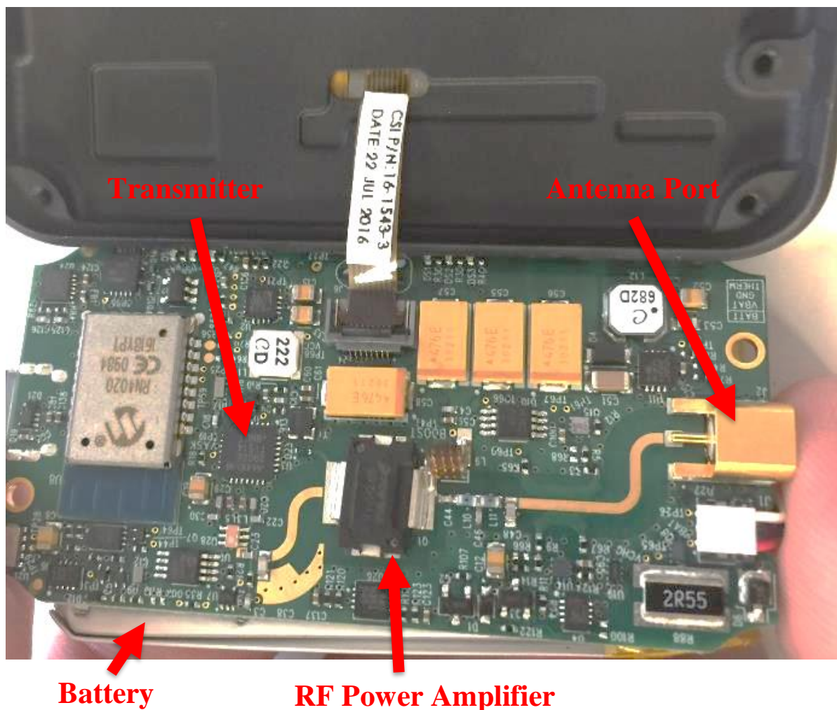
Figure 1. Overhead view of the Internals of the PDBT-2
