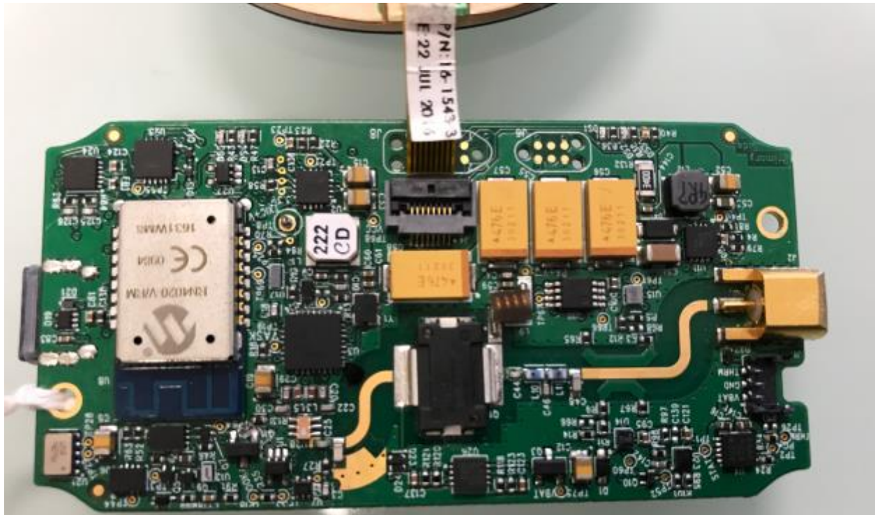
Figure 2. Top Side of the PDBT-2 Circuit board
