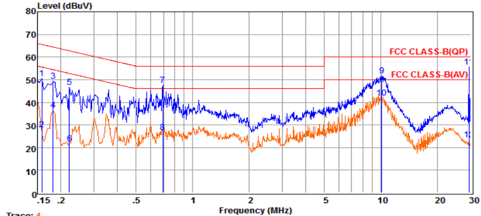
Trace: 4
