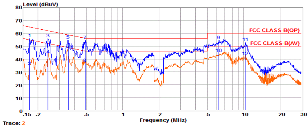
Trace: 2
