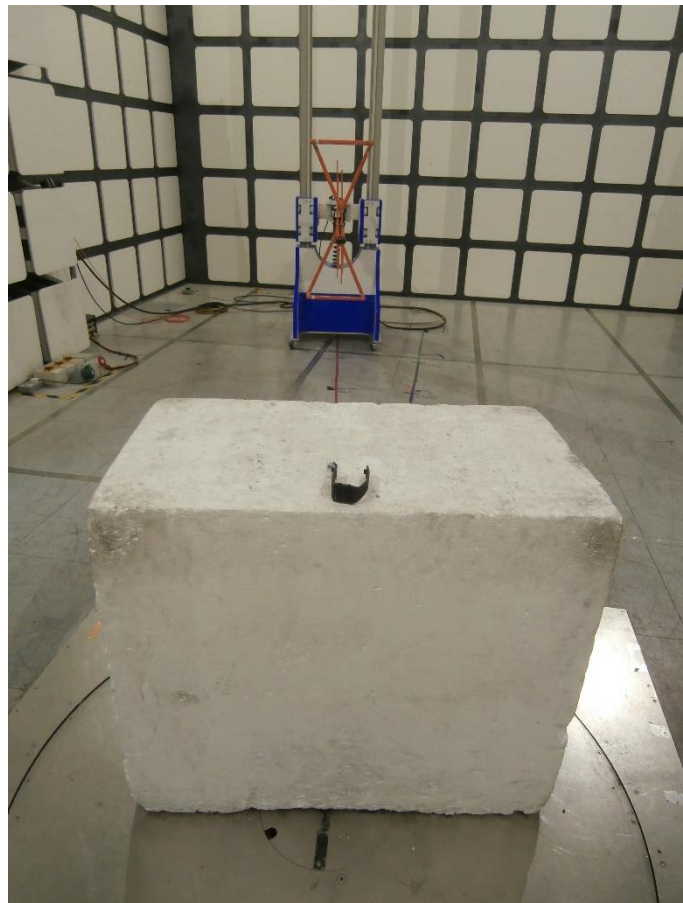
Figure 11 – 30 MHz to 1 GHz
