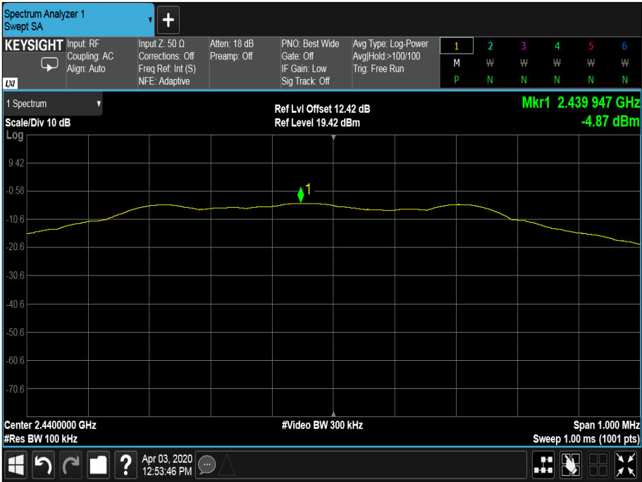
Figure 69 - 2440 MHz
