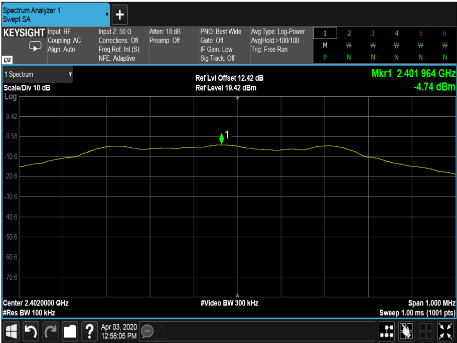
Figure 68 - 2402 MHz
