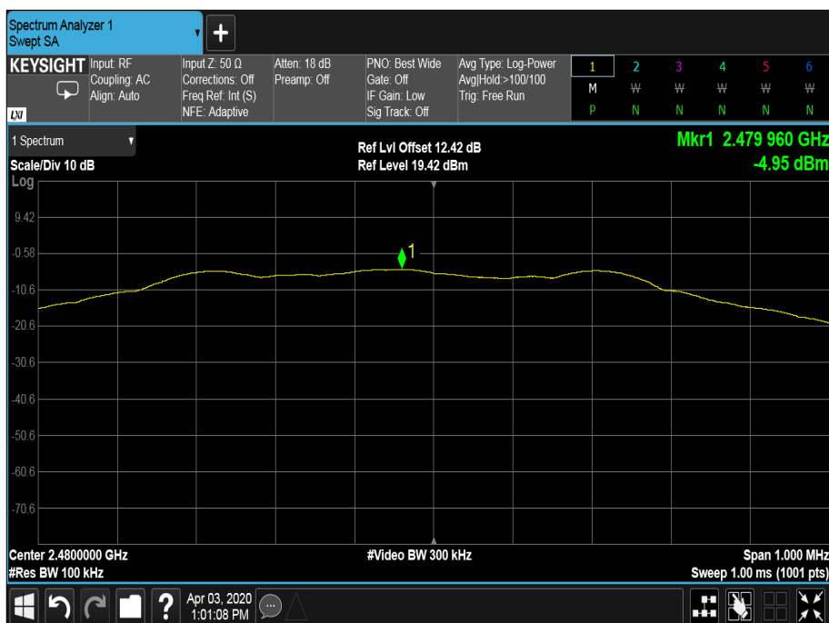
Figure 70 - 2480 MHz
