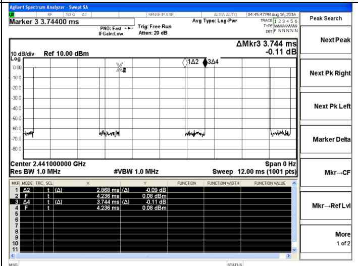
2DH5-2441MHz
