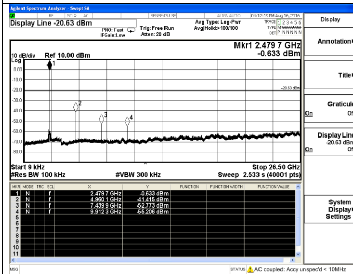
2DH1-High channel
