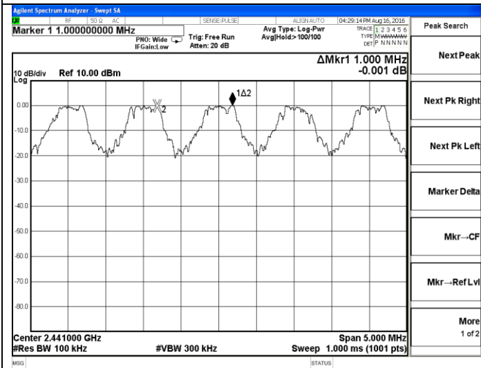
GFSK-Middle channel
