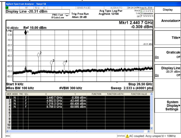
2DH1-Middle channel
