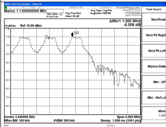
GFSK-High channel
