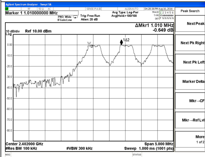
GFSK-Low channel
