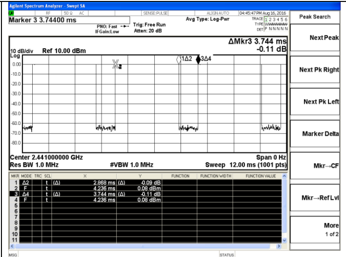
2DH1-2441MHz
