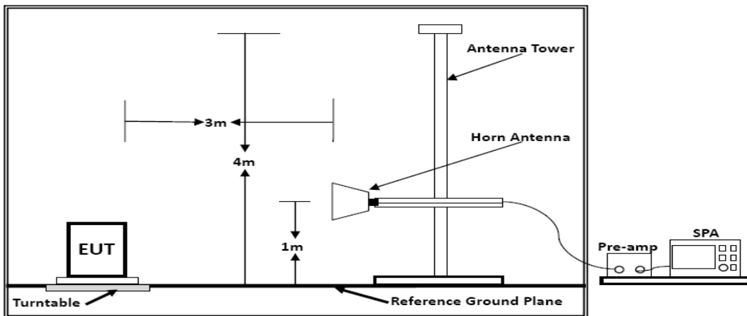
Above 1GHz
