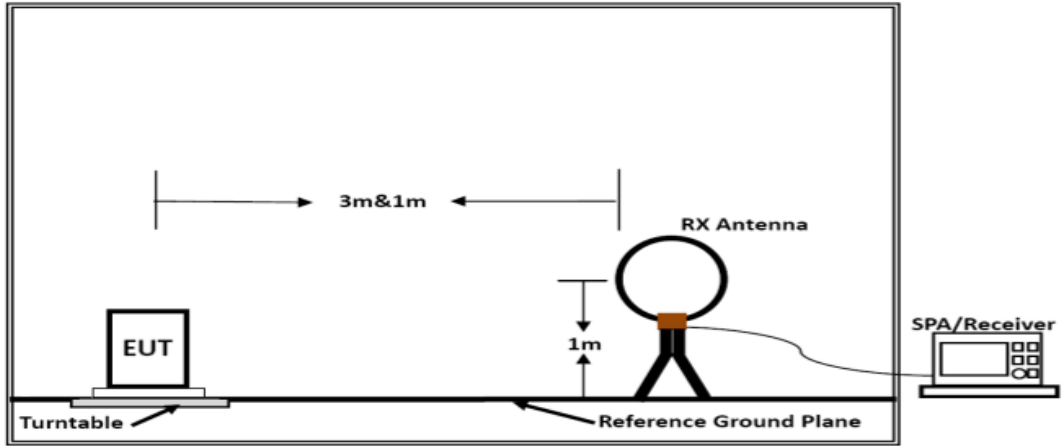
Below 30MHz
