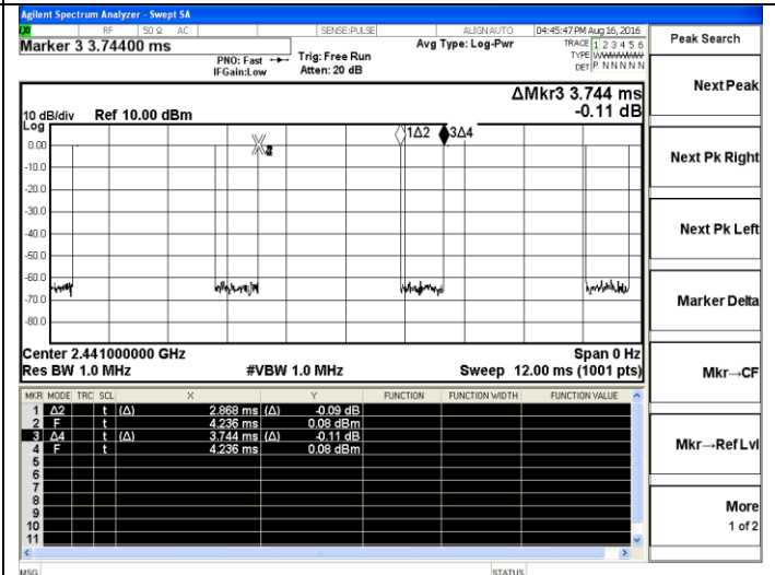
2DH3-2441MHz
