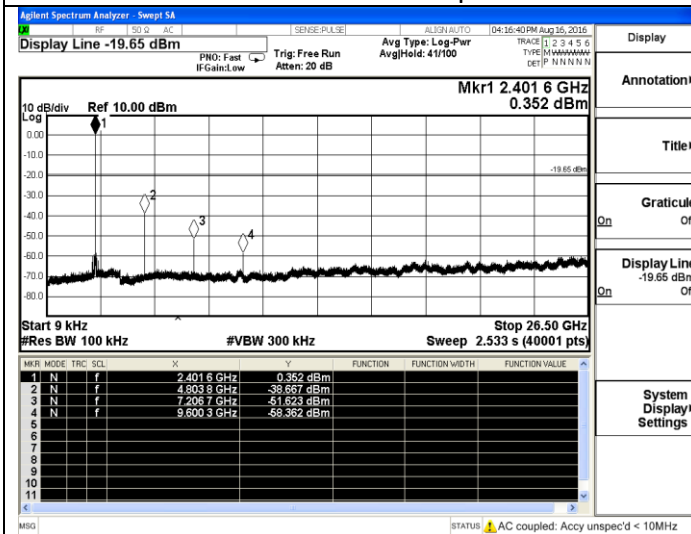
2DH1-Low channel
