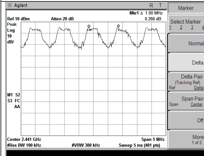
GFSK-Middle channel
