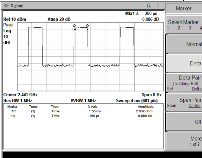
DH1-2441MHz
