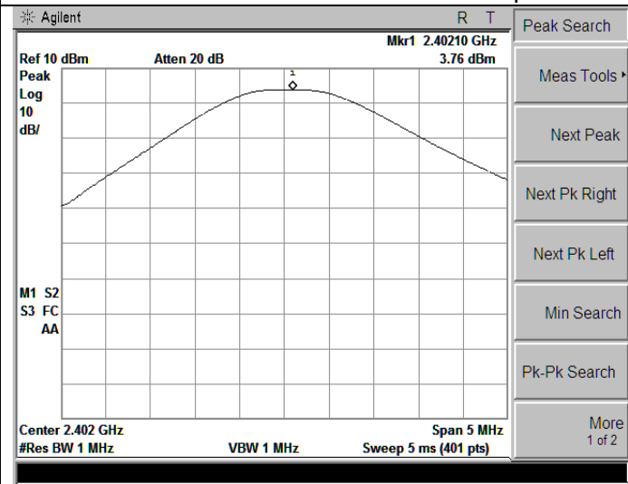
DH1-Low channel
