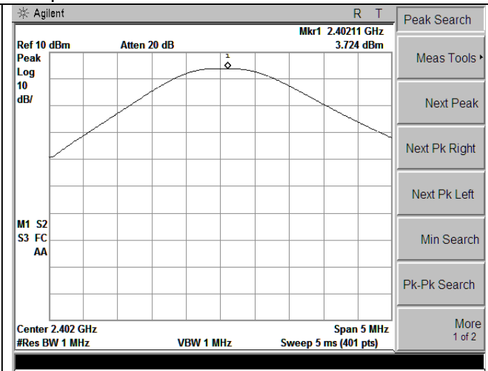
2DH1-Low channel
