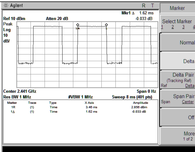
DH3-2441MHz
