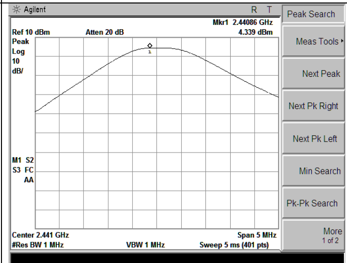
2DH1-Middle channel
