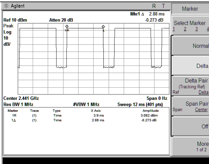
DH5-2441MHz
