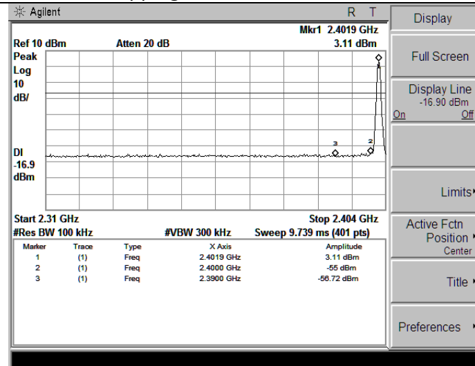
Hopping Off-GFSK-Low channel
