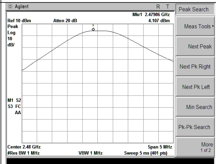
2DH1-High channel
