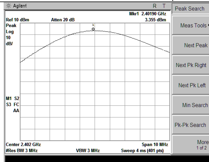
DH1-Low channel
