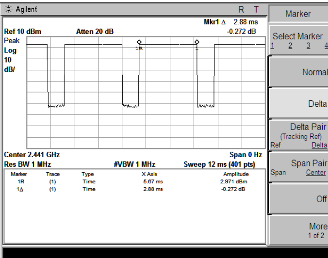
DH5-2441MHz
