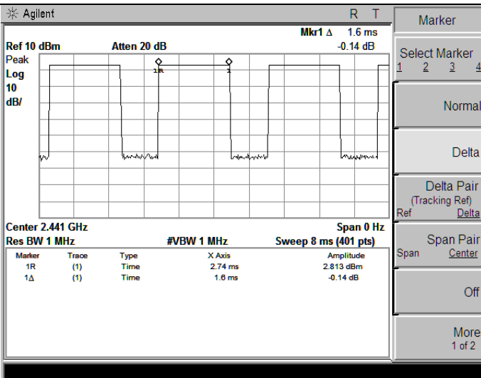
DH3-2441MHz
