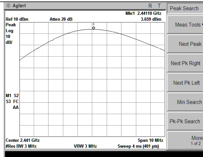
DH1-Middle channel
