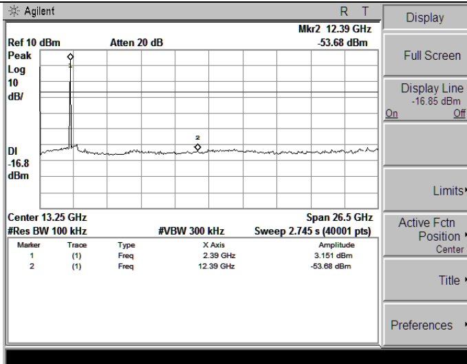
DH1-Low channel
