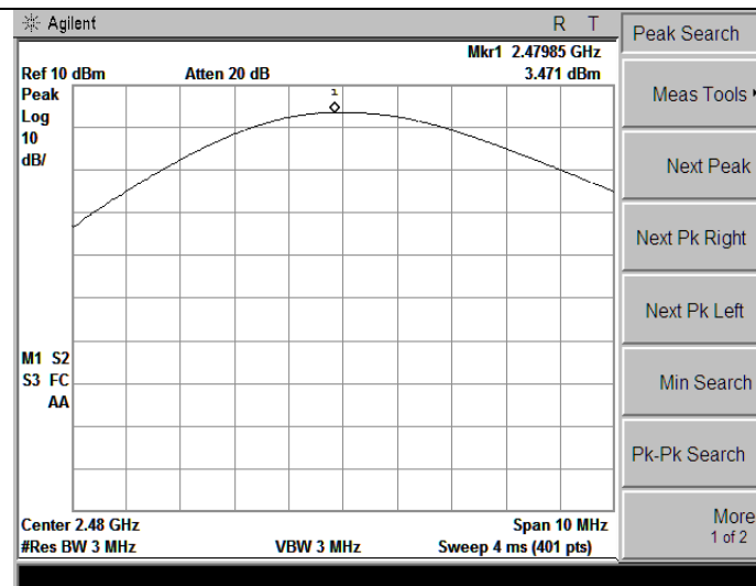
DH1-High channel
