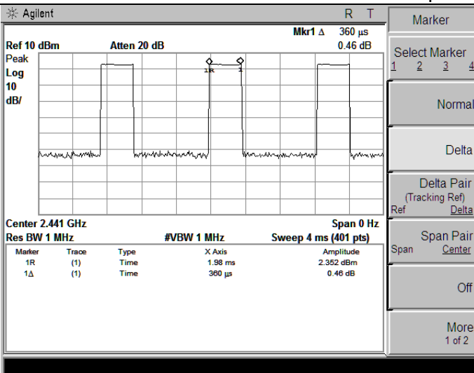
DH1-2441MHz
