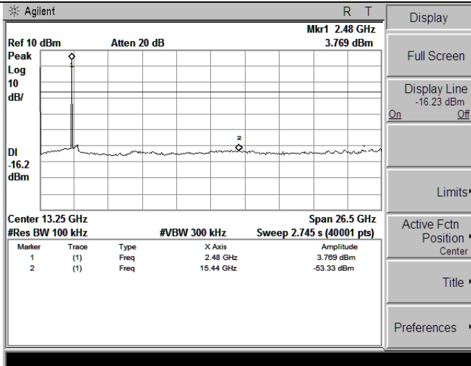
DH1-High channel
