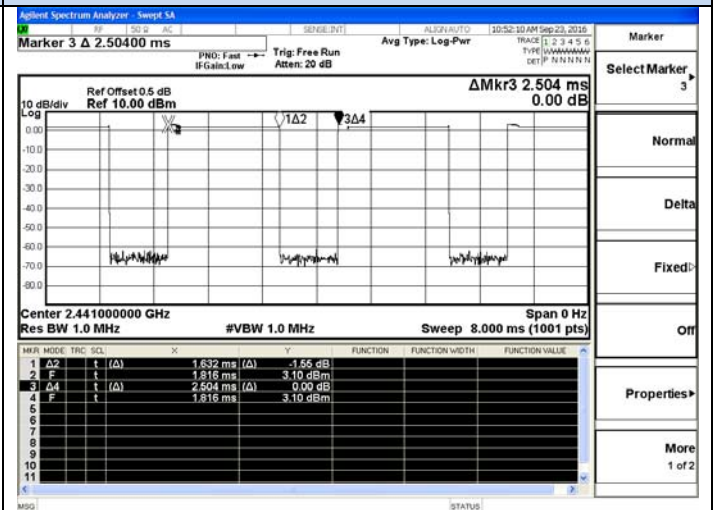
2DH3-2441MHz
