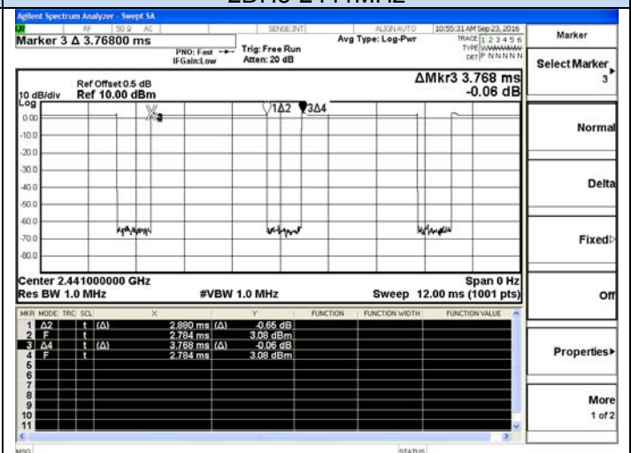
2DH5-2441MHz
