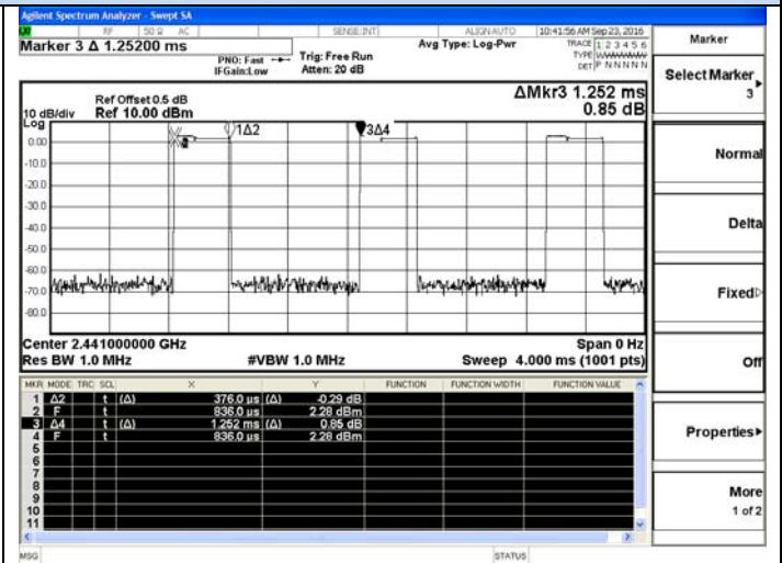
2DH1-2441MHz
