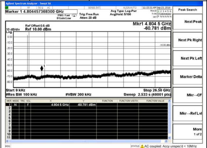
2DH1-Low channel
