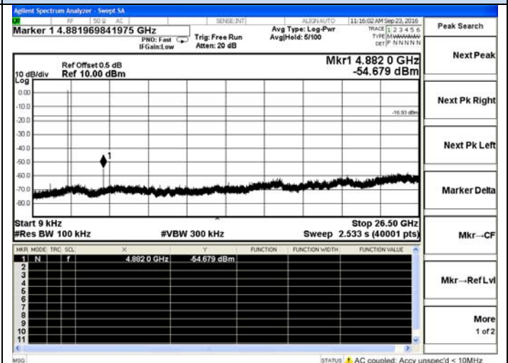
2DH1-Middle channel
