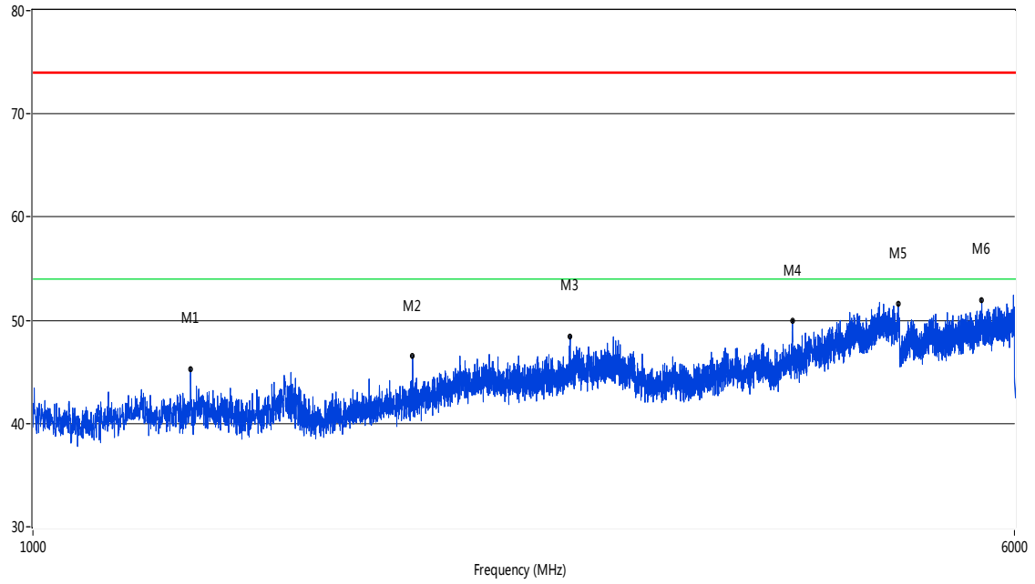
RE Test case_FCC_Part 15B_FCC Part15B ClassB 1GHz-6GHz
