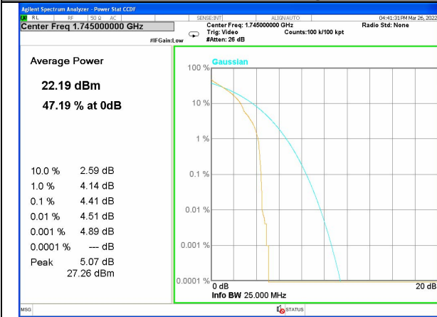
Band 4_1_Q16_High
