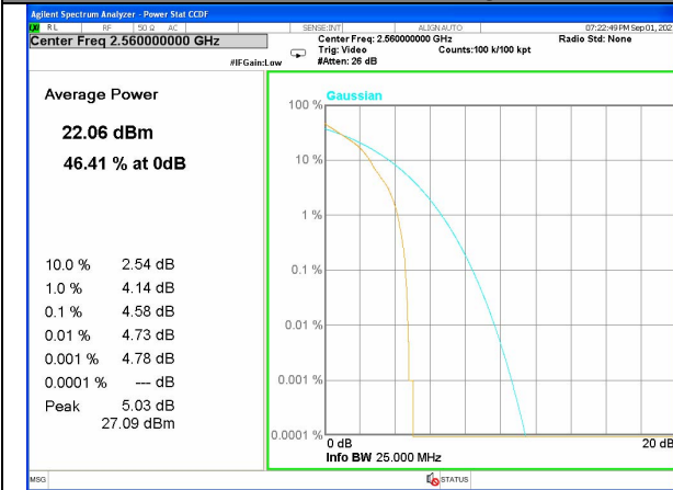
Band 7_1_Q16_High
