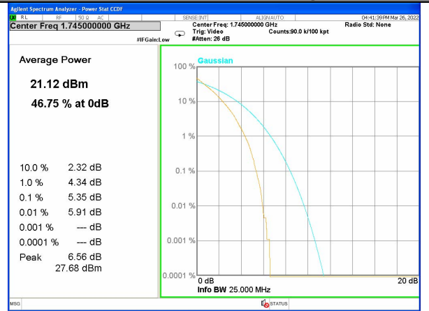
Band 4_100_Q16_High
