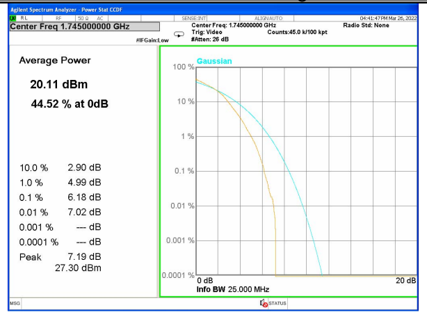
Band 4_100_Q16_High
