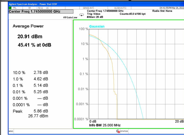
Band 4_1_Q16_High
