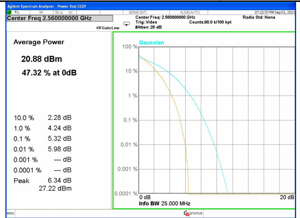
Band 7_100_Q16_High
