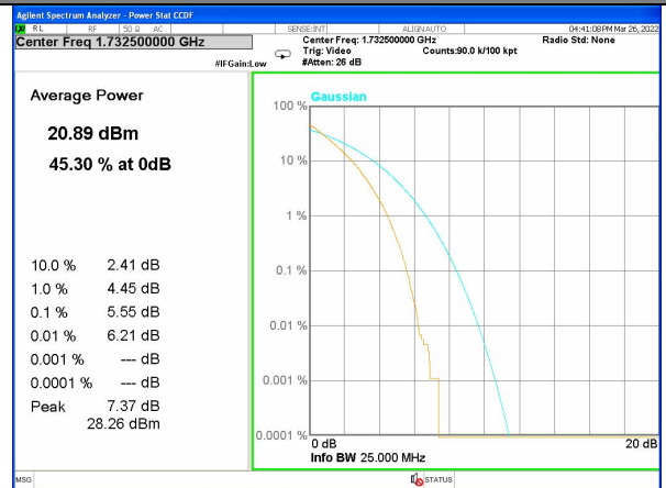
Band 4_100_QPSK_Middle
