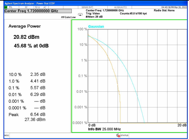
Band 4_100_Q16_Low
