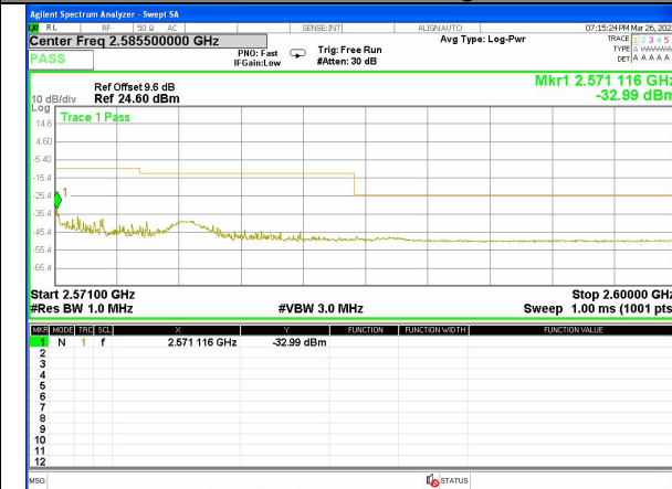
Band 7_20M_QPSK_High_Full-RB
