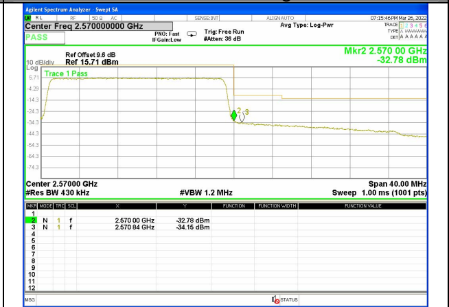
Band 7_20M_QPSK_High_Full-RB
