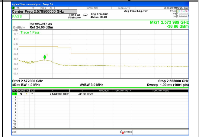
Band 7_5M_QPSK_High_1-RB
