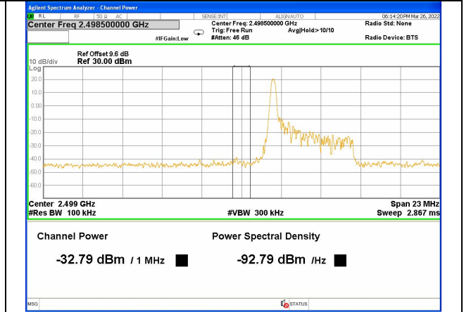
Band 7_5M_QPSK_Low_Full-RB
