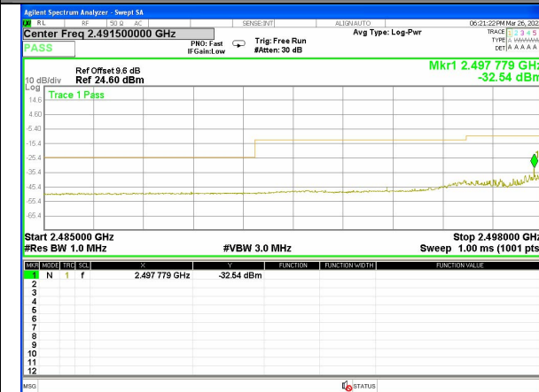
Band 7_5M_16QAM_Low_1-RB
