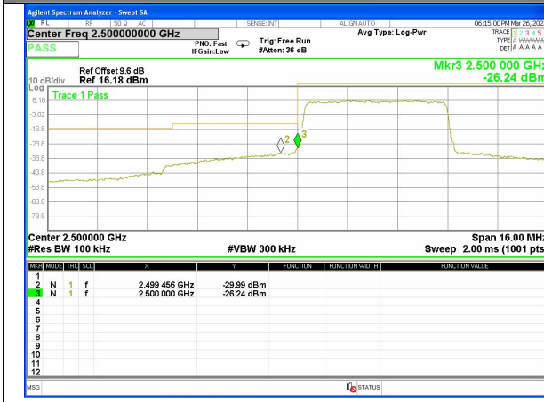
Band 7_5M_QPSK_Low_Full-RB
