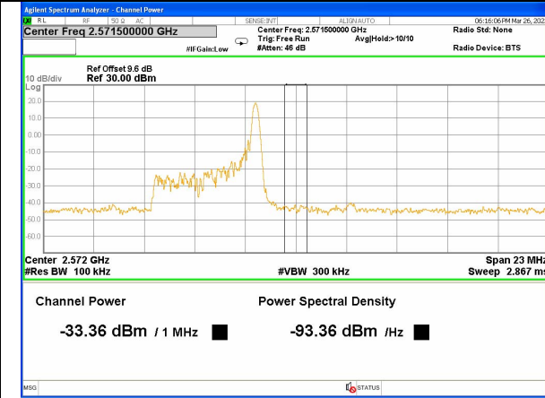
Band 7_5M_QPSK_High_Full-RB
