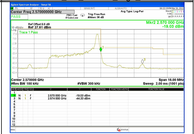
Band 7_5M_16QAM_High_1-RB
