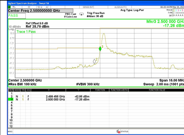
Band 7_5M_16QAM_Low_Full-RB
