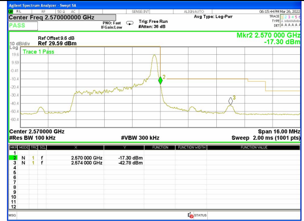
Band 7_5M_QPSK_High_Full-RB
