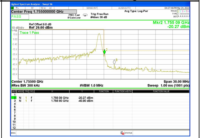
Band 4_15M_16QAM_High_1-RB
