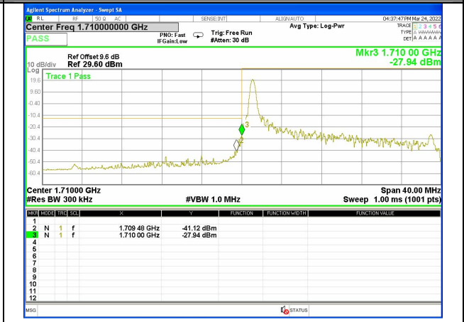
Band 4_20M_16QAM_Low_1-RB
