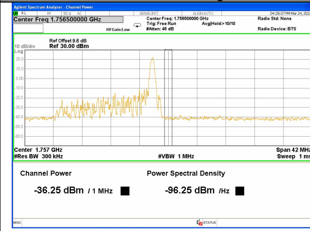
Band 4_15M_16QAM_High_1-RB
