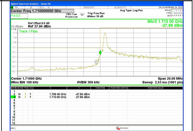
Band 4_10M_16QAM_Low_Full-RB
