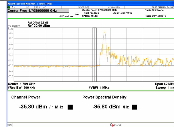
Band 4_20M_QPSK_Low_Full-RB
