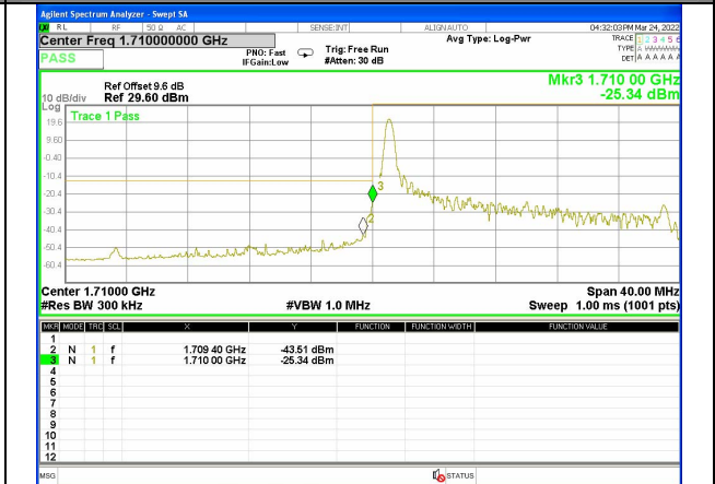
Band 4_20M_QPSK_Low_Full-RB
