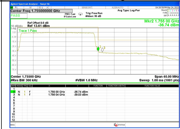
Band 4_20M_16QAM_High_Full-RB
