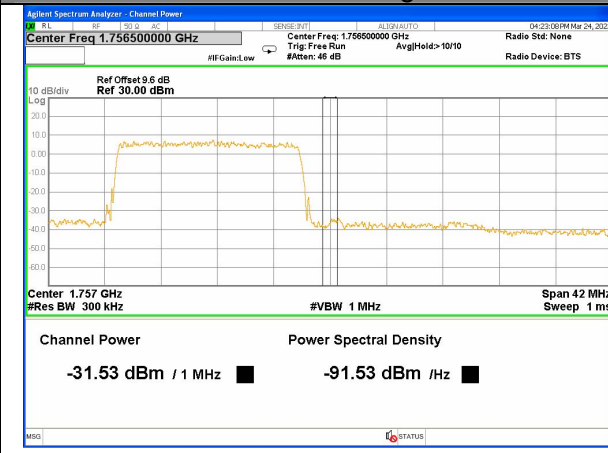
Band 4_15M_QPSK_High_Full-RB
