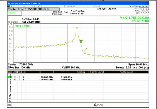
Band 4_10M_QPSK_High_1-RB
