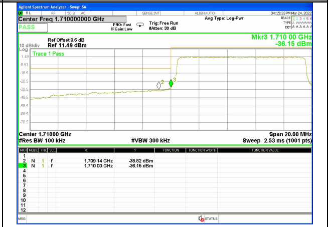
Band 4_10M_16QAM_Low_Full-RB
