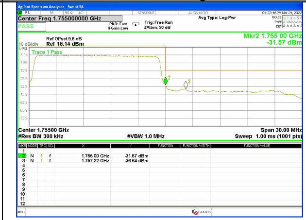
Band 4_15M_QPSK_High_Full-RB
