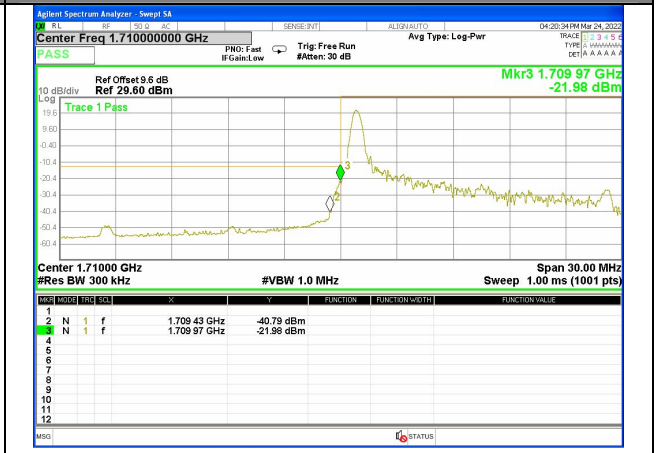
Band 4_15M_QPSK_Low_1-RB
