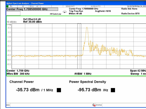
Band 4_15M_QPSK_Low_1-RB
