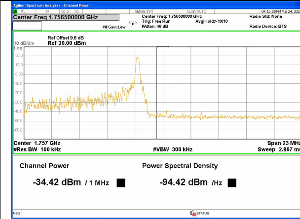
Band 4_10M_16QAM_High_Full-RB
