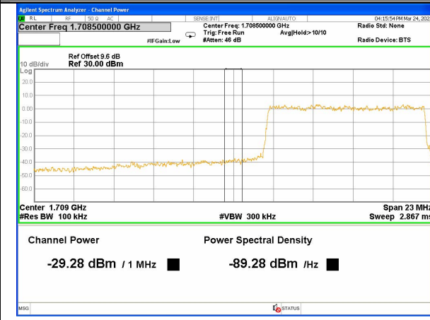
Band 4_10M_16QAM_Low_Full-RB
