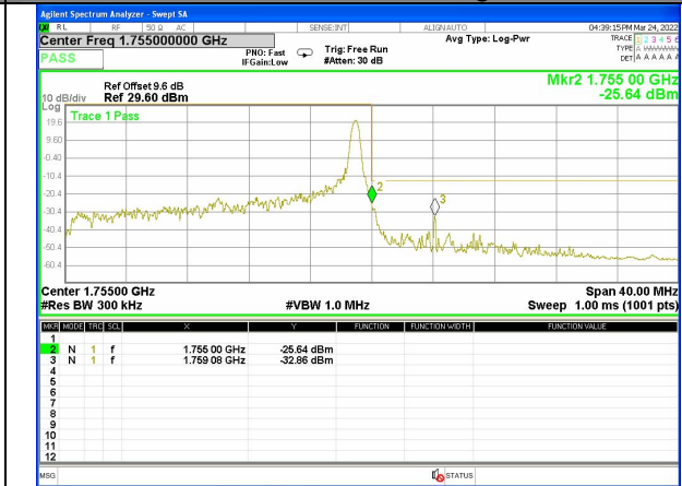
Band 4_20M_16QAM_High_Full-RB
