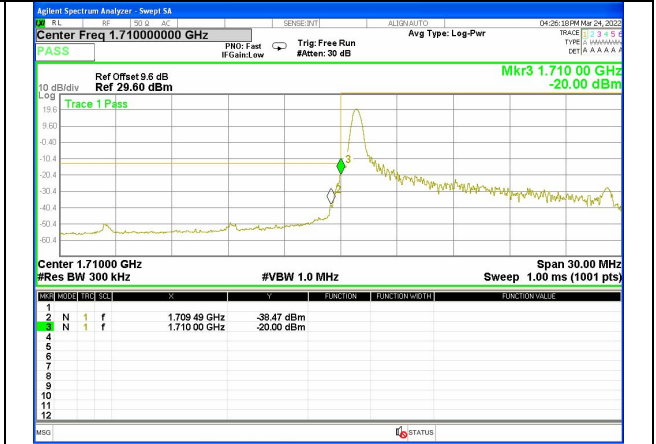
Band 4_15M_16QAM_Low_Full-RB
