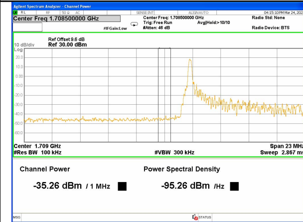
Band 4_10M_16QAM_Low_Full-RB
