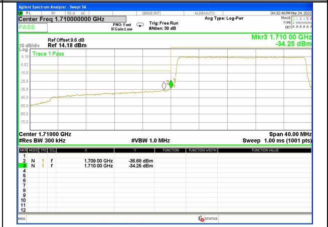
Band 4_20M_QPSK_Low_Full-RB
