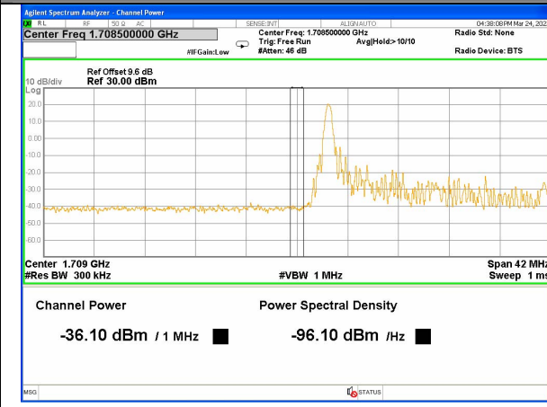
Band 4_20M_16QAM_Low_1-RB
