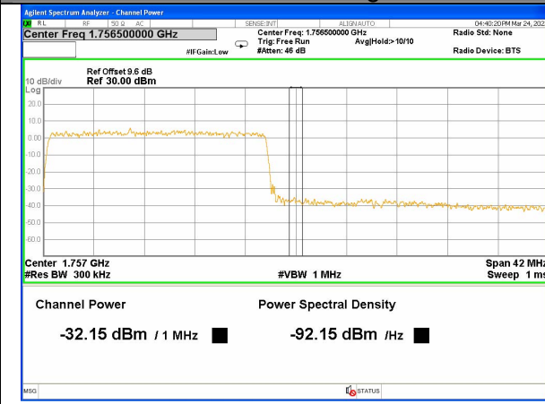
Band 4_20M_16QAM_High_Full-RB
