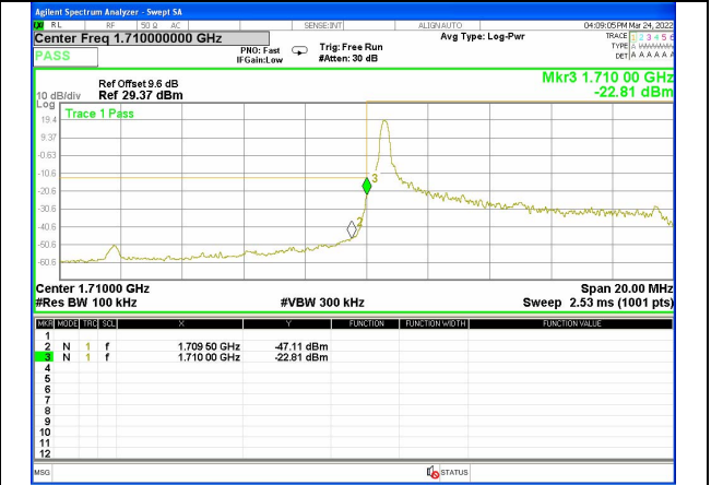
Band 4_10M_QPSK_Low_Full-RB
