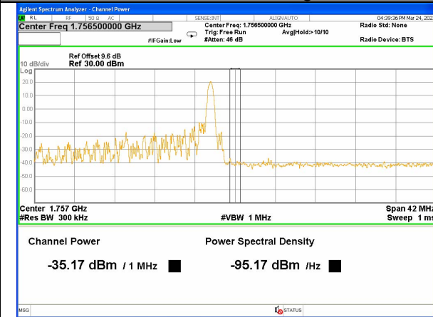
Band 4_20M_16QAM_High_Full-RB
