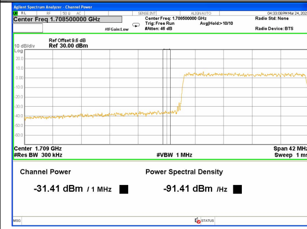
Band 4_20M_QPSK_Low_Full-RB
