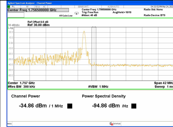
Band 4_20M_QPSK_High_Full-RB
