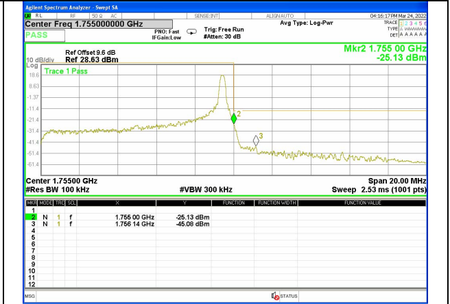
Band 4_10M_16QAM_High_Full-RB
