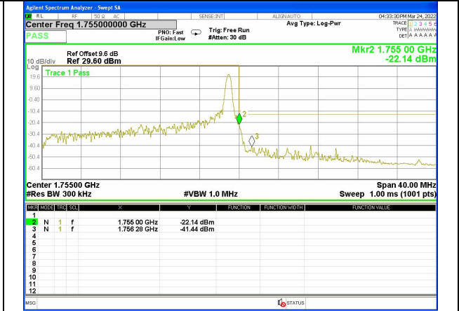
Band 4_20M_QPSK_High_Full-RB
