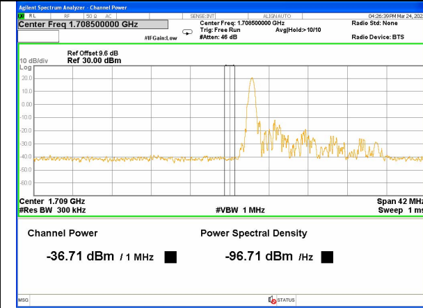
Band 4_15M_16QAM_Low_Full-RB
