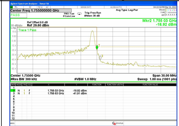
Band 4_15M_QPSK_High_Full-RB
