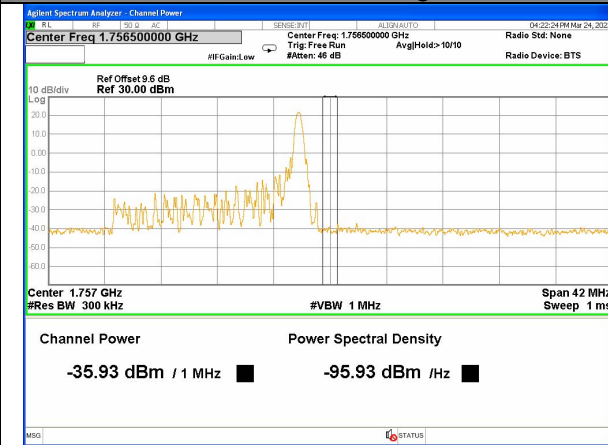
Band 4_15M_QPSK_High_Full-RB
