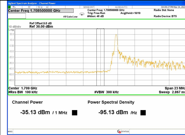
Band 4_10M_QPSK_Low_Full-RB
