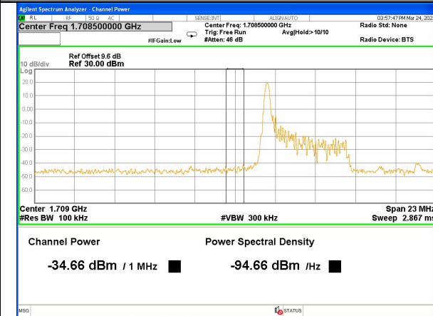
Band 4_5M_QPSK_Low_Full-RB
