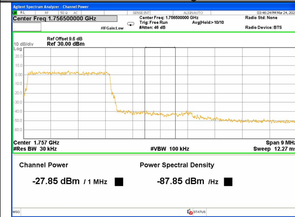
Band 4_3M_QPSK_High_Full-RB
