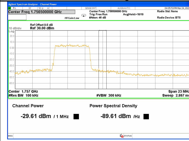
Band 4_5M_16QAM_High_Full-RB
