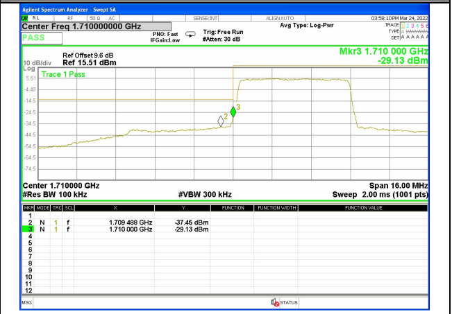
Band 4_5M_QPSK_Low_Full-RB
