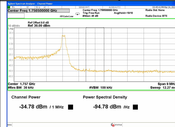
Band 4_3M_QPSK_High_Full-RB
