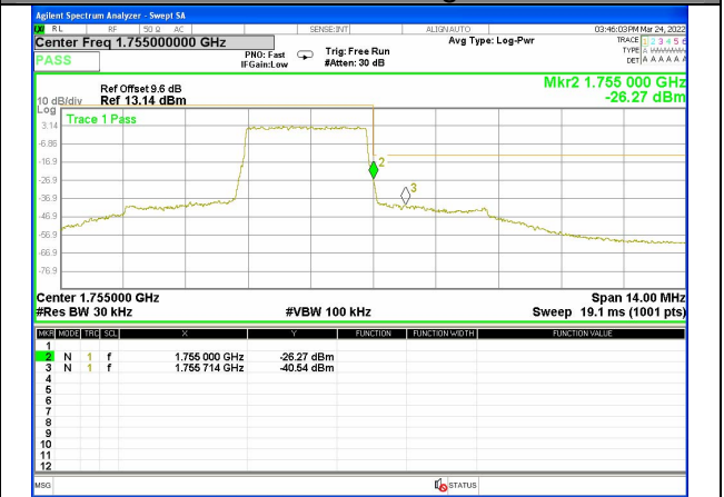
Band 4_3M_QPSK_High_Full-RB
