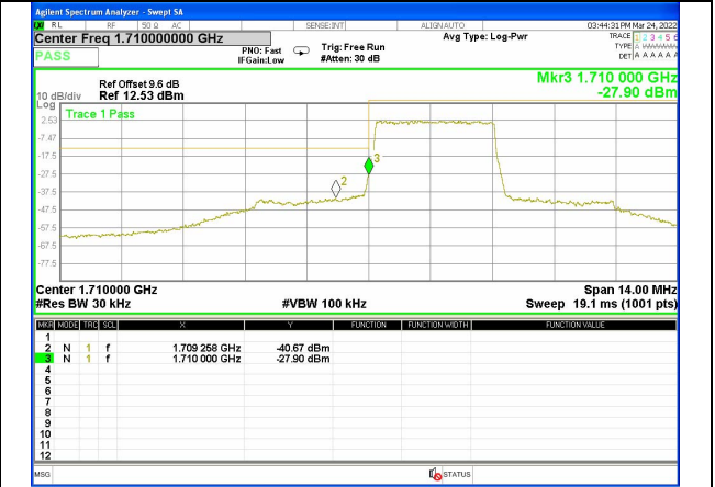
Band 4_3M_QPSK_High_1-RB
