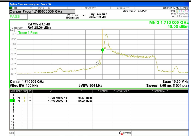
Band 4_5M_16QAM_Low_1-RB
