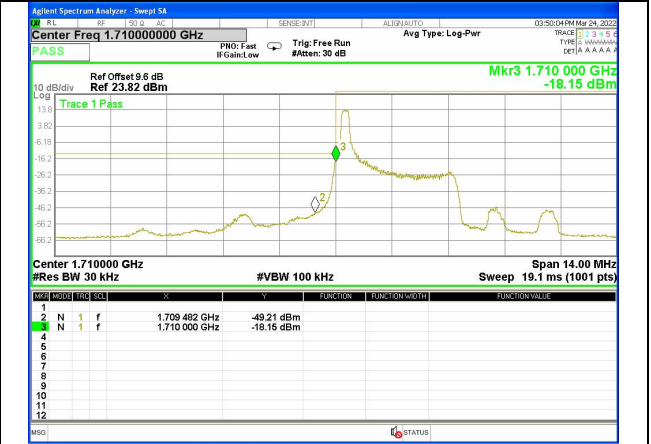
Band 4_3M_16QAM_Low_Full-RB
