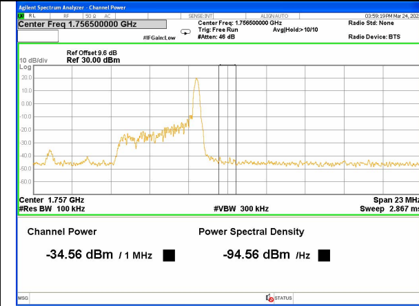
Band 4_5M_QPSK_High_Full-RB
