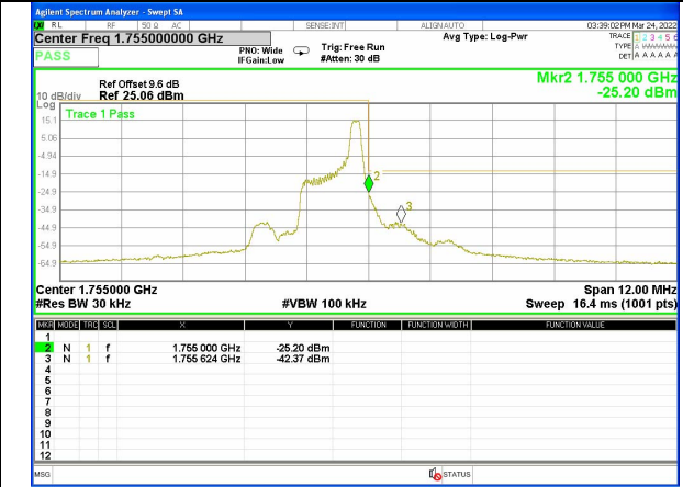
Band 4_1.4M_16QAM_High_Full-RB
