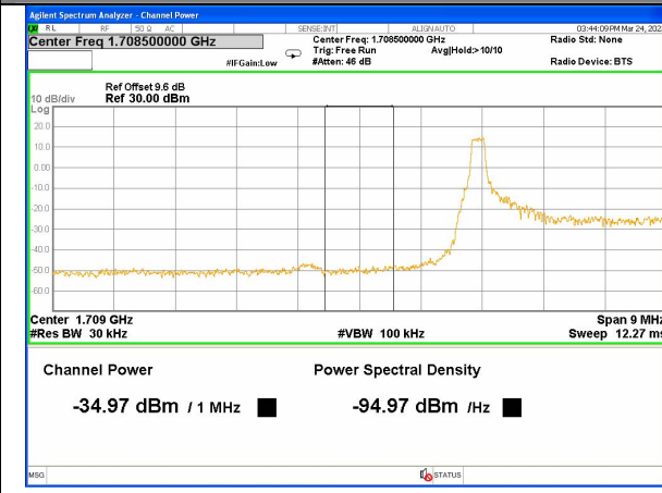
Band 4_3M_QPSK_Low_1-RB
