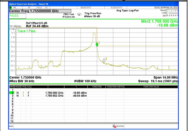
Band 4_3M_16QAM_High_1-RB
