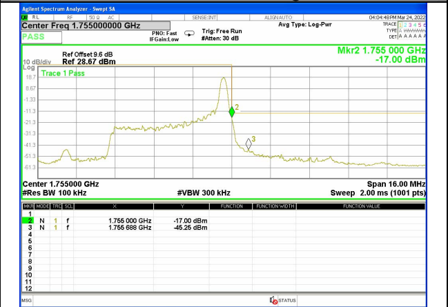
Band 4_5M_16QAM_High_Full-RB
