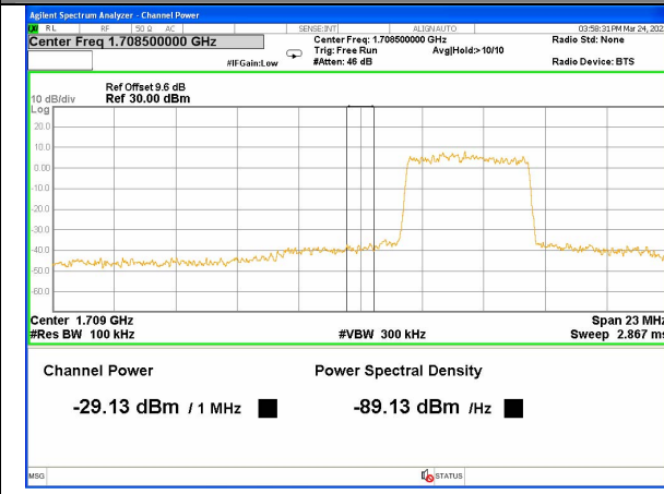
Band 4_5M_QPSK_Low_Full-RB
