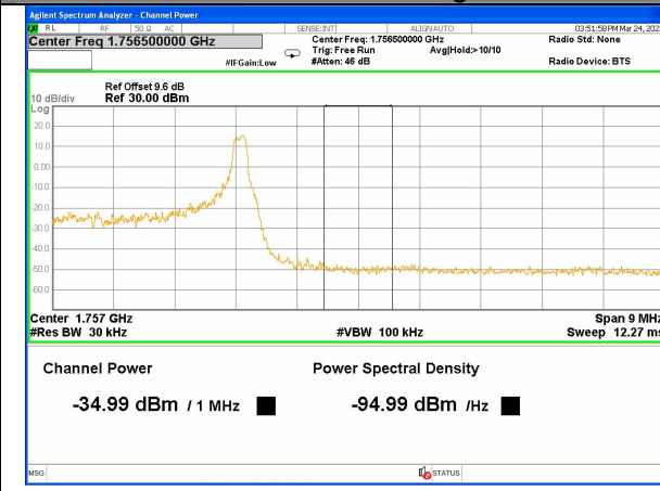
Band 4_3M_16QAM_High_1-RB
