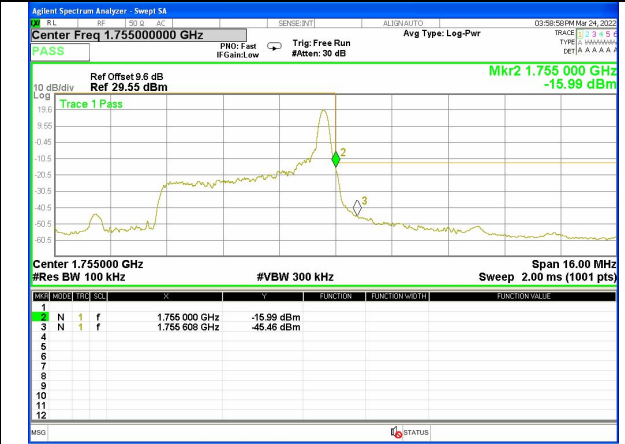
Band 4_5M_QPSK_High_Full-RB
