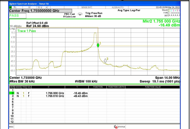
Band 4_3M_QPSK_High_Full-RB
