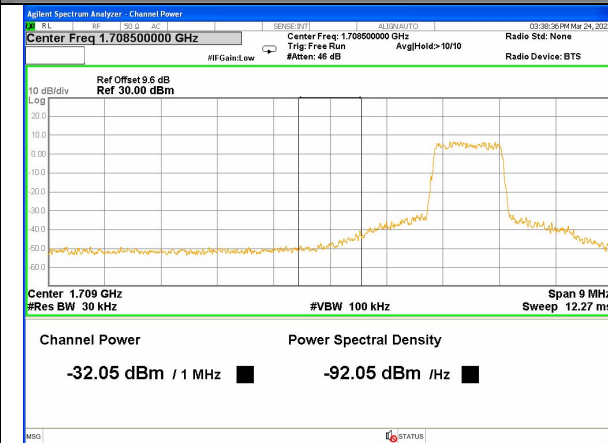
Band 4_1.4M_16QAM_Low_Full-RB
