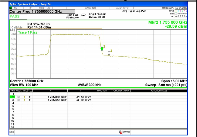
Band 4_5M_16QAM_High_Full-RB
