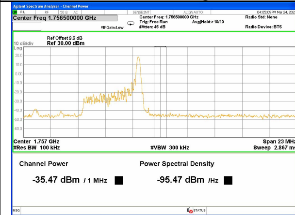
Band 4_5M_16QAM_High_Full-RB
