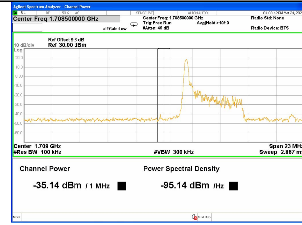
Band 4_5M_16QAM_Low_1-RB
