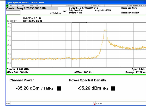
Band 4_3M_16QAM_Low_Full-RB
