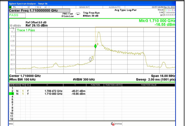
Band 4_5M_QPSK_Low_Full-RB
