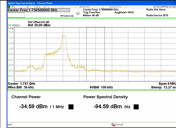
Band 4_1.4M_16QAM_High_Full-RB
