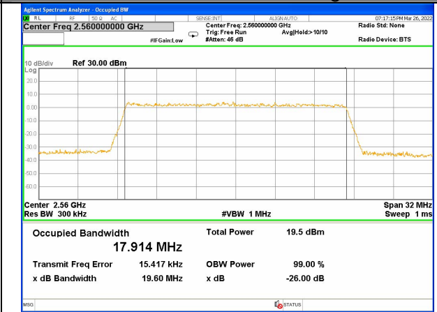
Band 7_20M_16QAM_High
