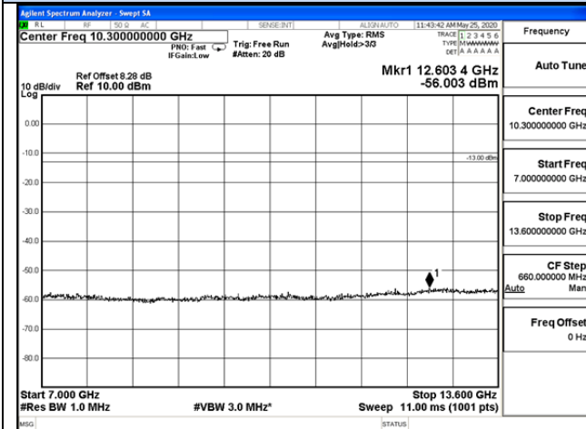
7 GHz – 13.6 GHz
