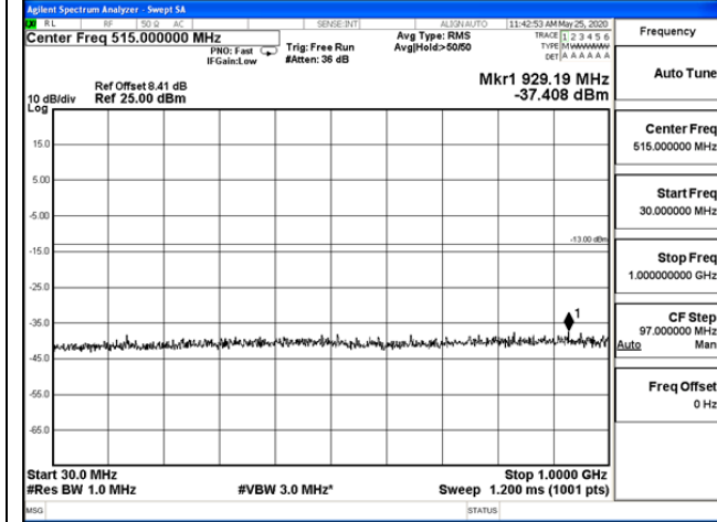
30 MHz – 1000 MHz
