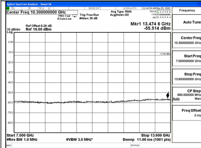
7 GHz – 13.6 GHz
