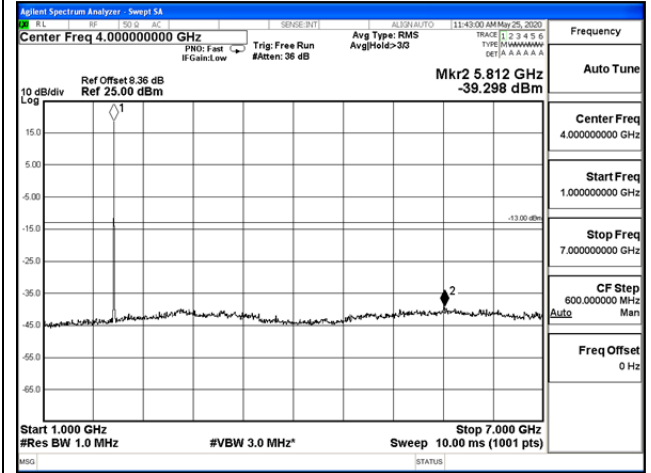
1 GHz – 7 GHz
