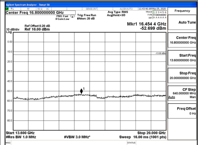
13.6 GHz – 20 GHz
