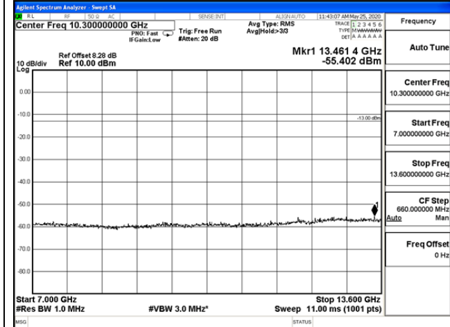
7 GHz – 13.6 GHz
