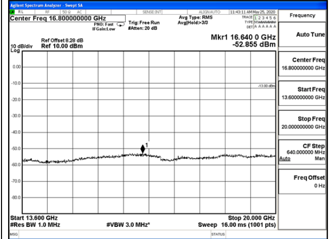
13.6 GHz – 20 GHz
