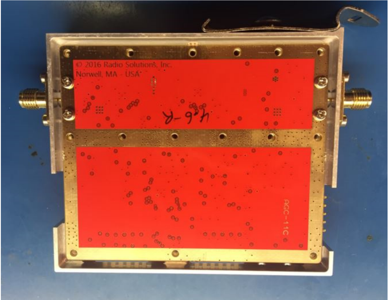
AGC Amplifier Back Side Inside the Enclosure*
