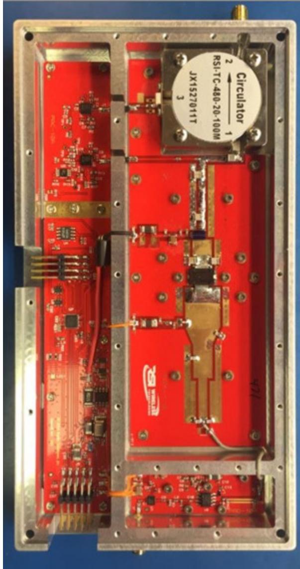
Power Amplifier Module with PA Controller and PA Driver
