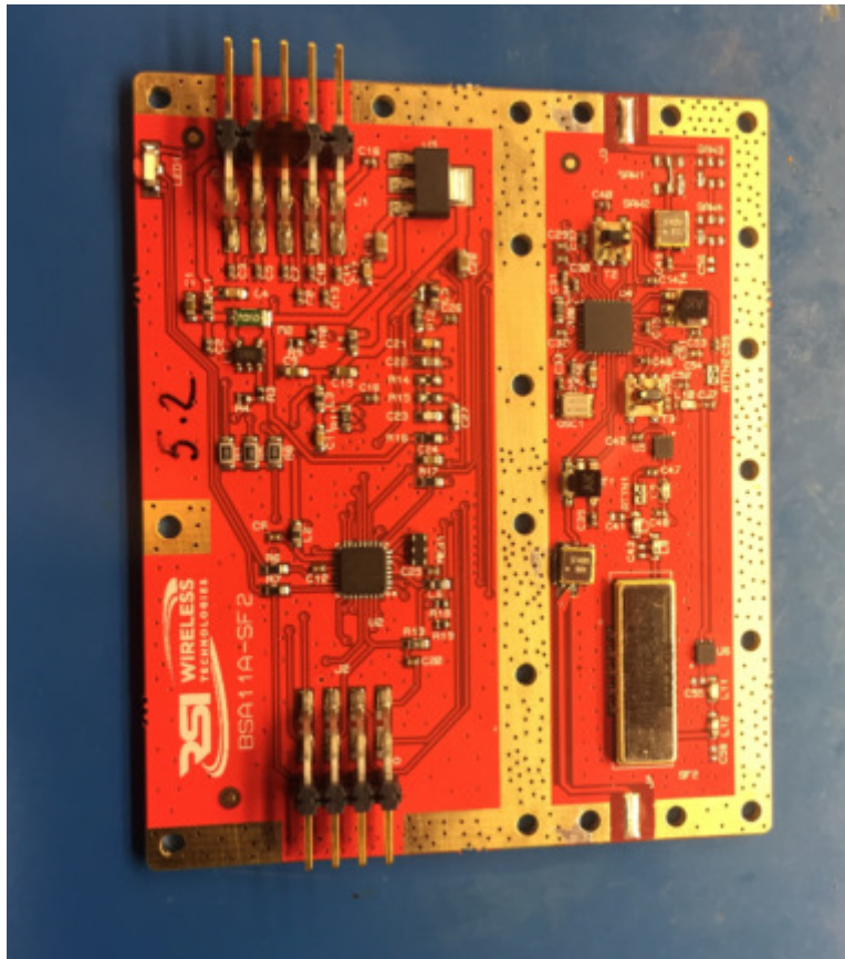
Channel Module Component Side
