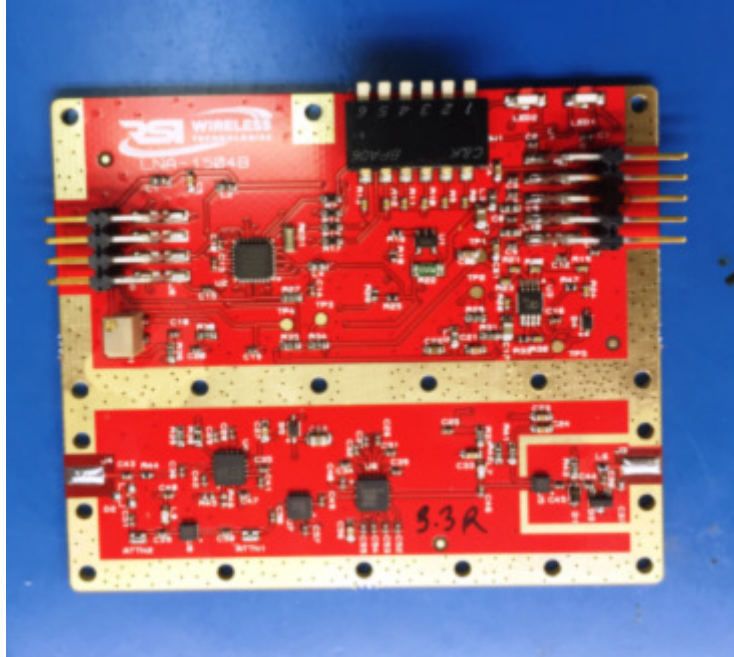
LNA Amplifier Component Side
