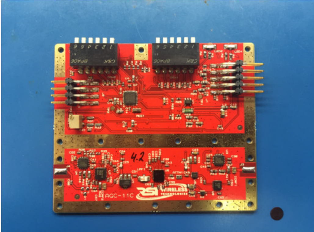
AGC Amplifier Component Side
