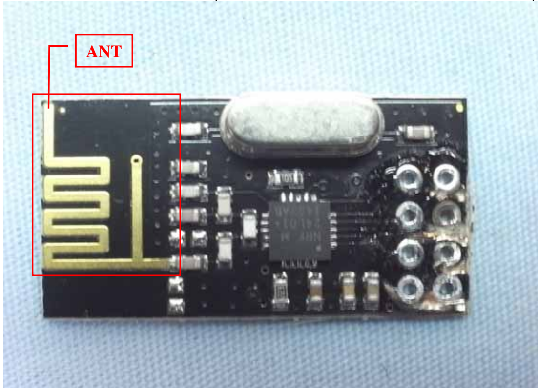
Figure 11 Internal View (Transmitter RF Module Board, Front View)
