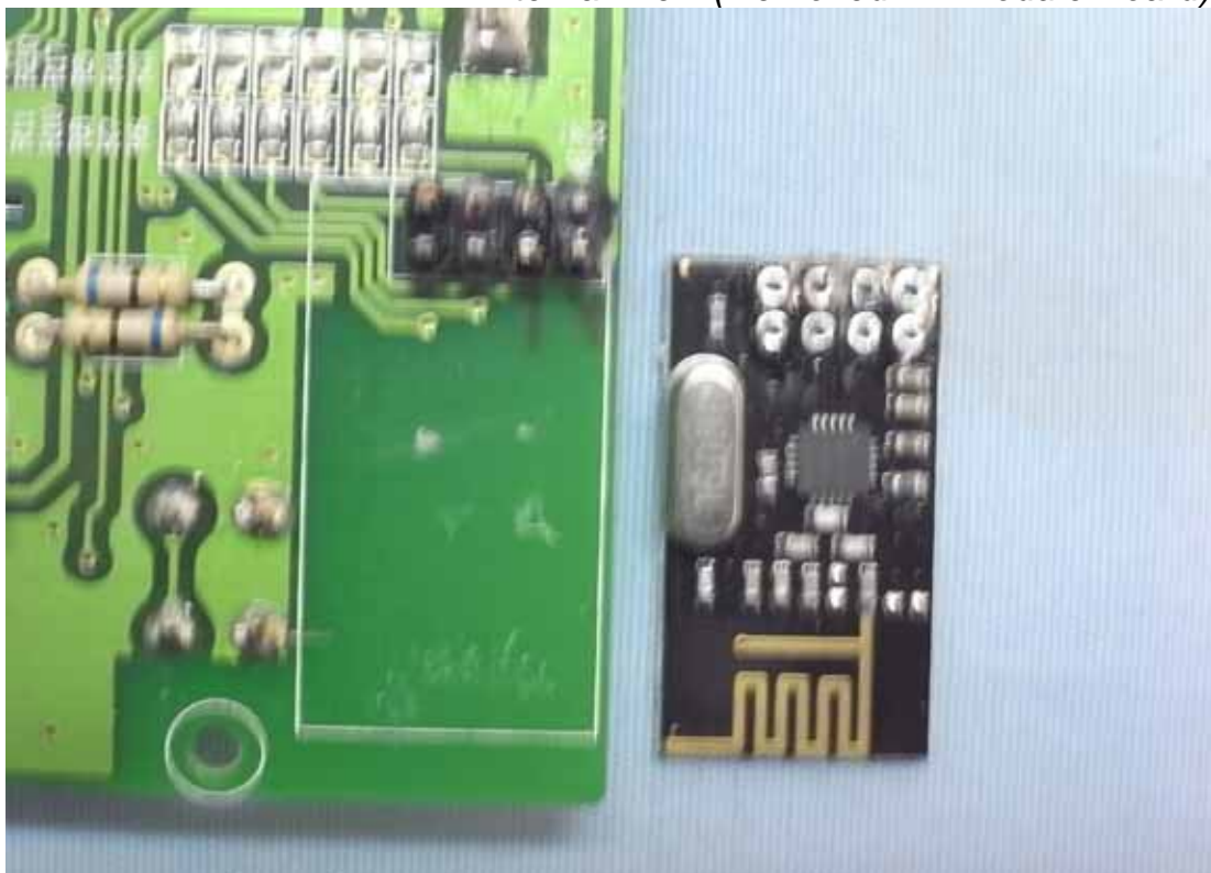
Figure 10 Internal View (Removed RF Module Board)
