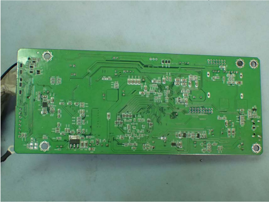
Figure 57 Model: WB001, Internal View (Tuner Board, Back View)
