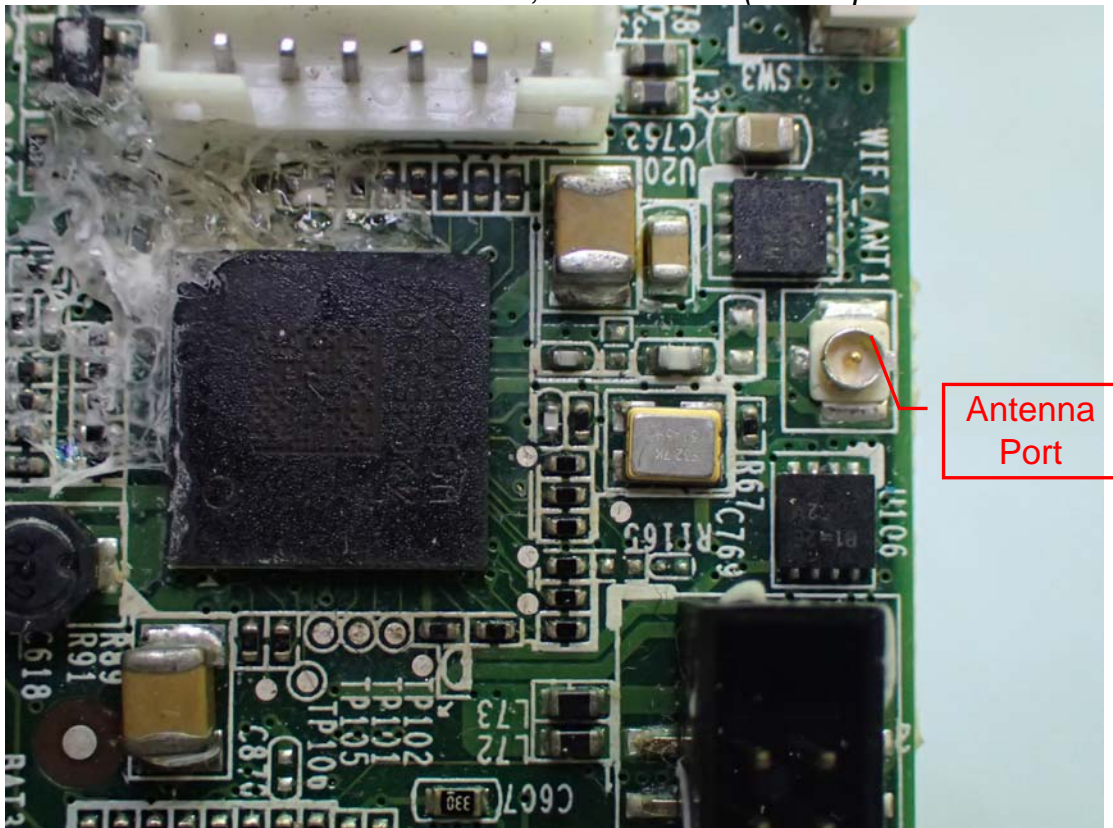
Model: WT002, Internal View (RF Chip and Antenna Port View)
