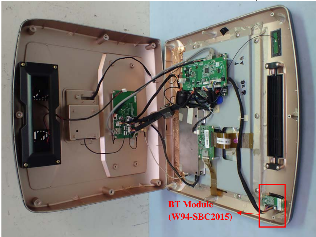
Model: WT002, Internal View (Removed Back Cover)
