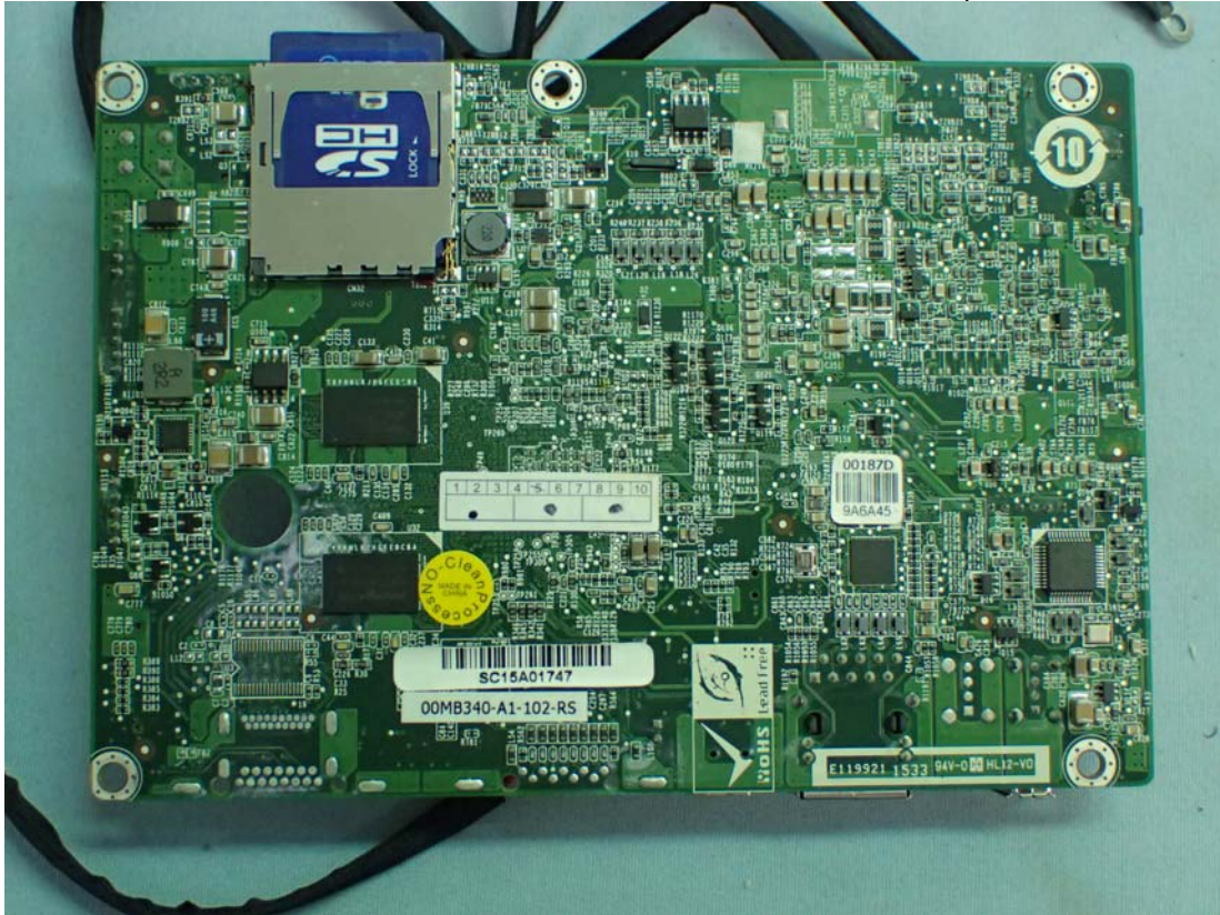
Model: WT002, Internal View (Main Board, Back View)
