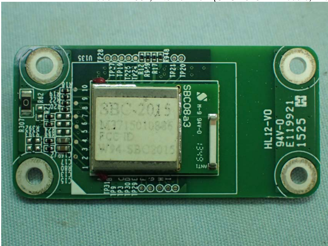
Model: WT002, Internal View (SBC-2015 BT Module, Front View)
