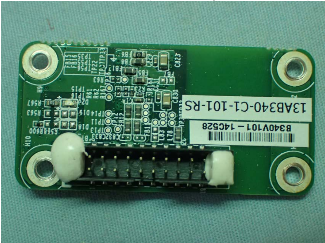
Figure 48 Model: WB001, Internal View (SBC-2015 BT Module, Back View)
