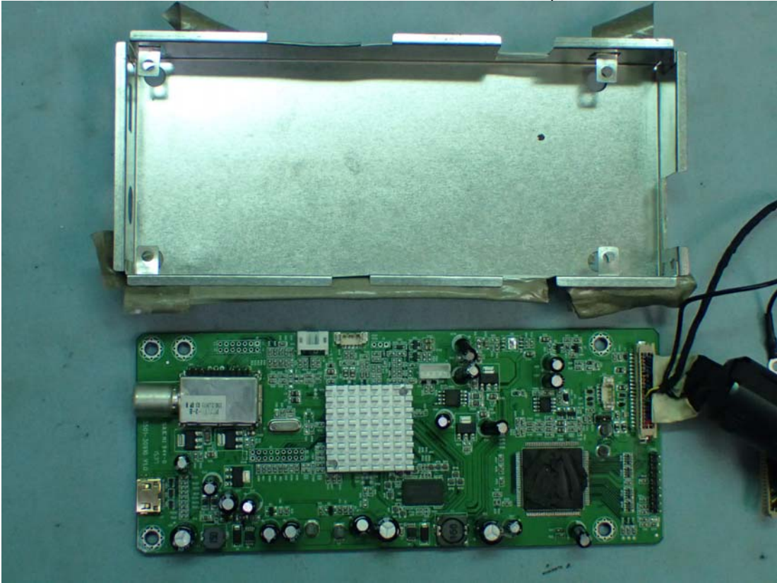
Model: WT002, Internal View (Removed Tuner Board Cover)
