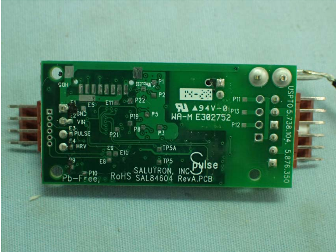
Model: WB001, Internal View (Internal Board, Back View)
