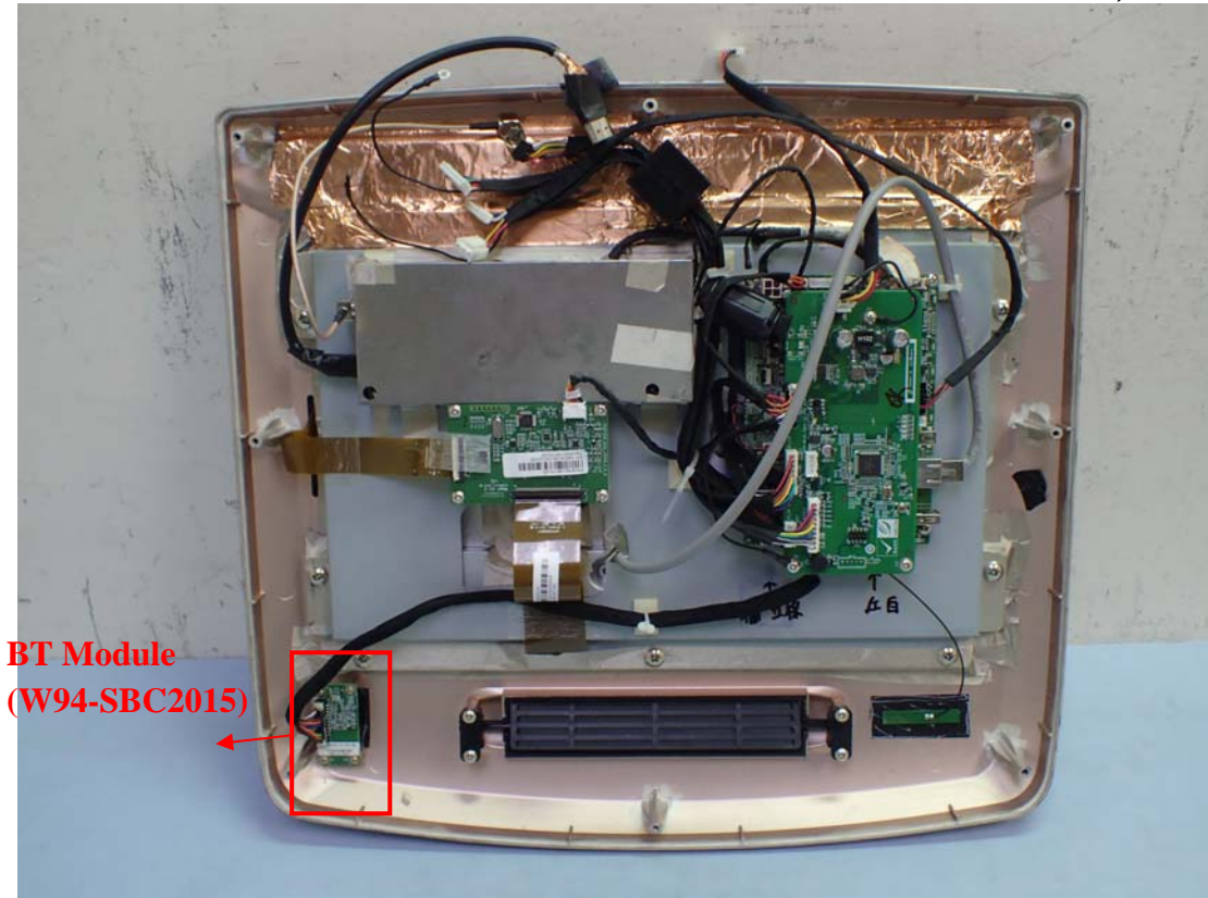
Figure 15 Model: WT002, Internal View
