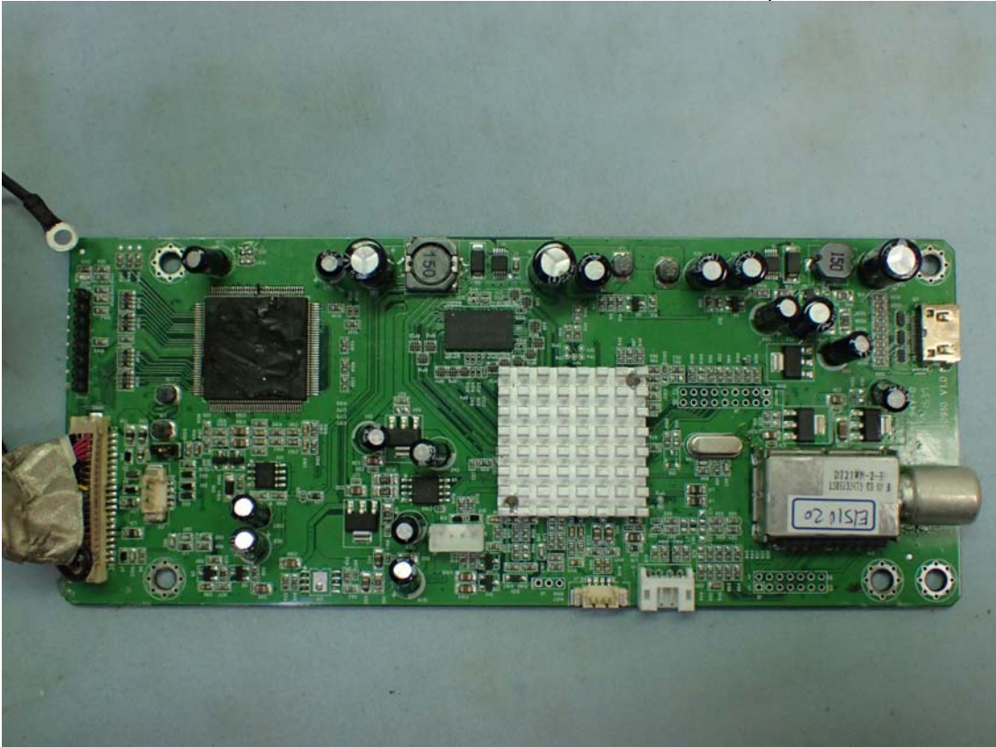
Model: WB001, Internal View (Tuner Board, Front View)
