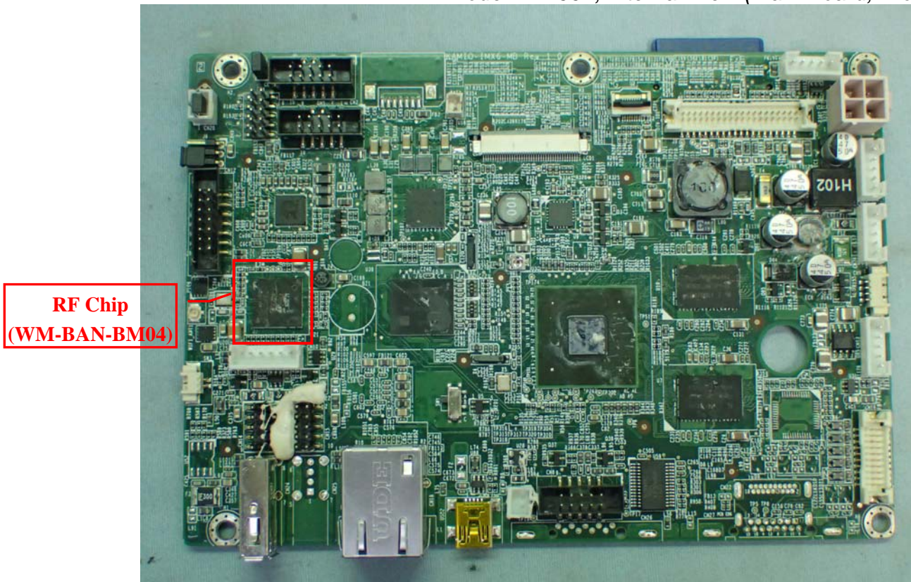
Model: WB001, Internal View (Main Board, Front View)
