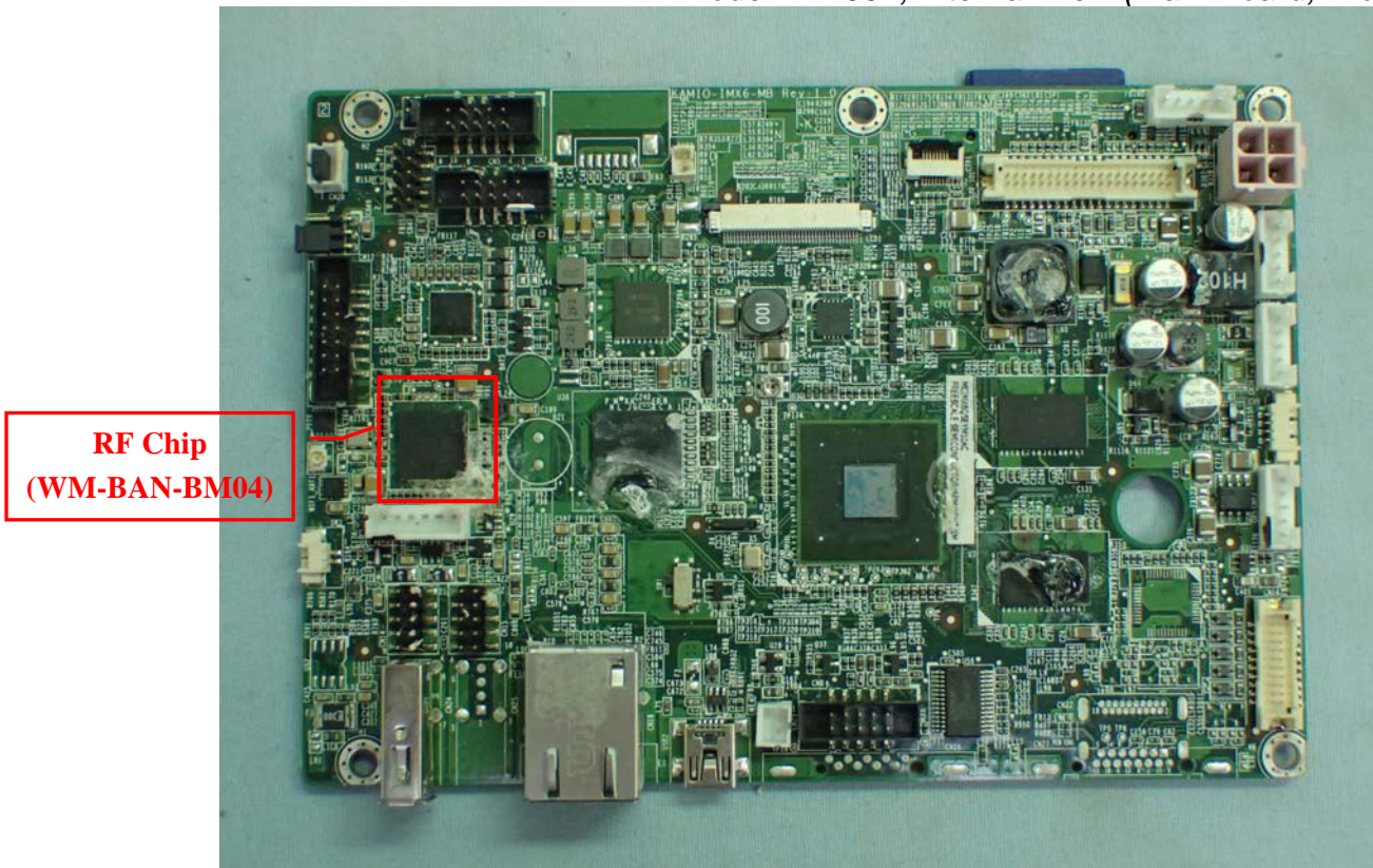
Model: WT002, Internal View (Main Board, Front View)
