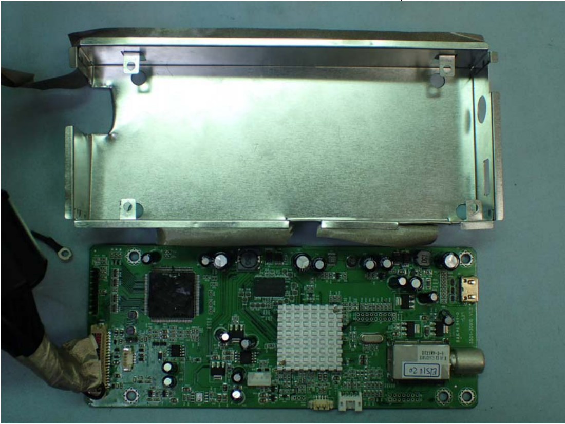
Model: WB001, Internal View (Removed Tuner Board Cover)
