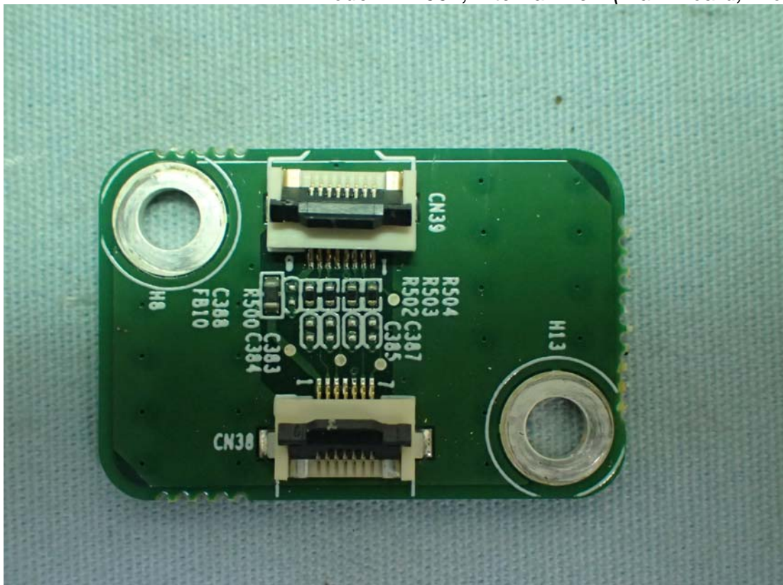
Model: WB001, Internal View (Main Board, Front View)
