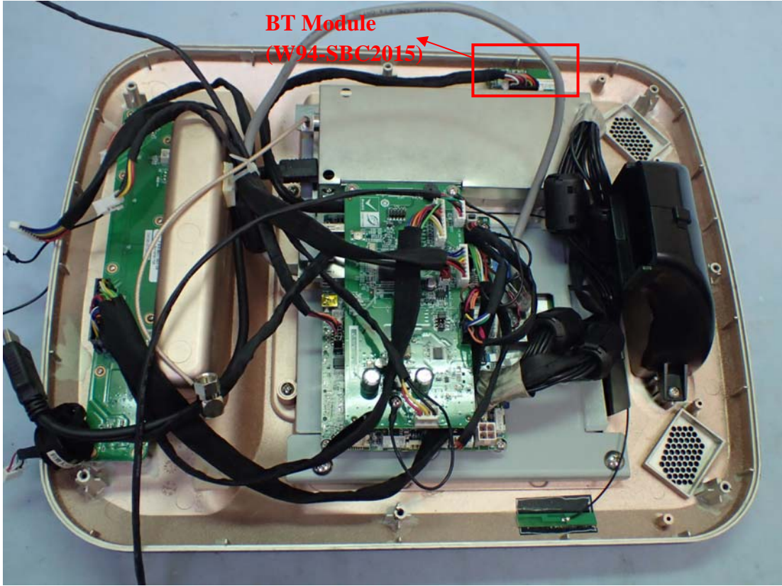
Figure 41 Model: WB001, Internal View
