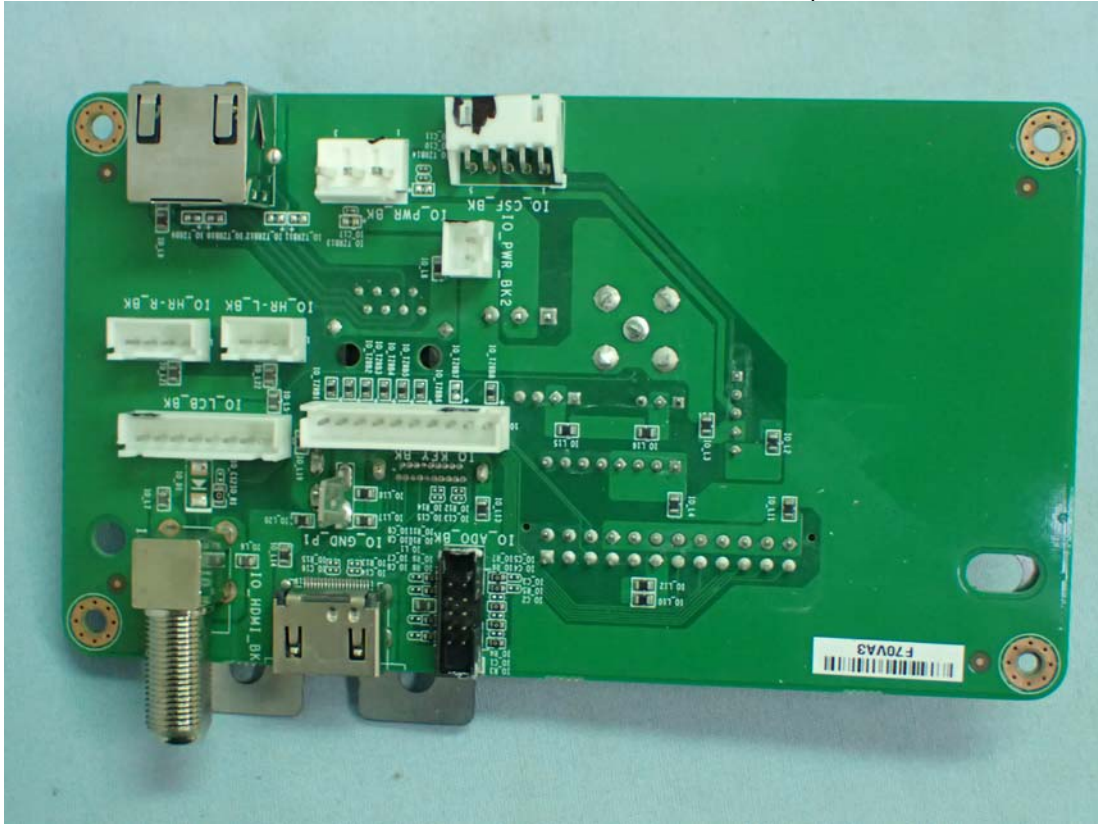
Figure 11 Model: WT002, Internal View (I/O Ports Board, Back View)
