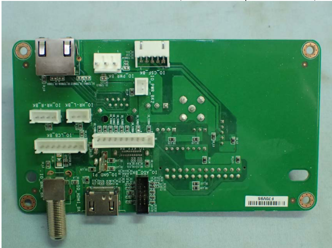
Model: WB001, Internal View (I/O Ports Board, Back View)
