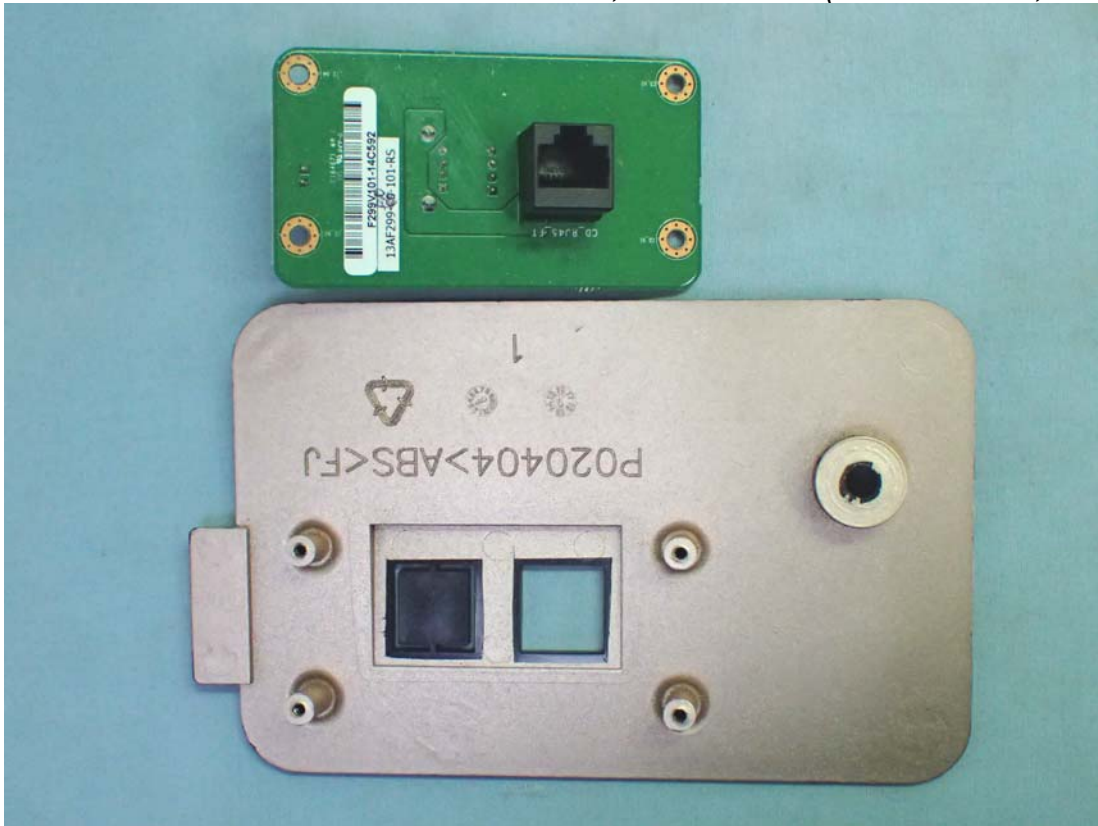
Model: WT002, Internal View (Internal Board, Front View)
