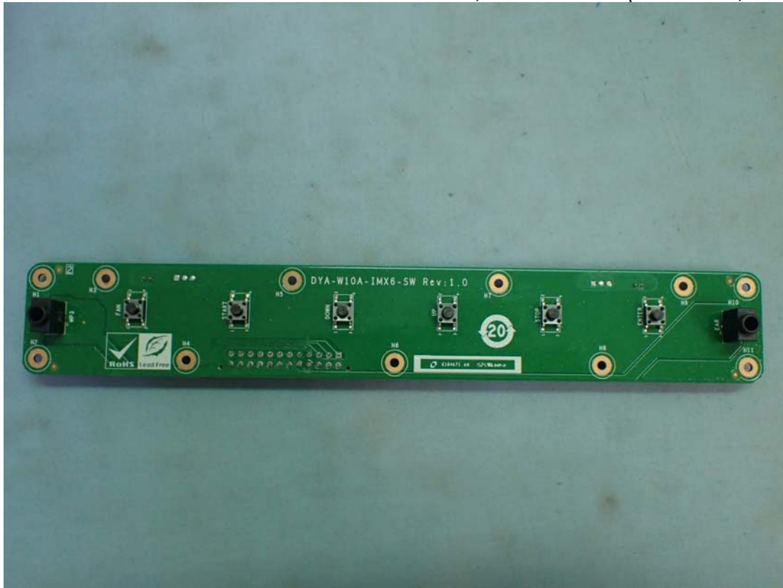
Model: WB001, Internal View (SW Board, Front View)
