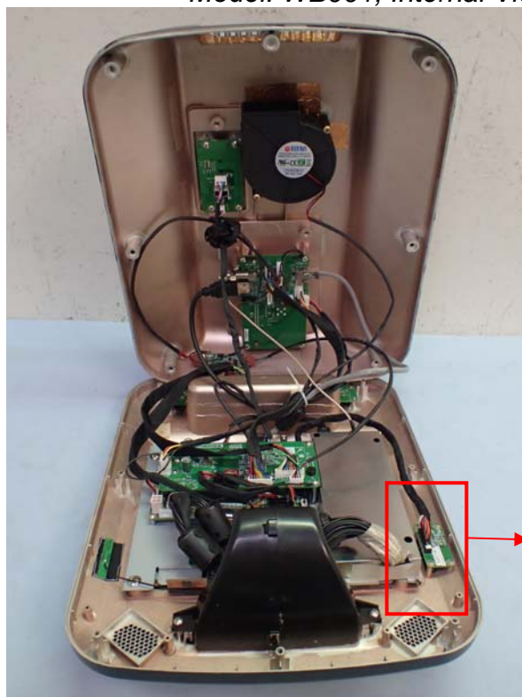
Model: WB001, Internal View (Removed Back Cover)
