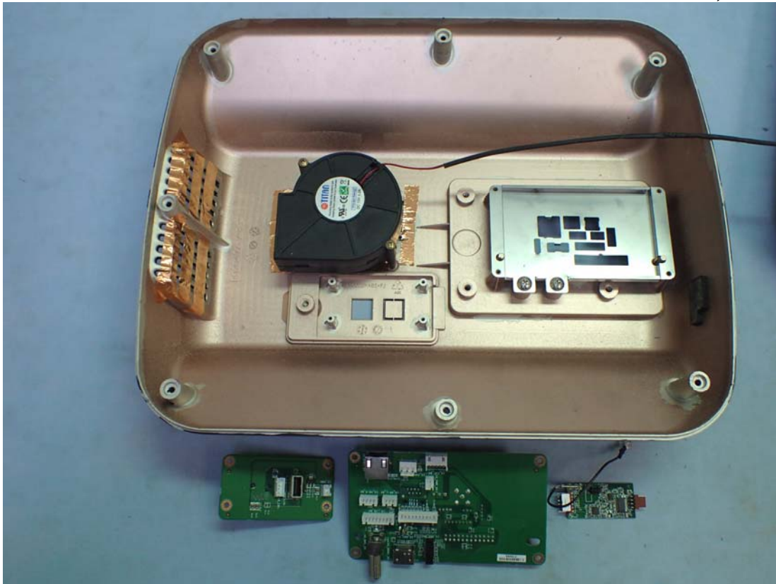
Figure 33 Model: WB001, Internal View
