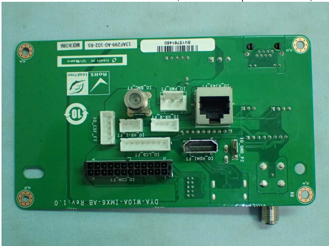
Model: WT002, Internal View (I/O Ports Board, Front View)
