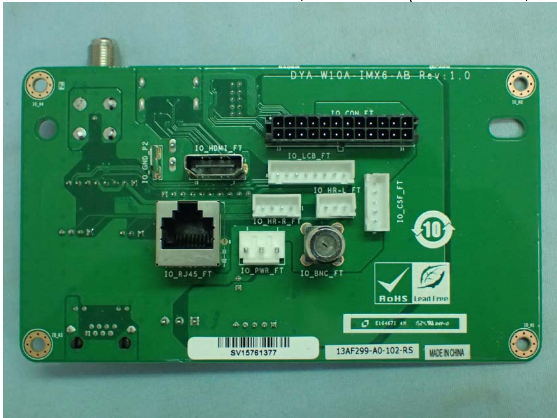
Model: WB001, Internal View (I/O Ports Board, Front View)
