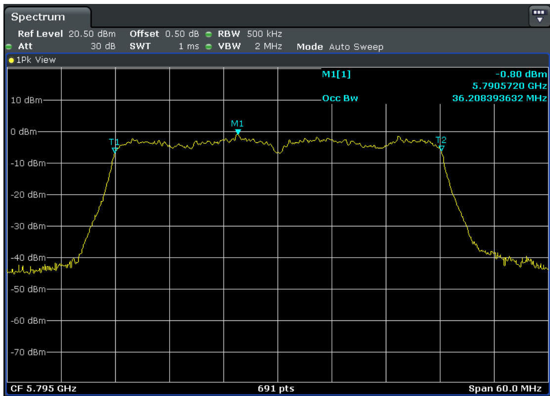
5795MHz-Ant2
