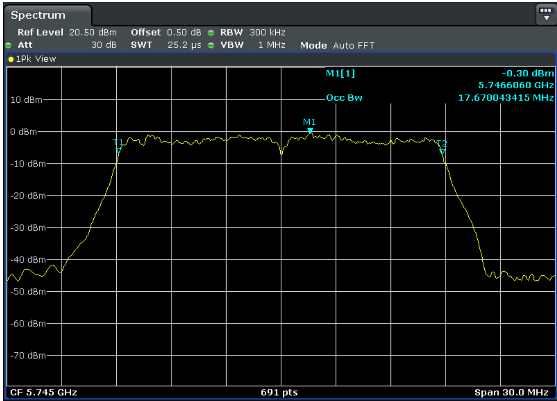
5745MHz-Ant2
