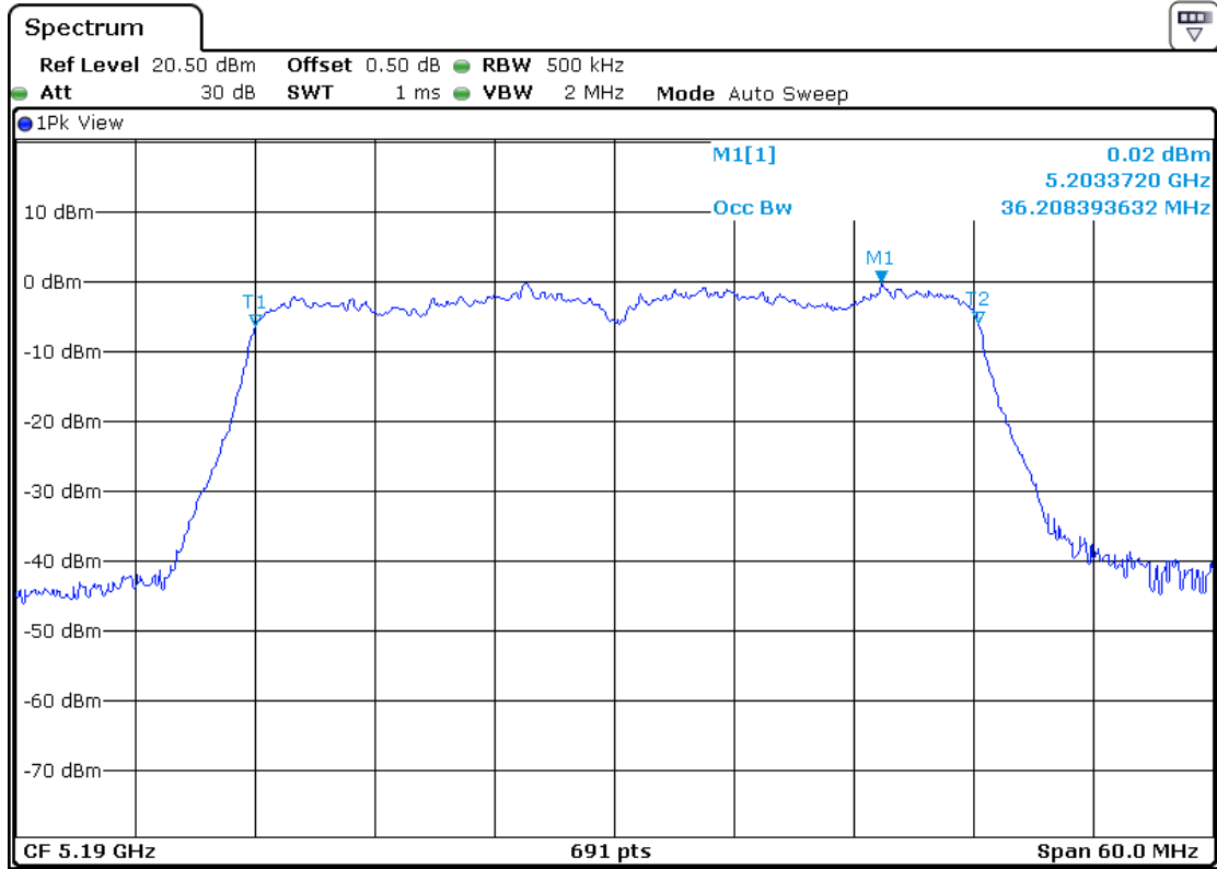
5190MHz-Ant2
