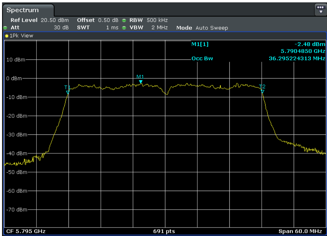
5795MHz-Ant2
