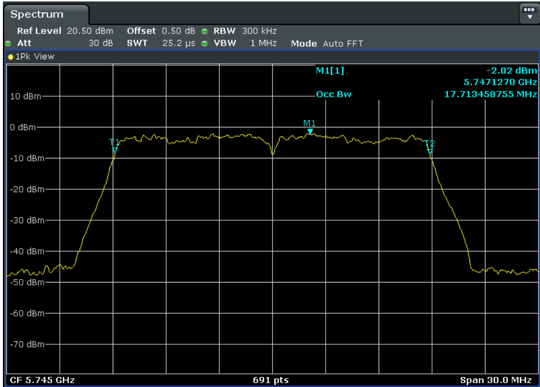
5745MHz-Ant2
