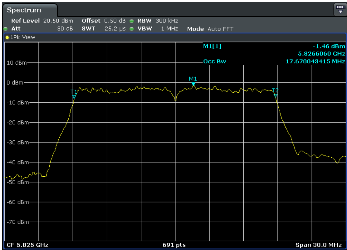
5825MHz-Ant2
