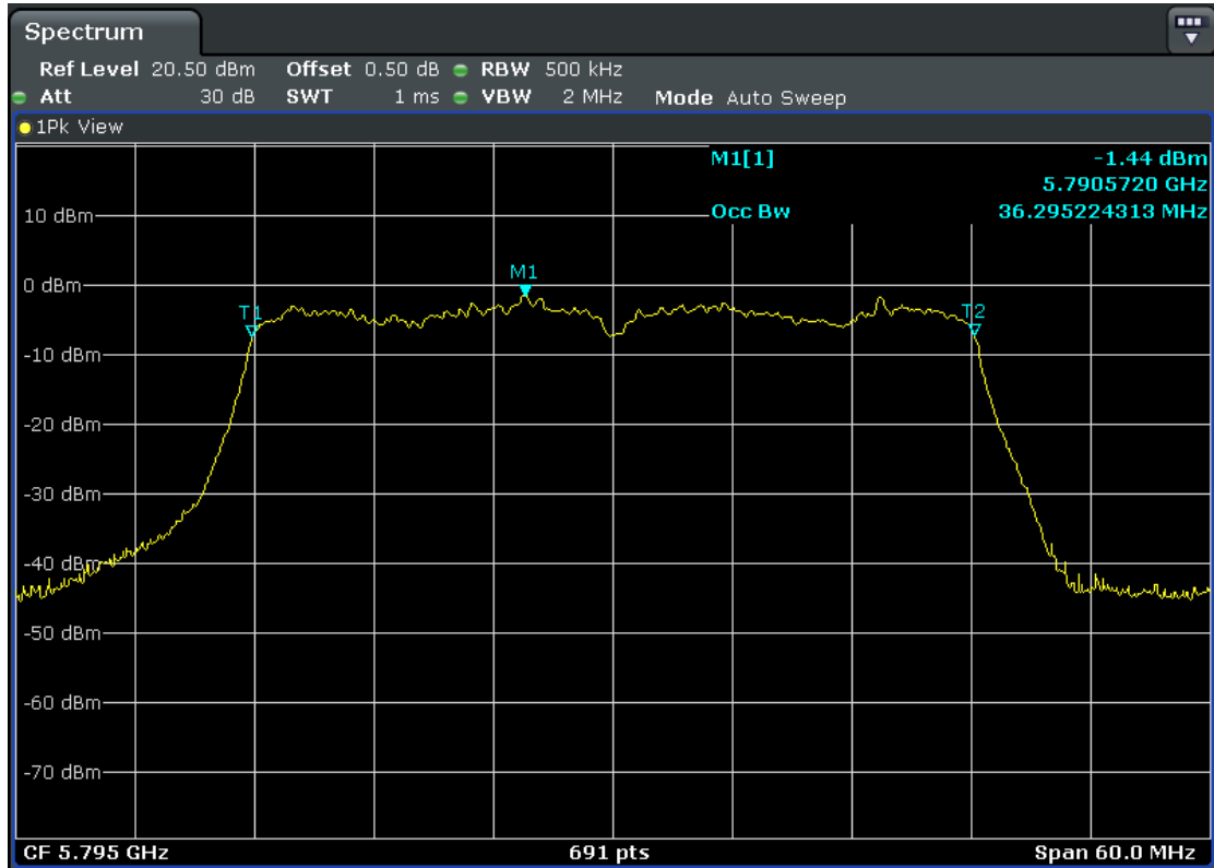
5795MHz-Ant2
