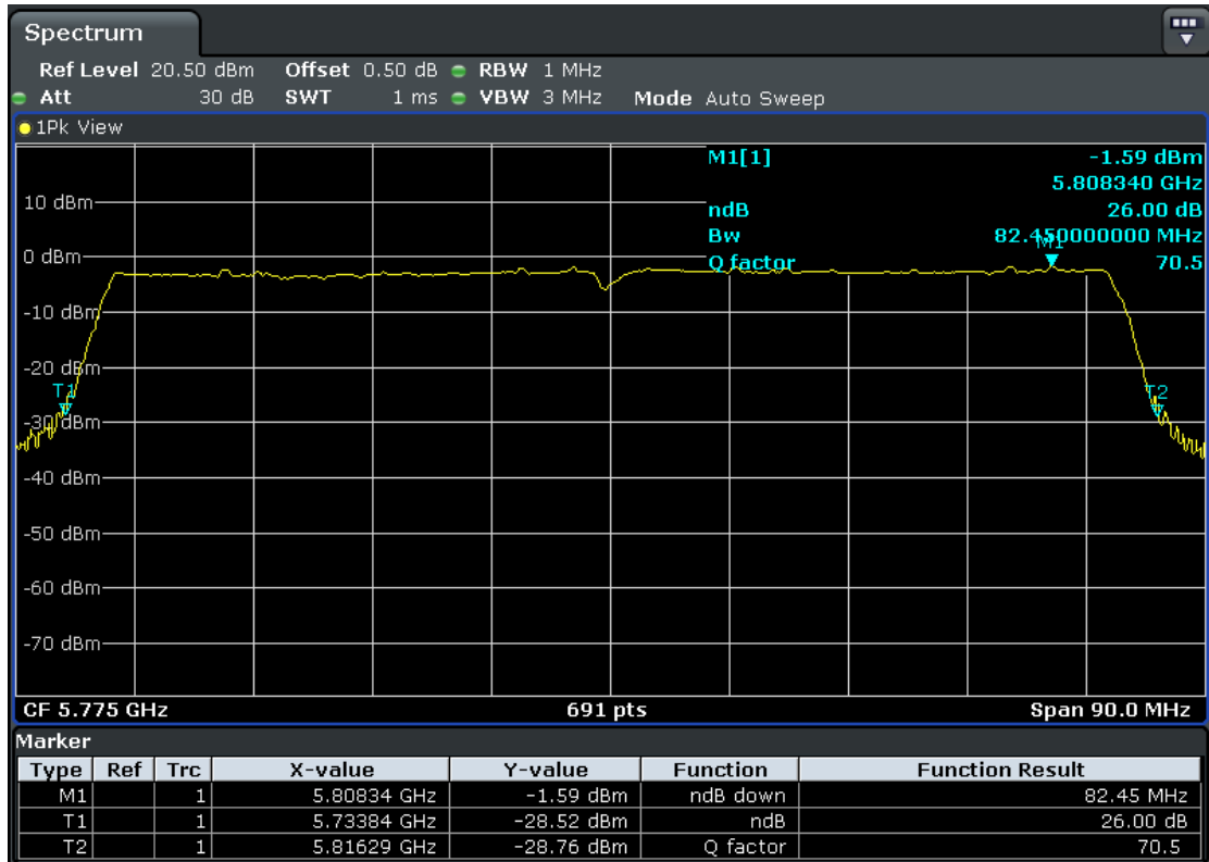
5775MHz-Ant2
