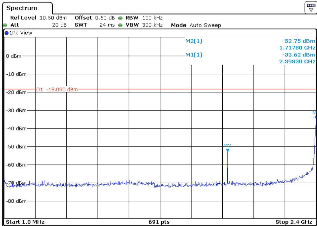
ANT4 Channel 01 (2412MHz) Reference Level: 1.91dBm
