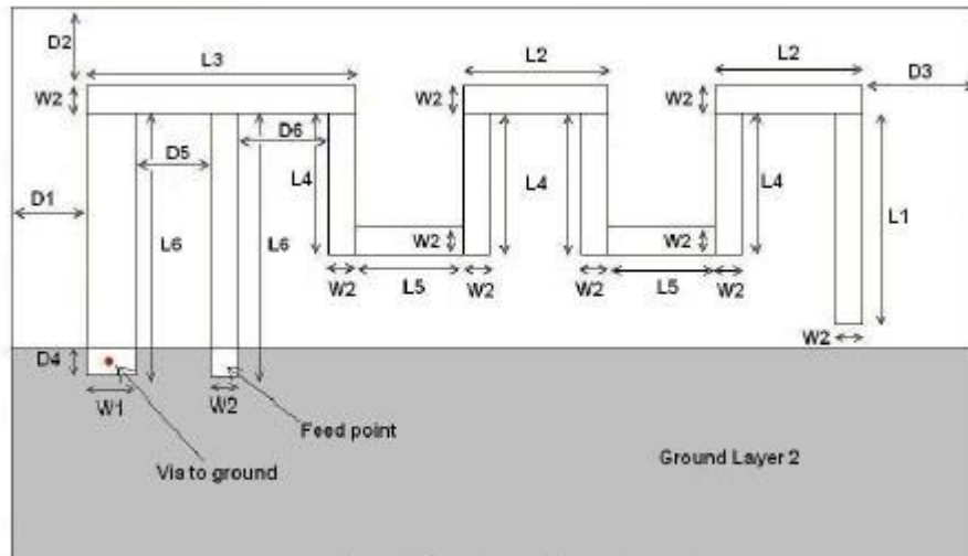
Figure 3: Antenna Dimensions
