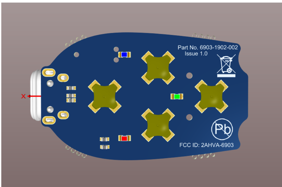
Figure 2 FCC ID on Silkscreen of PCB bottom side
