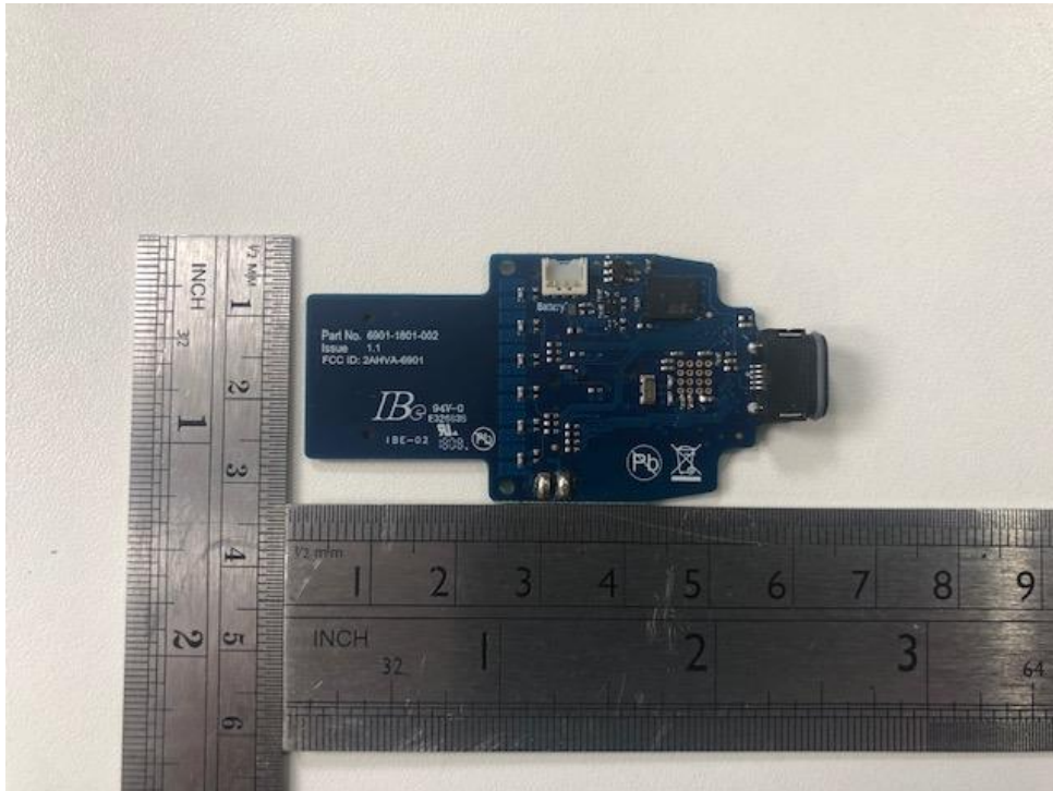
Figure 1 PCB Top View
