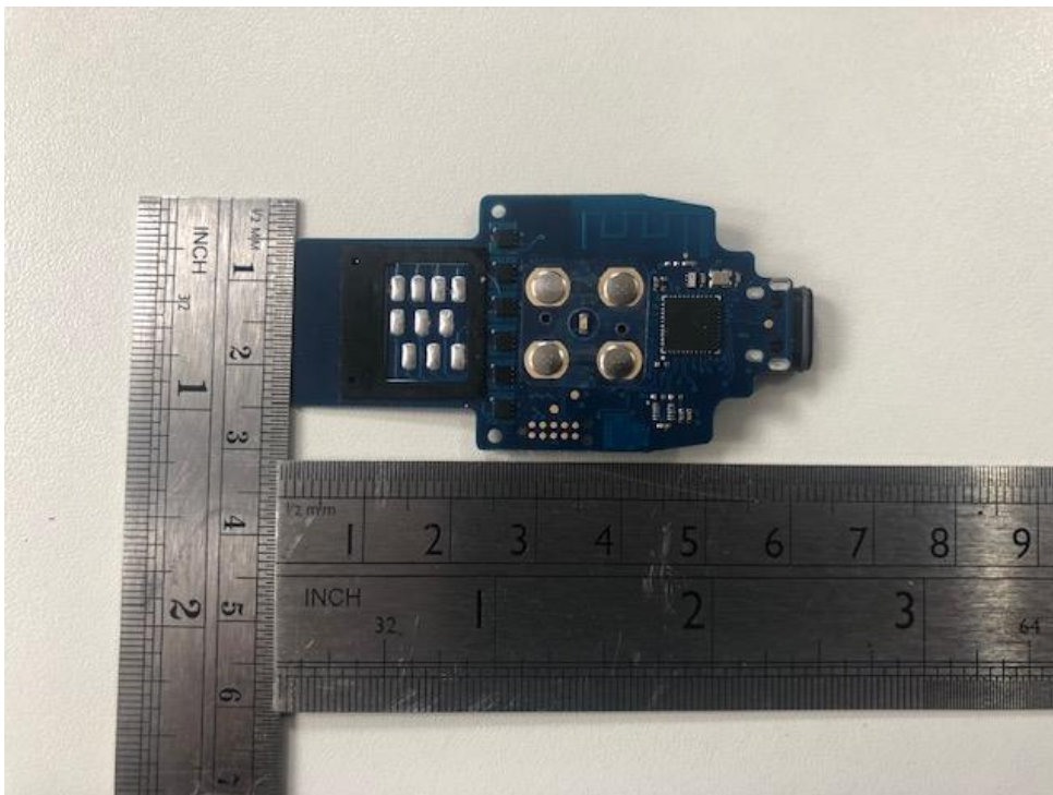
Figure 2 PCB Bottom View
