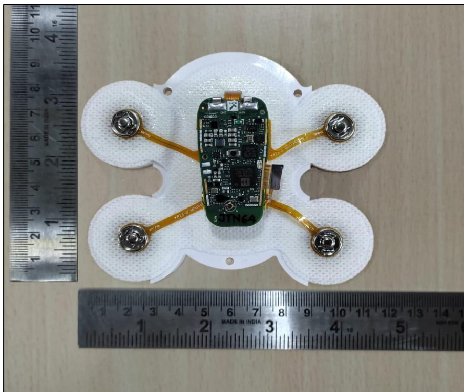
RF module shield open
