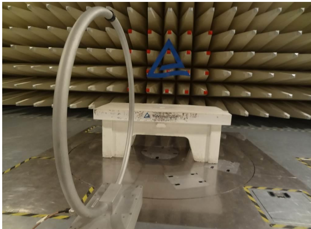
Test Setup
