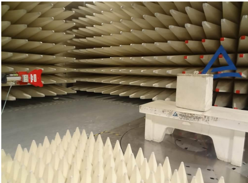
Test Setup
