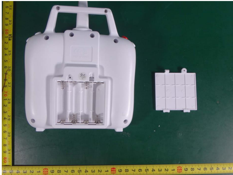
EUT Photo #1 Uncover View
