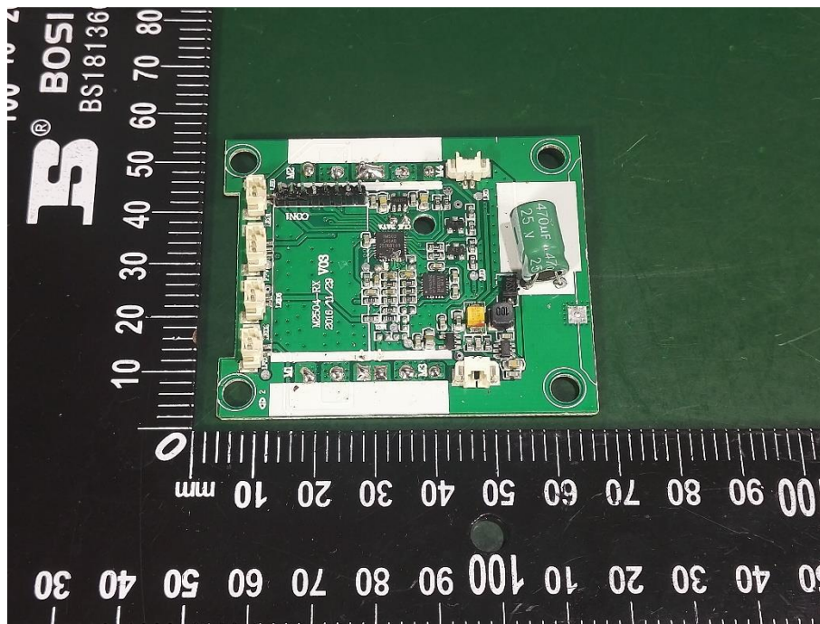
EUT Photo #3 PCB View
