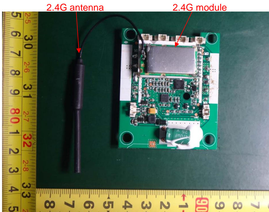
EUT Photo #2 PCB View
