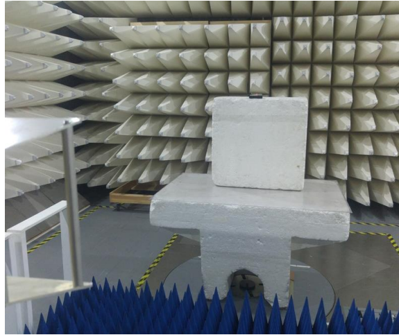
Photograph No.4 Setup for OBW measurements
