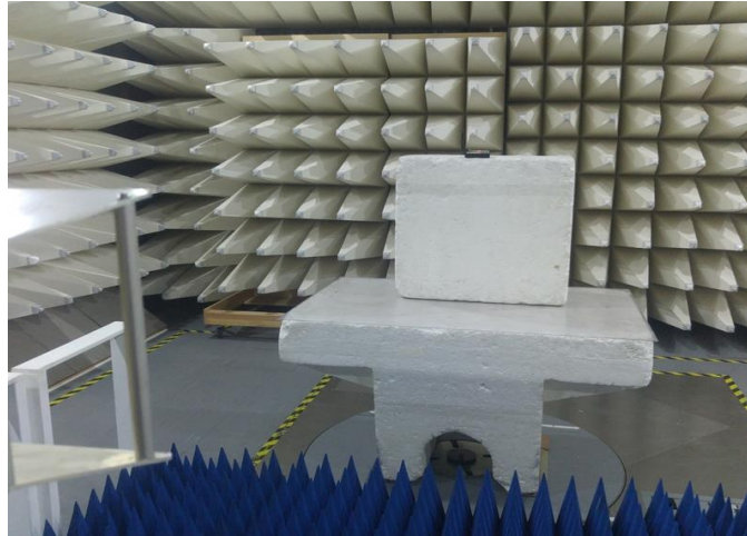
Photograph No.3 Setup for spurious emission field strength measurements in the anechoic chamber above 1000 MHz range
