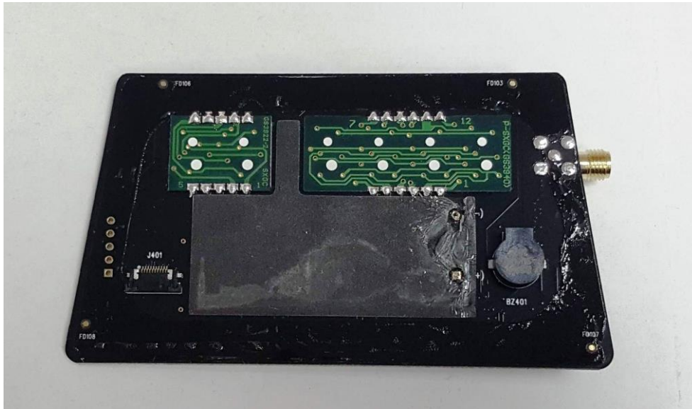
Photograph No.3 i-MTTS-C unit PCB component side
