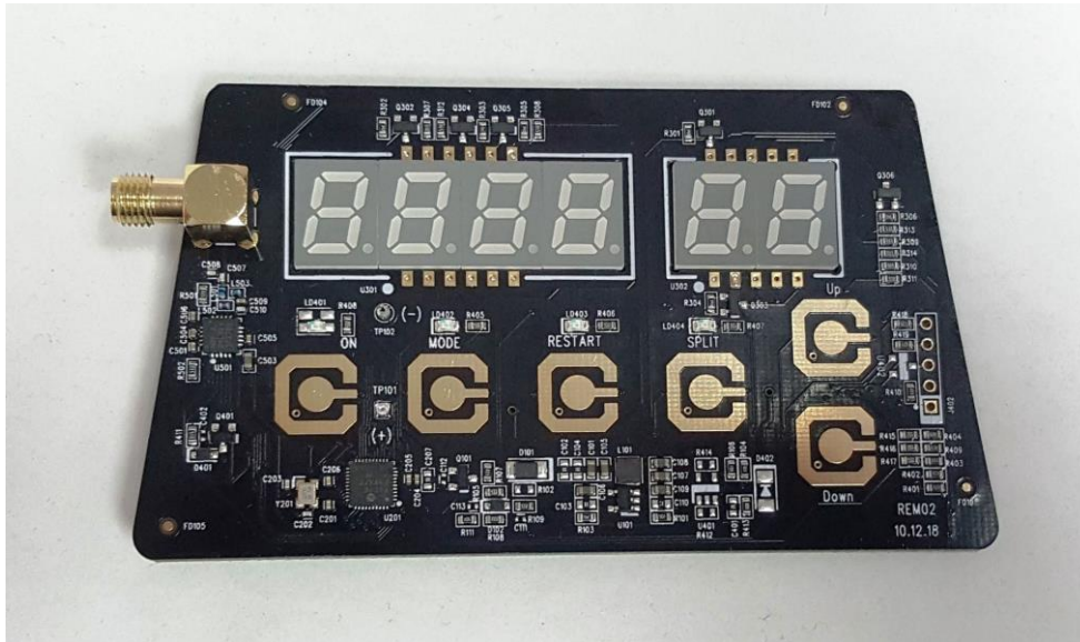
Photograph No.2 i-MTTS-C unit PCB print side
