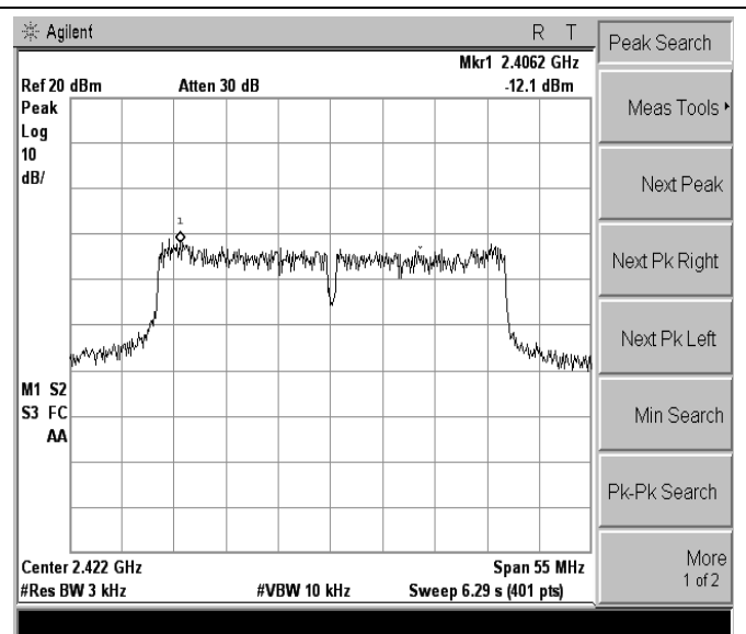
802.11n(HT40)-Low channel
