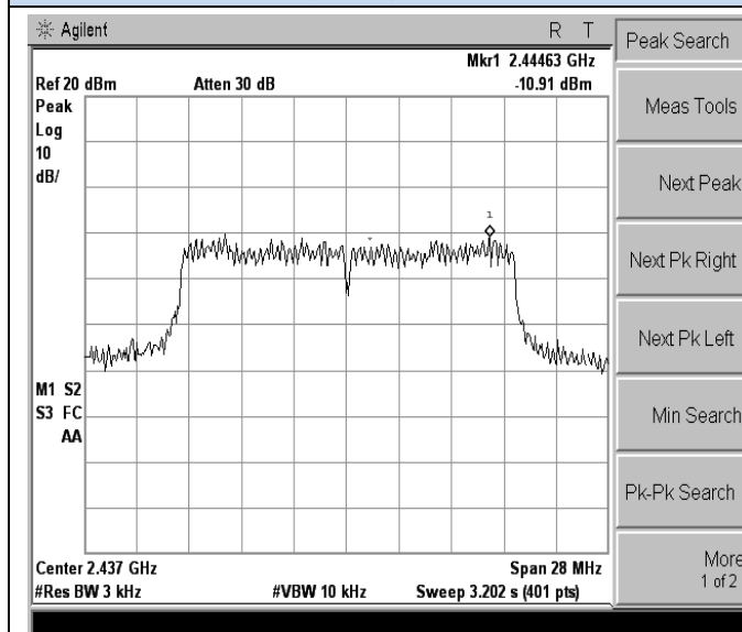
802.11n(HT20)-Middle channel
