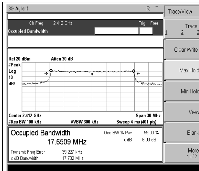
802.11n(HT20)-Low channel
