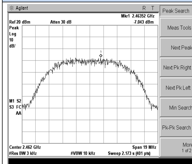
802.11b-High channel
