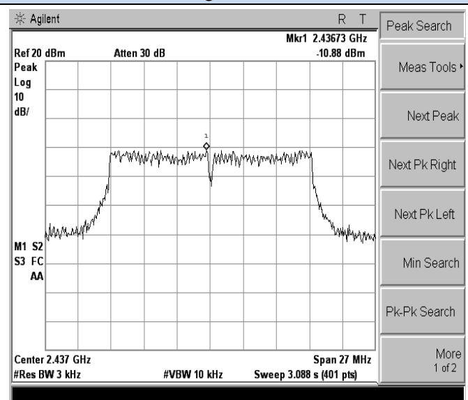
802.11g-Middle channel
