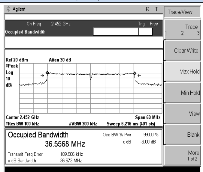
802.11n(HT40)-High channel
