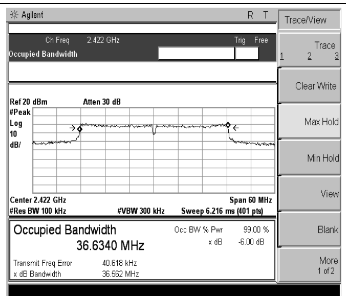
802.11n(HT40)-Low channel
