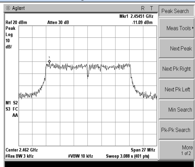
802.11g-High channel
