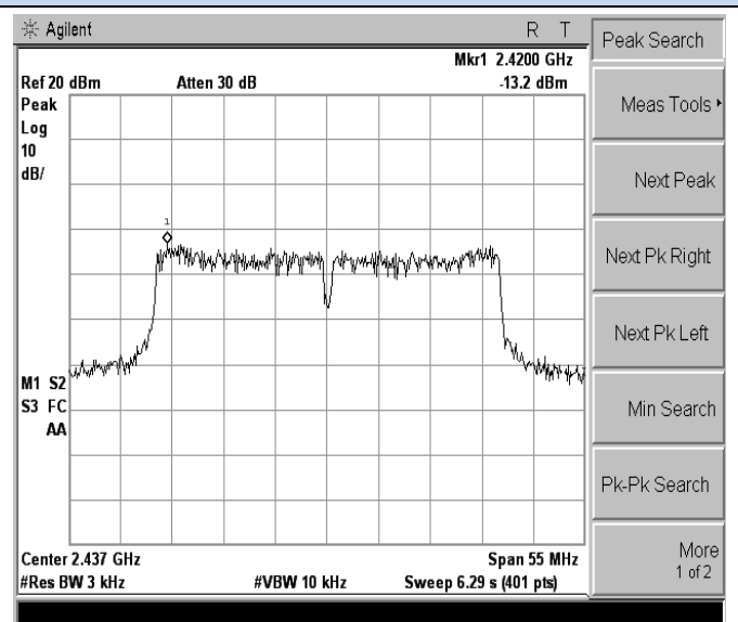
802.11n(HT40)-Middle channel
