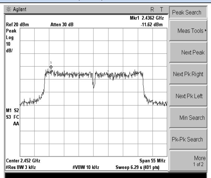
802.11n(HT40)-High channel
