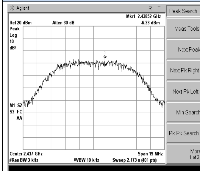
802.11b-Middle channel
