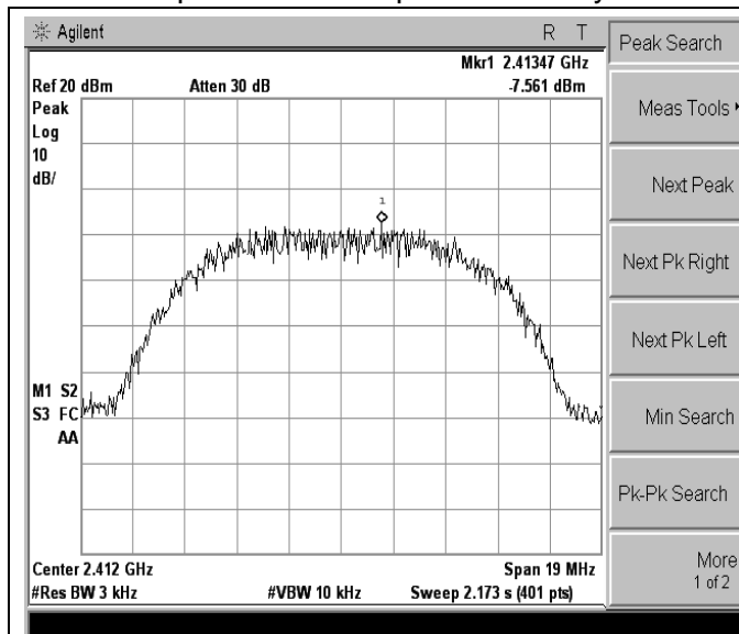
802.11b-Low channel
