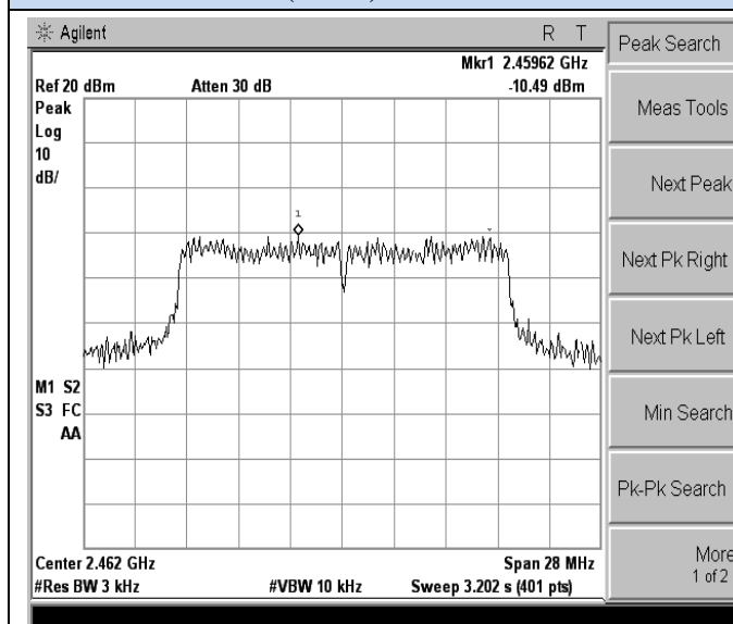
802.11n(HT20)-High channel
