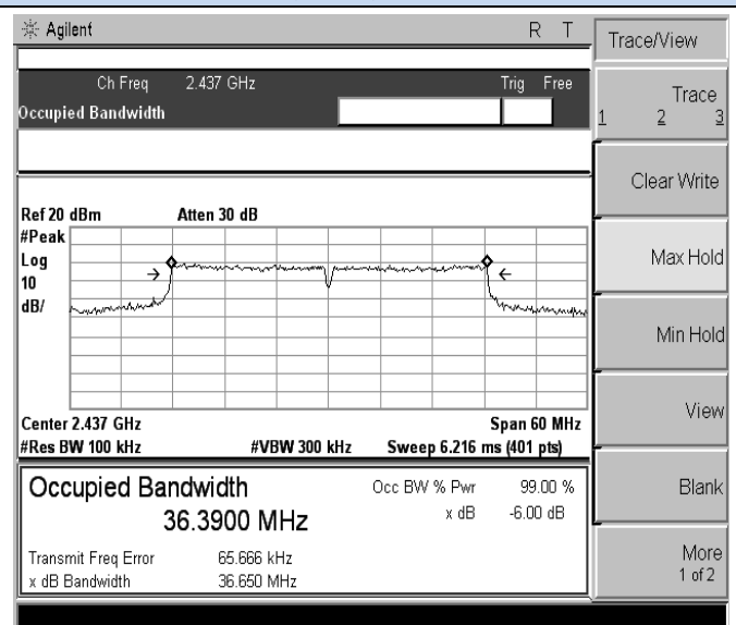
802.11n(HT40)-Middle channel
