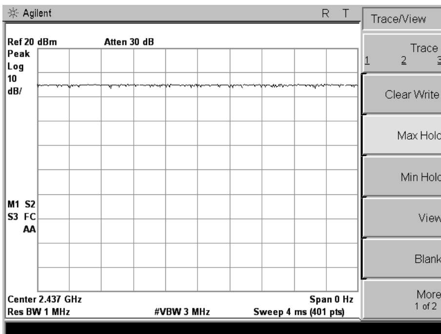
Test plot of Duty Cycle for 802.11n(HT40)
