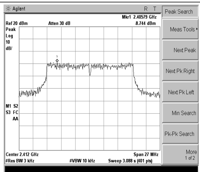
802.11g-Low channel
