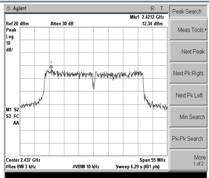
802.11n(HT40)-Middle channel
