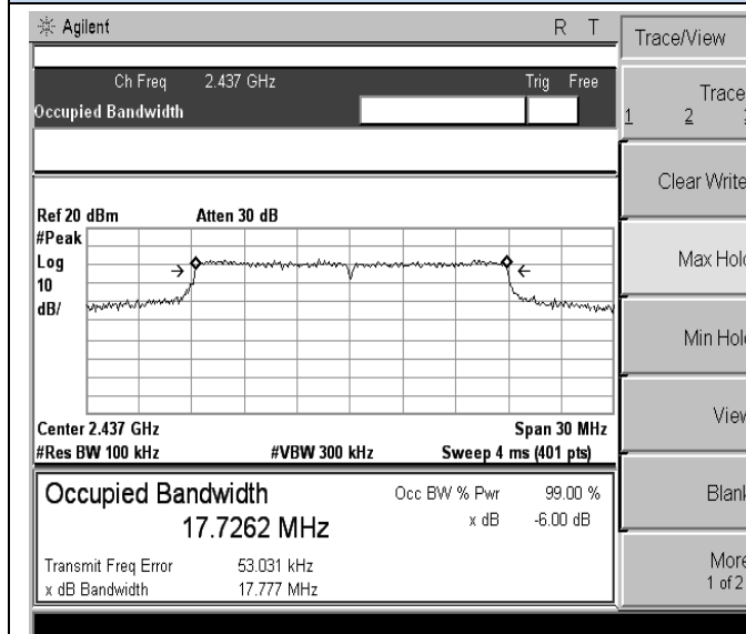
802.11n(HT20)-Middle channel
