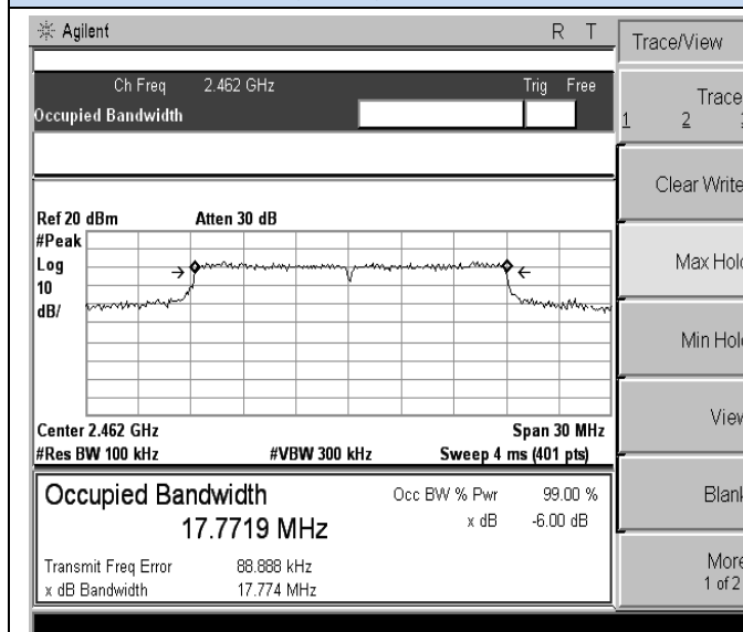
802.11n(HT20)-High channel
