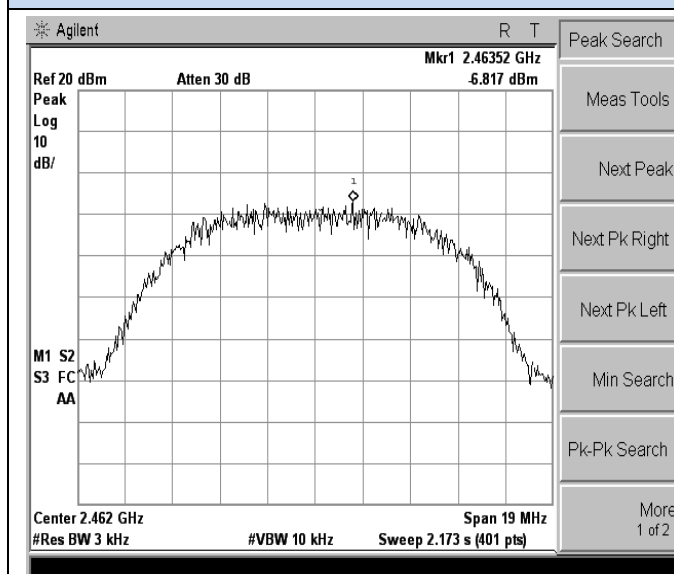
802.11b-High channel
