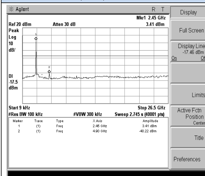
802.11n(HT20)-High channel
