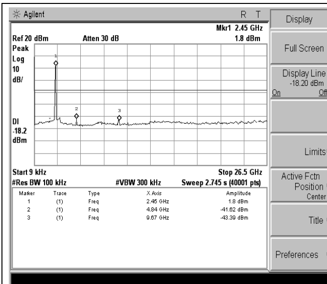
802.11n(HT20)-Low channel
