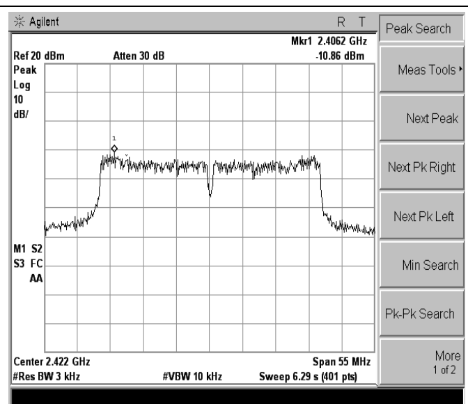
802.11n(HT40)-Low channel
