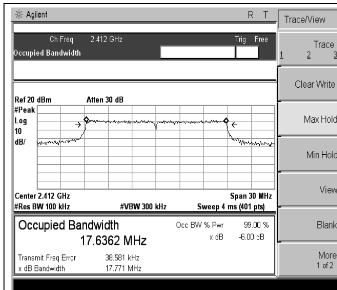
802.11n(HT20)-Low channel
