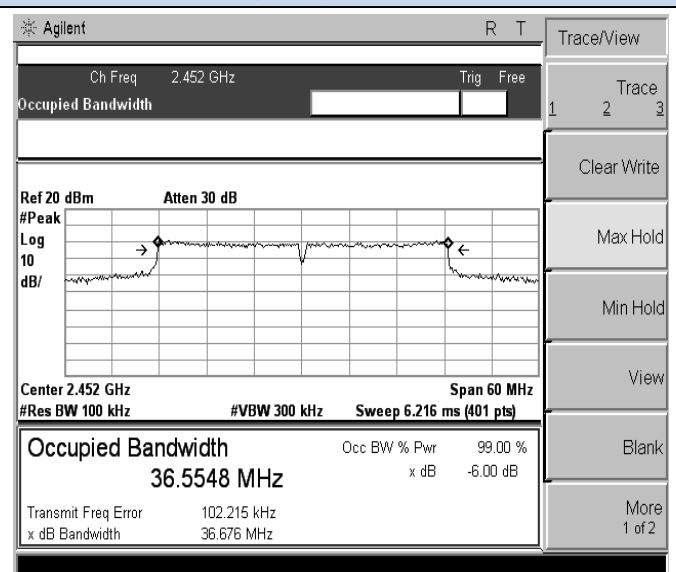
802.11n(HT40)-High channel
