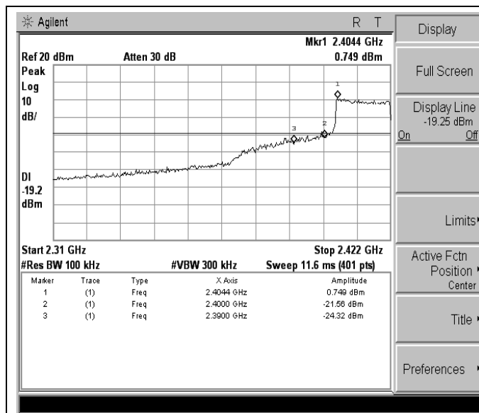
802.11n(HT40)-Low channel
