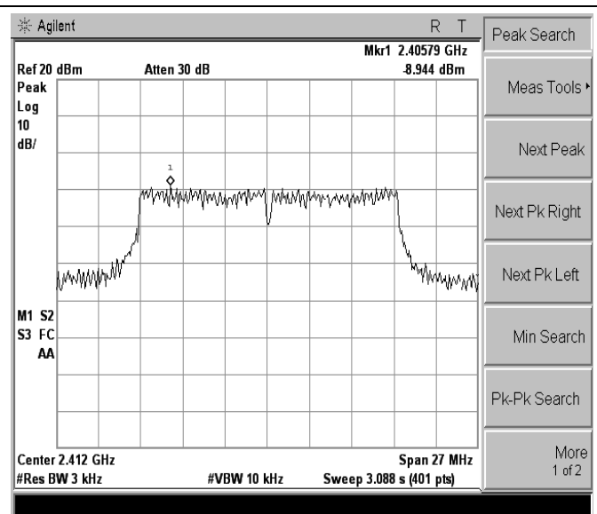
802.11g-Low channel
