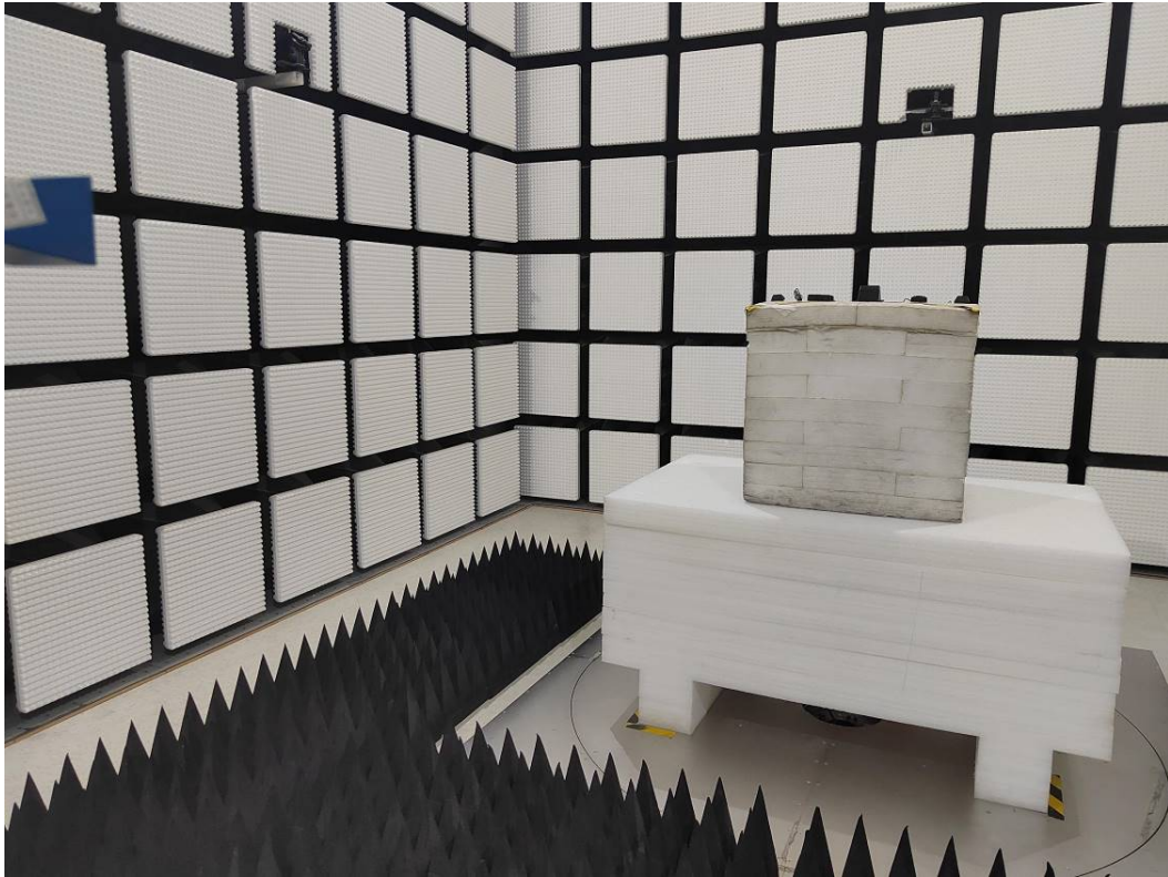
Radiated Emission 26.5-40GHz View
