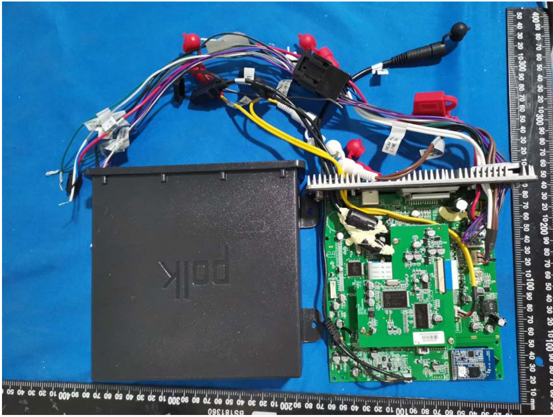
Tuner/Amp Module
