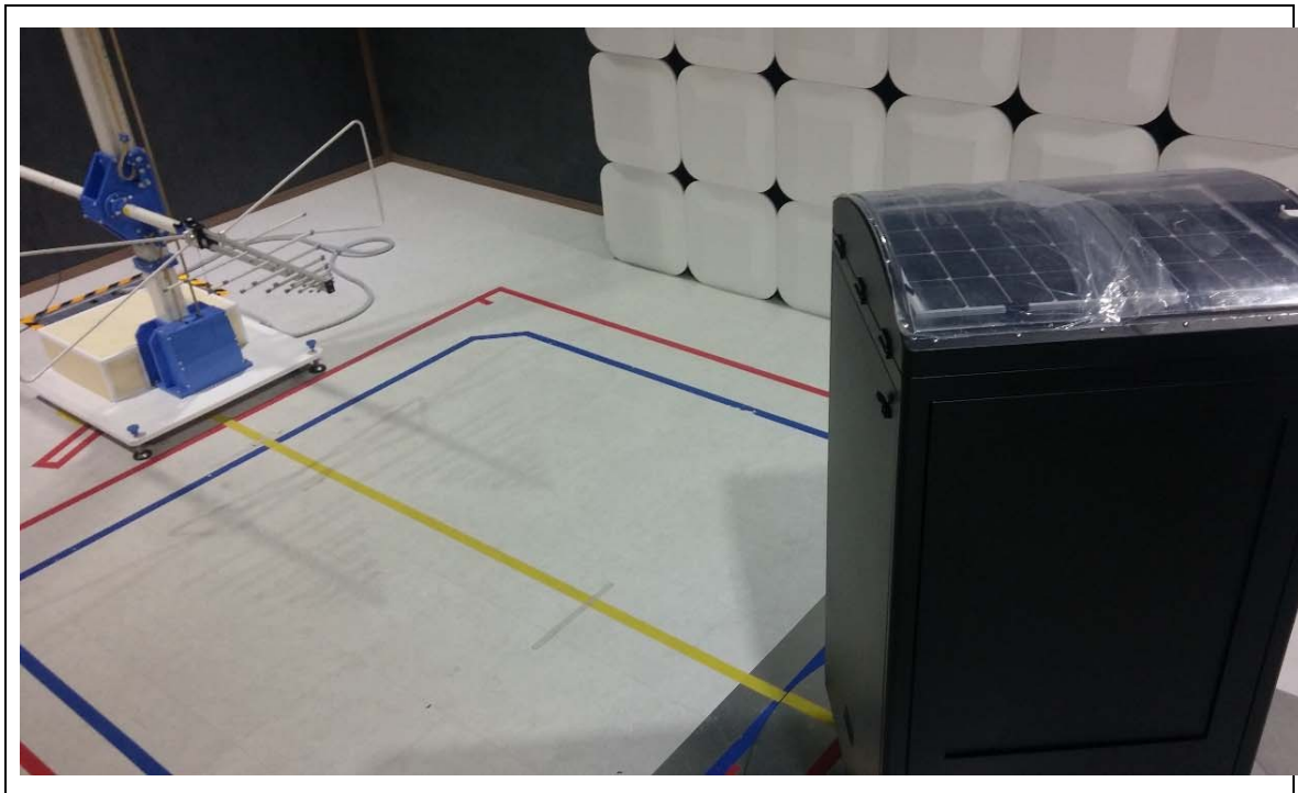
Test Setup Photo of Radiated Measurement (below 1000MHz)
