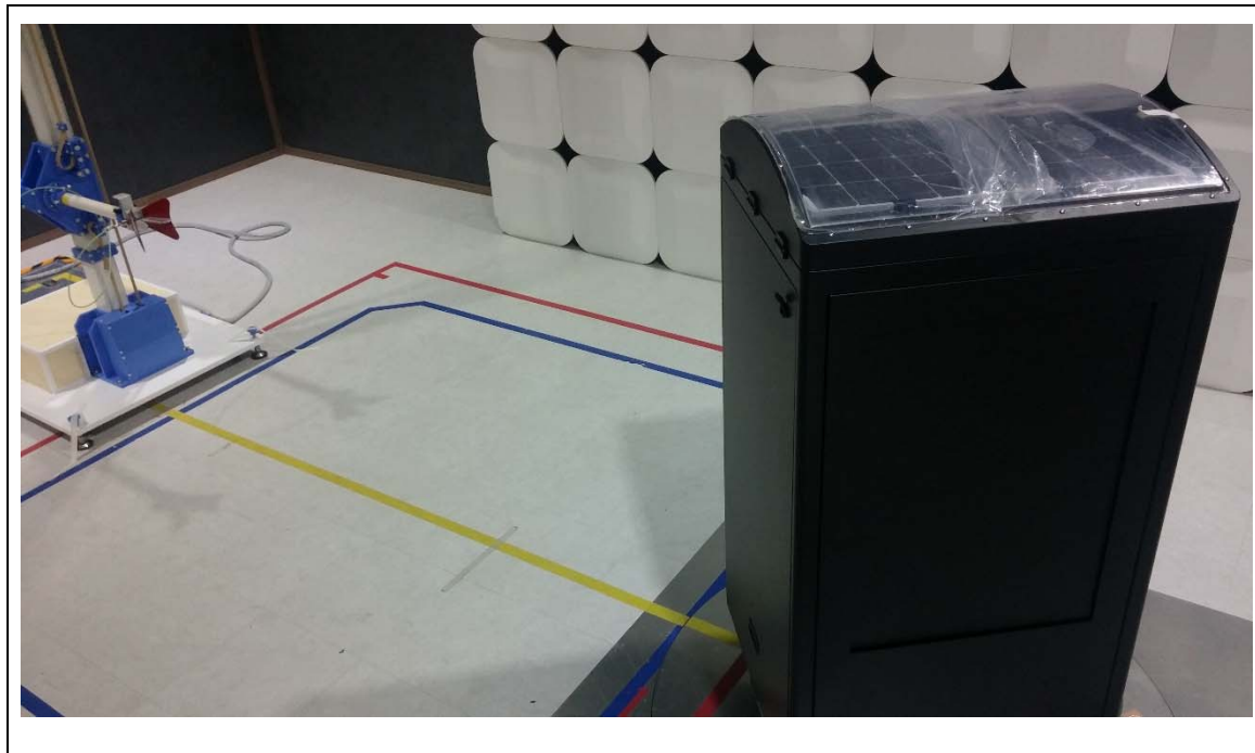
Test Setup Photo of Radiated Measurement (Above 1GHz)
