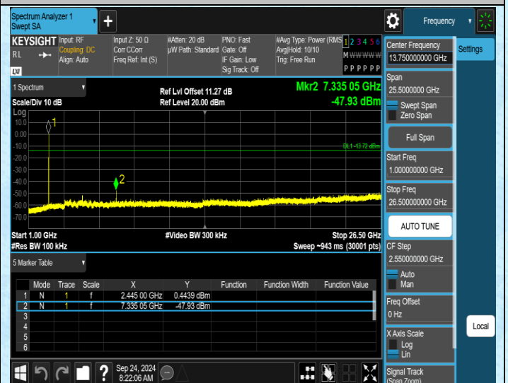
ZIGBEE-Ant1-2445-1000-26500-PASS
