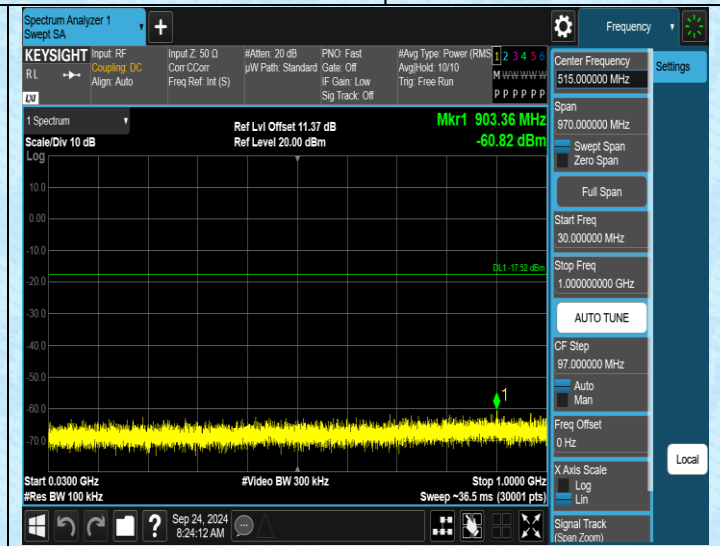
ZIGBEE-Ant1-2480-30-1000-PASS
