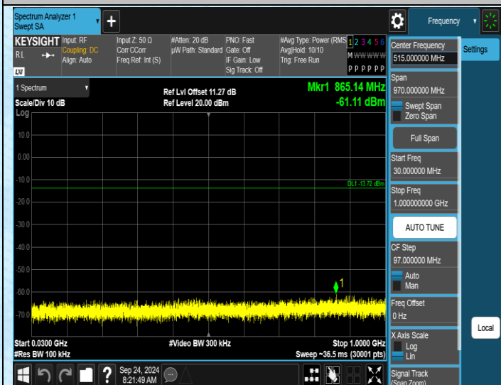
ZIGBEE-Ant1-2445-30-1000-PASS
