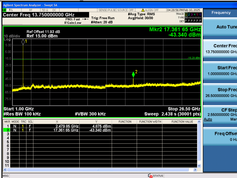
BLE_1M-Ant1-2480MHz-1000~26500-PASS
