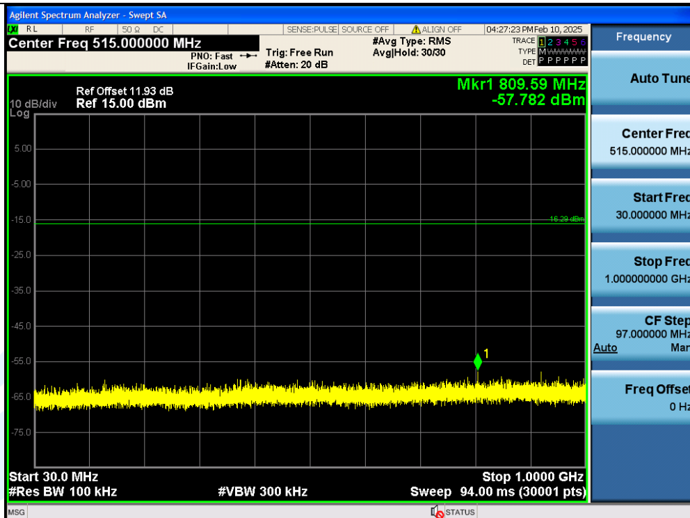
BLE_1M-Ant1-2480MHz-30~1000-PASS
