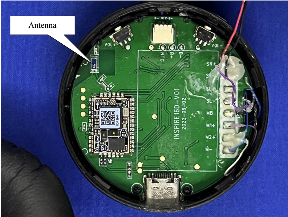
Photo 2: Internal View for PCB
