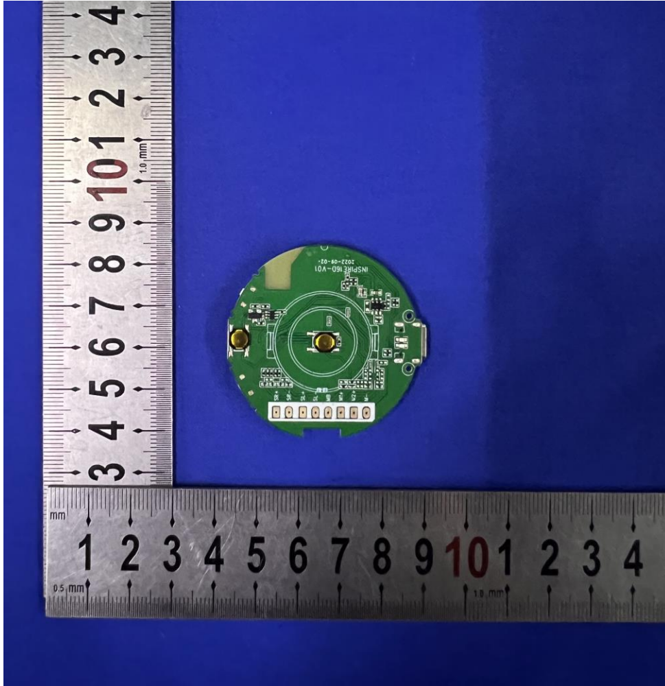
Photo 3: Internal View for PCB
