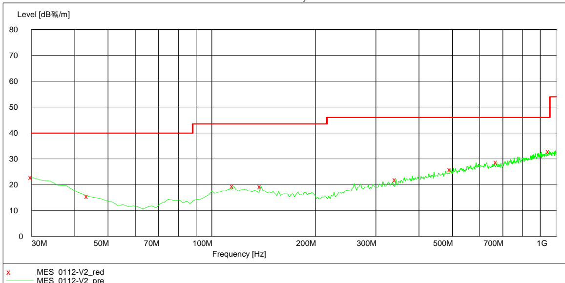
30MHz~1GHz, Vertical
