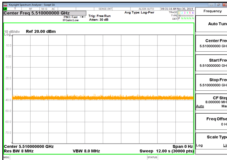
Noise Floor (No transmission)
