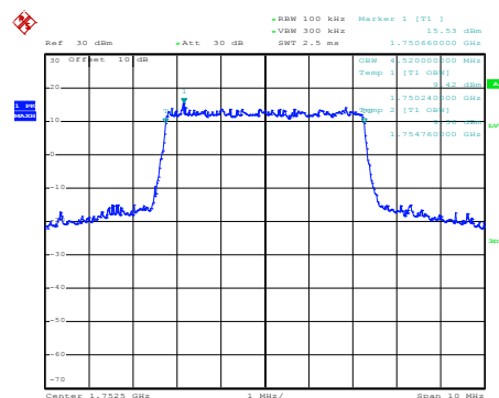
Modulation: QPSK
