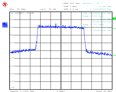
Modulation: 16QAM
