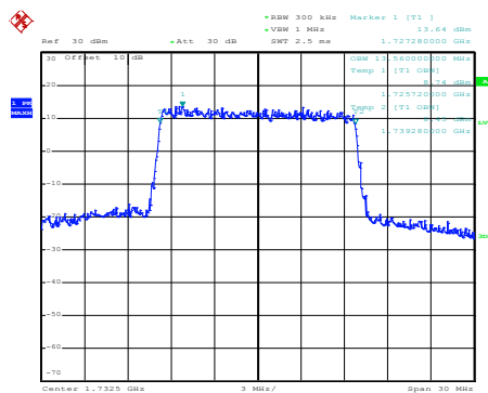
Modulation:16QAM
