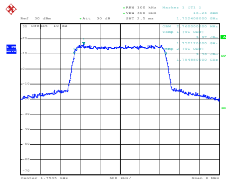
Modulation: QPSK
