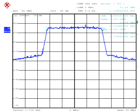
Modulation: QPSK
