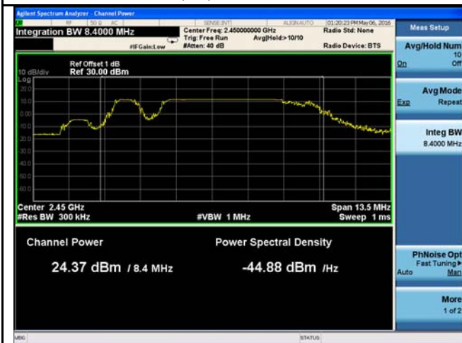
Output power - CH 2450
