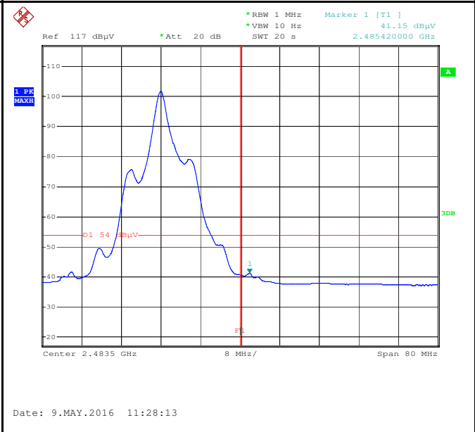
Band Edge, Right Side (Average)
