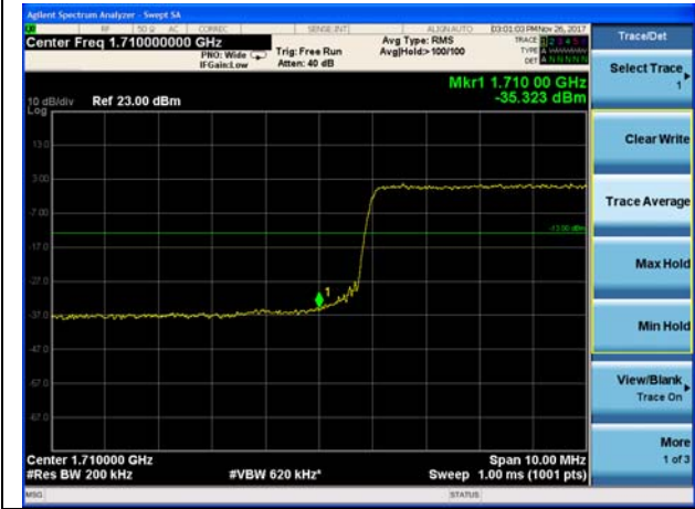
LTE Band 4 16QAM 20MHz CH-Low, 100%RB
