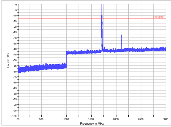
LTE Band 4 5MHz CH-Middle 30MHz~3GHz
