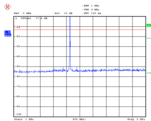
LTE Band 2 5MHz CH-Low 1GHz~3GHz
