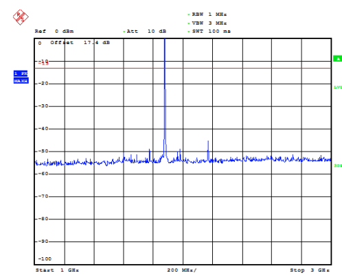
LTE Band 2 5MHz CH-Middle 1GHz~3GHz
