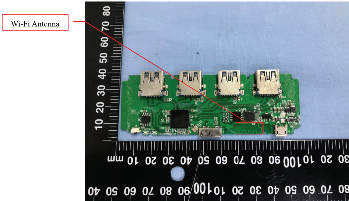
Solder Board-Component View 2
