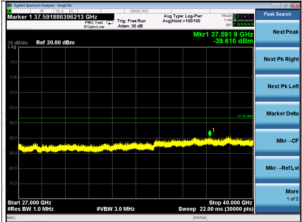
Test_Graph_802.11n40_ANT2_5230_MCS0_Frequency Band 5
