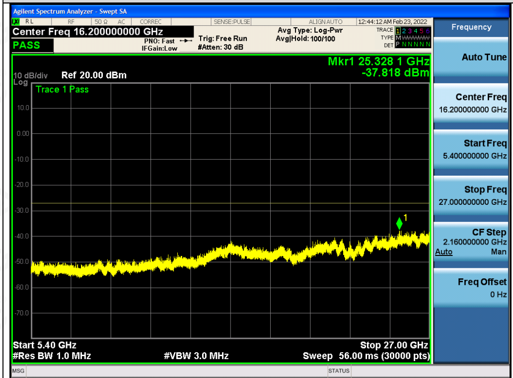
Test_Graph_802.11n40_ANT2_5190_MCS0_Frequency Band 4
