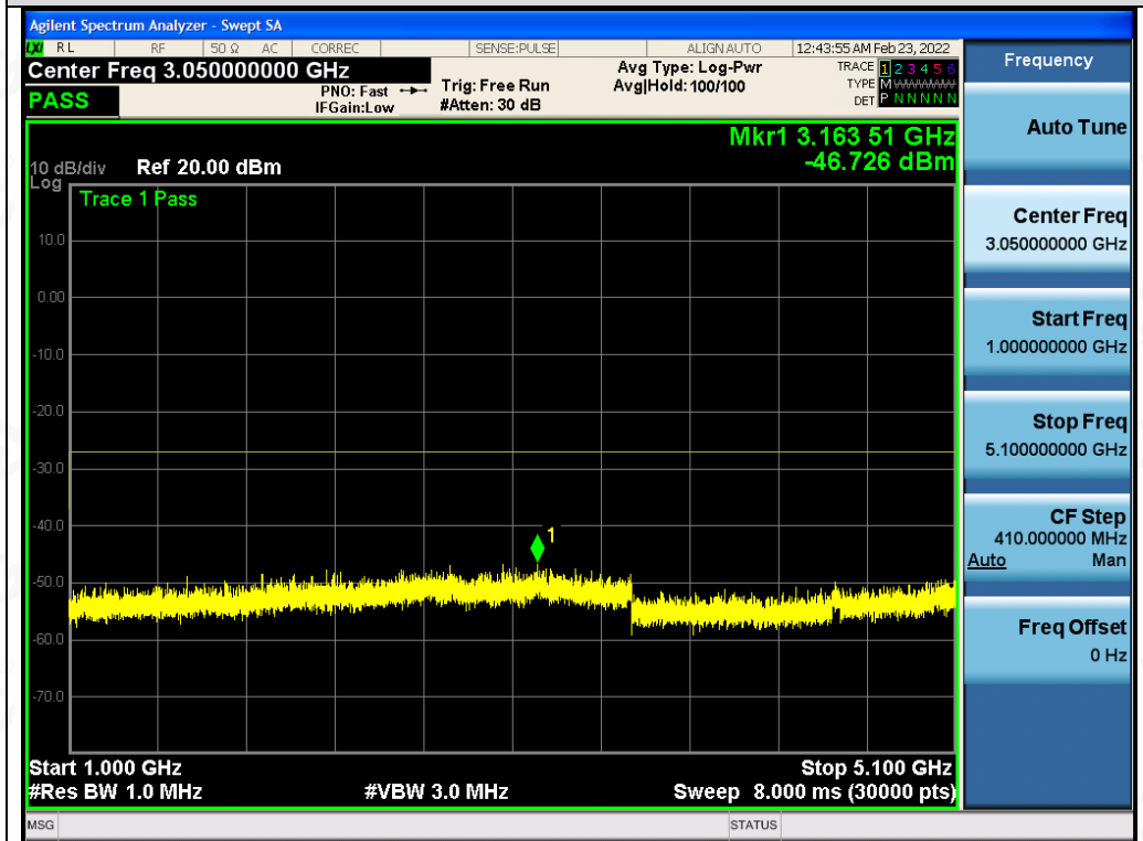
Test_Graph_802.11n40_ANT2_5190_MCS0_Frequency Band 2
