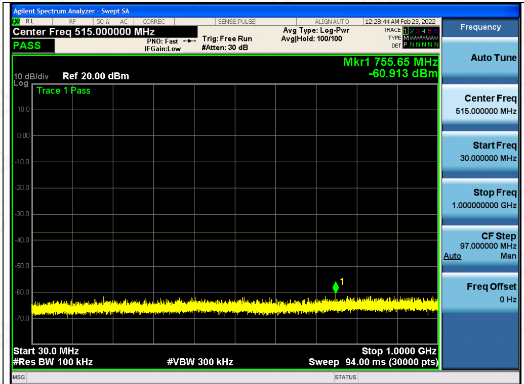
Test_Graph_802.11a_ANT2_5180_6Mbps_Frequency Band 1
