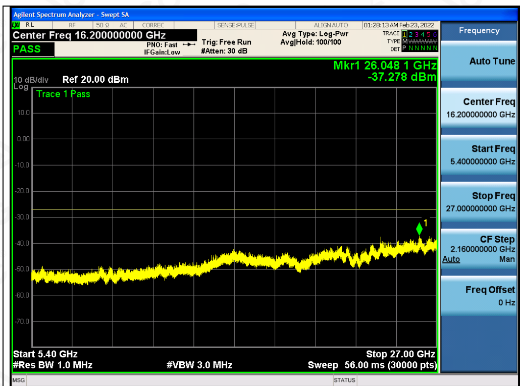
Test_Graph_802.11n40_ANT2_5310_MCS0_Frequency Band 4
