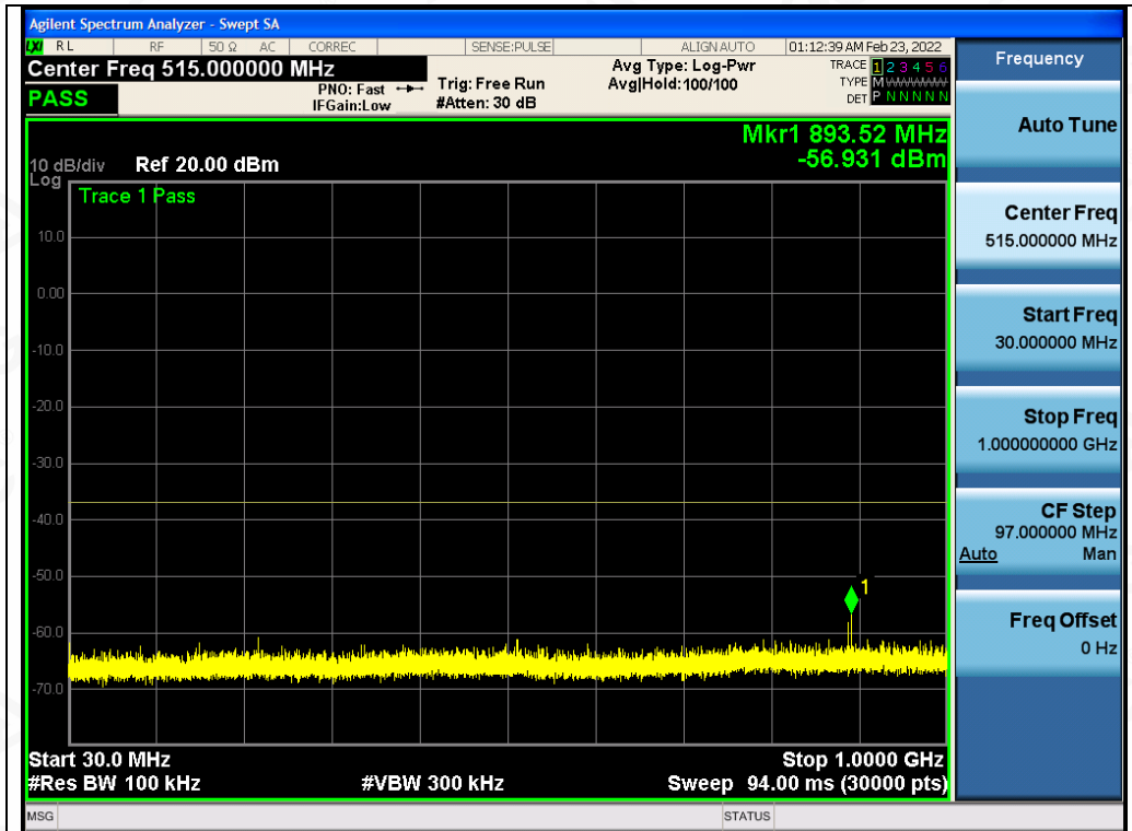
Test_Graph_802.11a_ANT2_5260_6Mbps_Frequency Band 1
