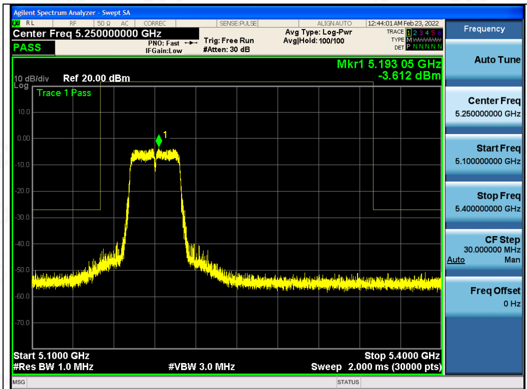
Test_Graph_802.11n40_ANT2_5190_MCS0_Frequency Band 3
