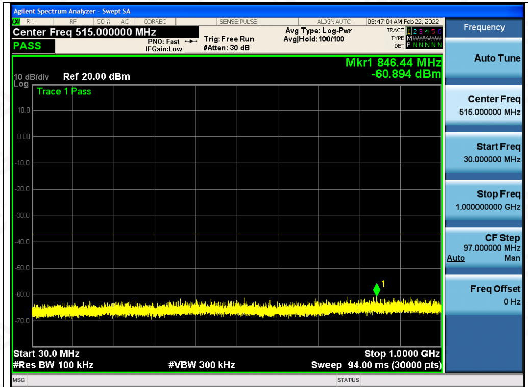
Test_Graph_802.11ac80_ANT1_5610_MCS9_Frequency Band 1
