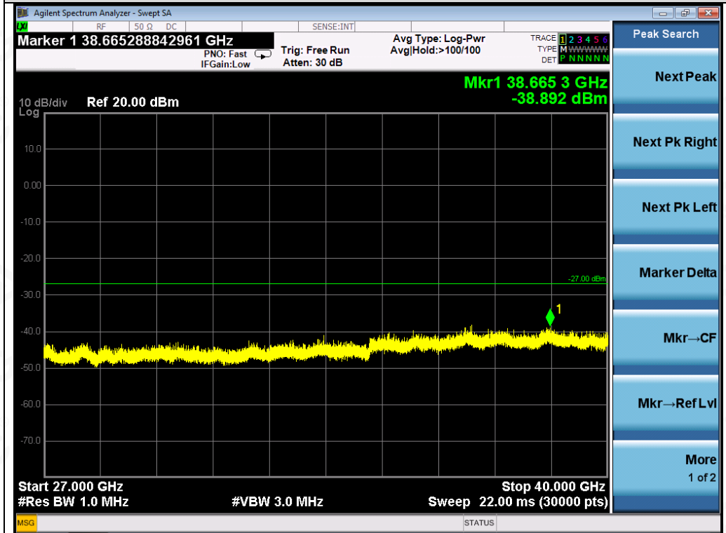
Test_Graph_802.11a_ANT2_5500_6Mbps_Frequency Band 5
