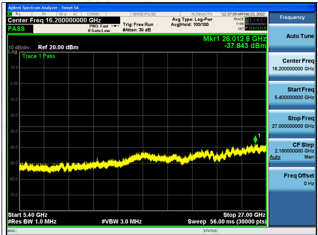
Test_Graph_802.11a_ANT2_5240_6Mbps_Frequency Band 4
