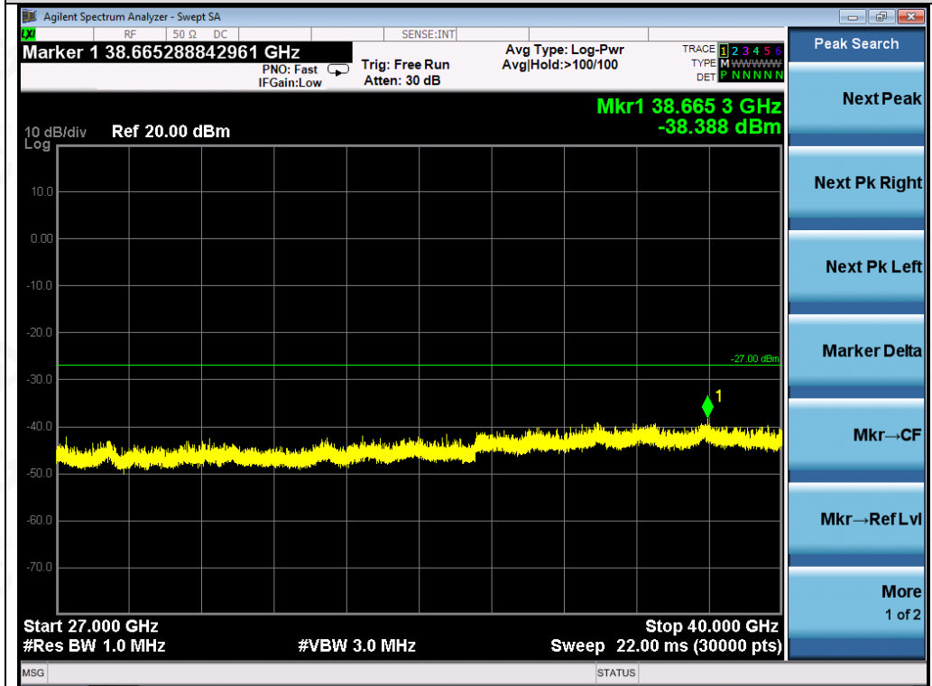
Test_Graph_802.11a_ANT2_5240_6Mbps_Frequency Band 5
