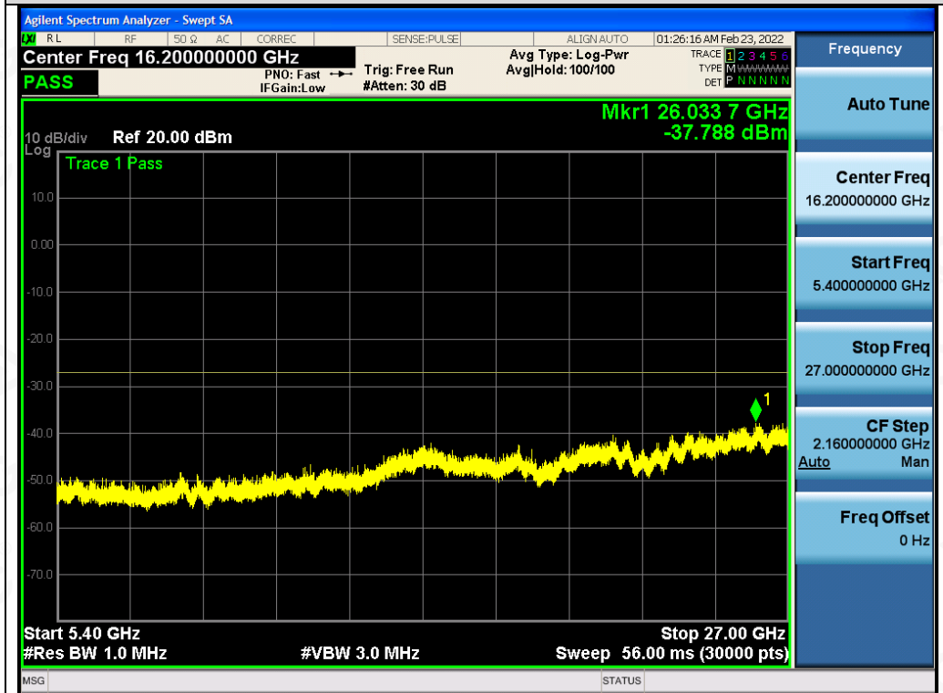
Test_Graph_802.11n40_ANT2_5270_MCS0_Frequency Band 4
