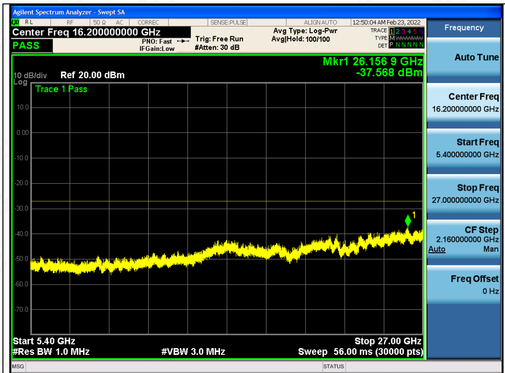
Test_Graph_802.11n40_ANT2_5230_MCS0_Frequency Band 4
