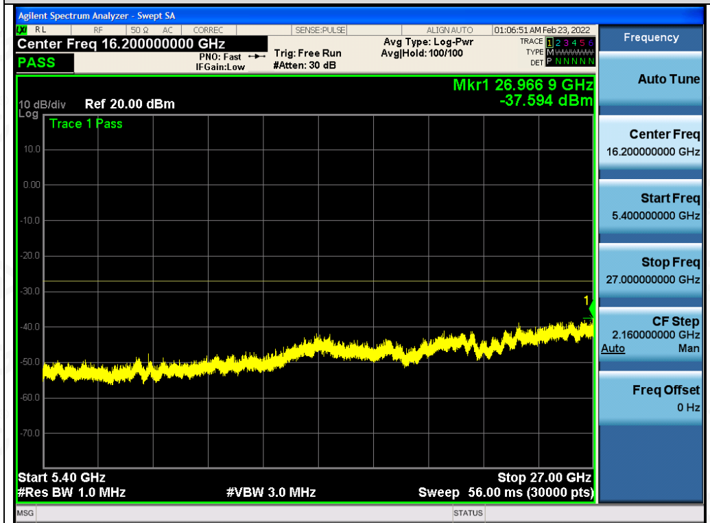
Test_Graph_802.11ac80_ANT2_5210_MCS9_Frequency Band 4
