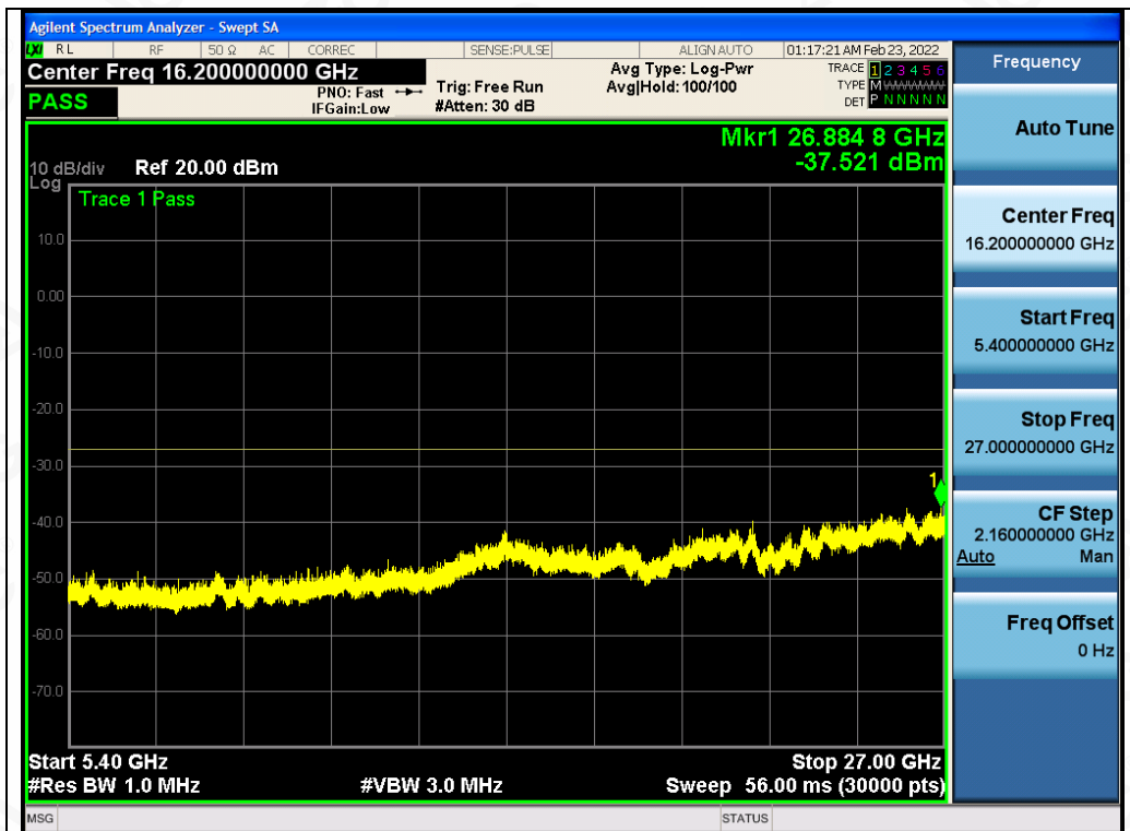
Test_Graph_802.11a_ANT2_5320_6Mbps_Frequency Band 4
