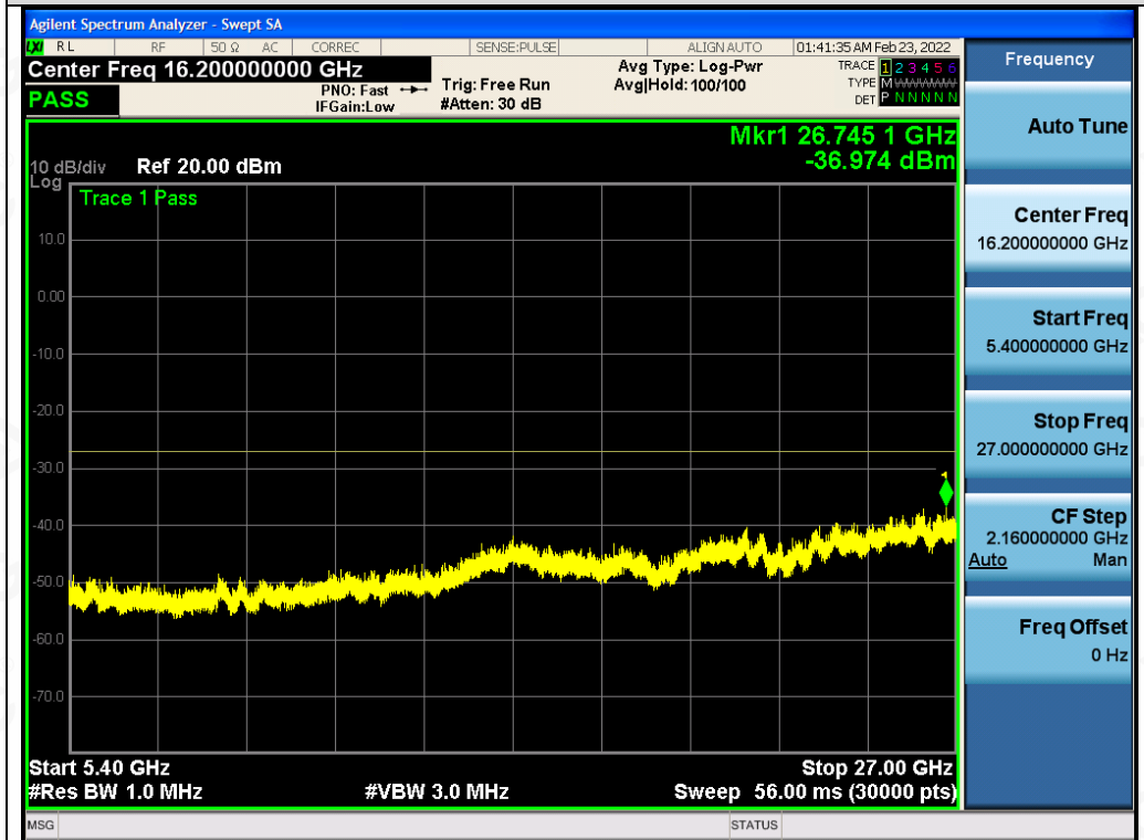
Test_Graph_802.11ac80_ANT2_5290_MCS9_Frequency Band 4
