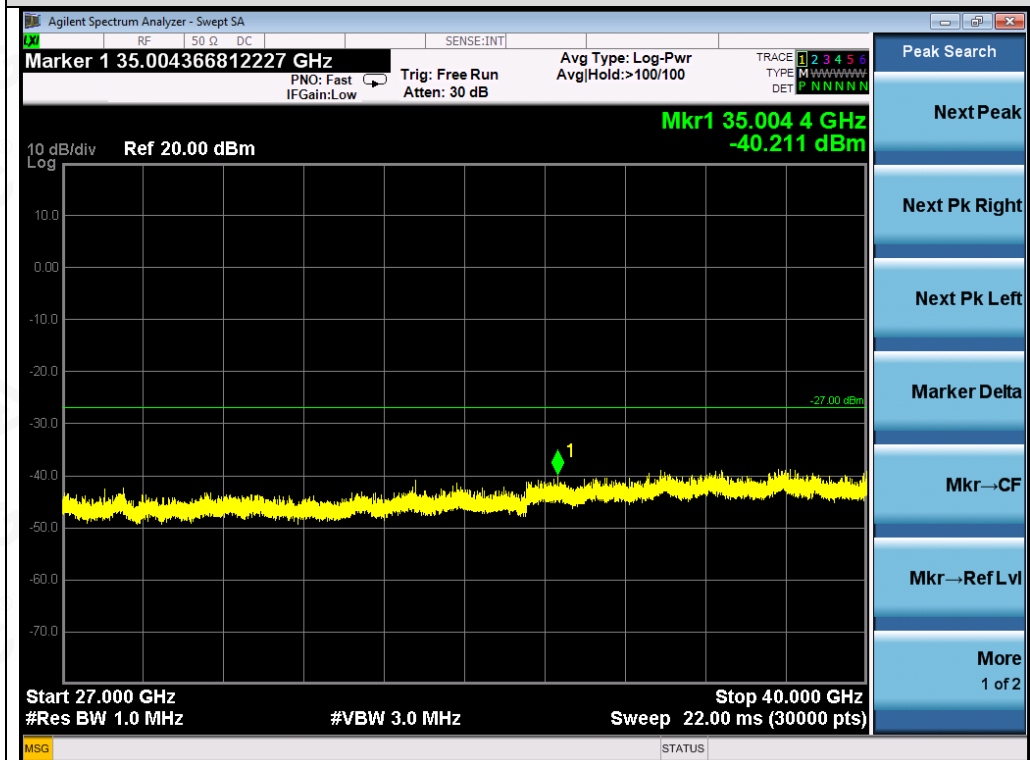
Test_Graph_802.11n40_ANT2_5310_MCS0_Frequency Band 5
