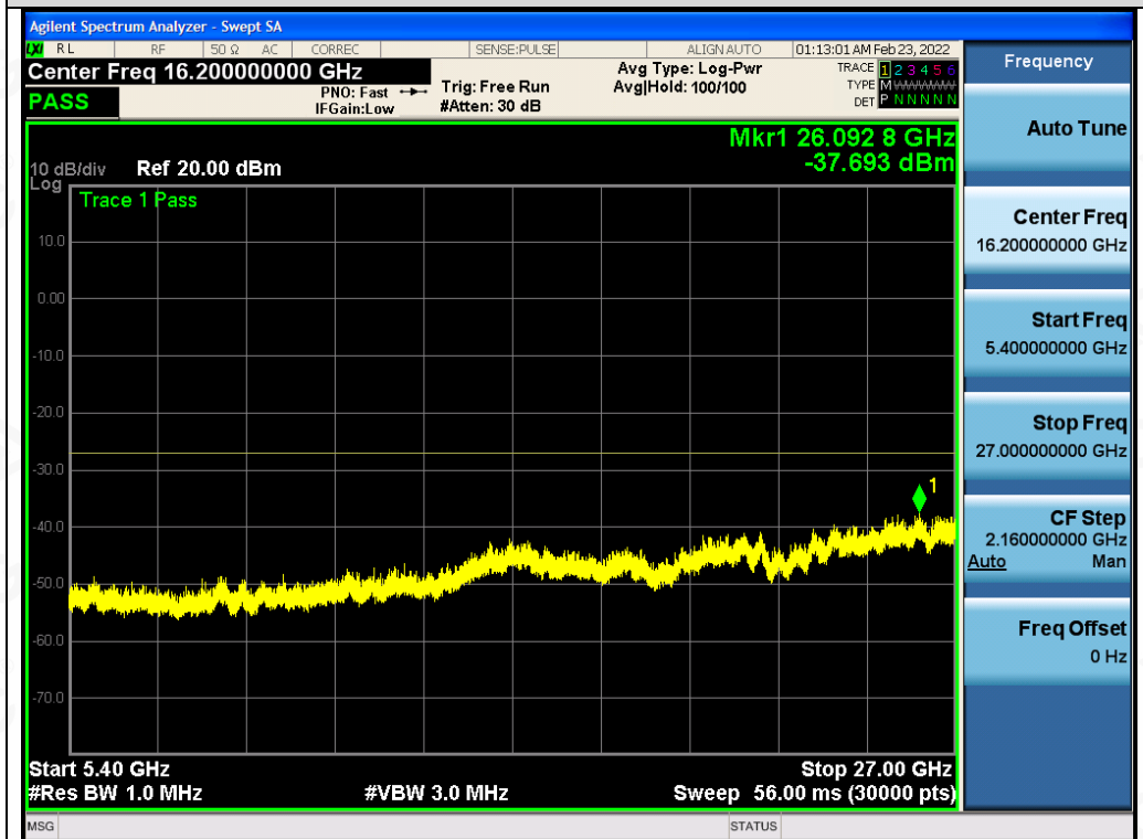
Test_Graph_802.11a_ANT2_5260_6Mbps_Frequency Band 4
