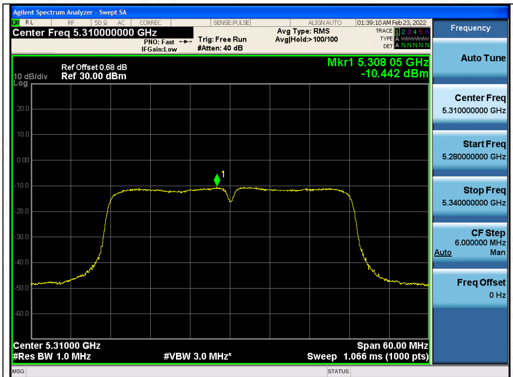
Test_Graph_802.11ac40_ANT2_5310_MCS9_PSD
