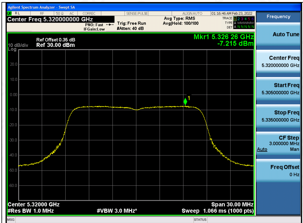
Test_Graph_802.11a_ANT2_5320_6Mbps_PSD
