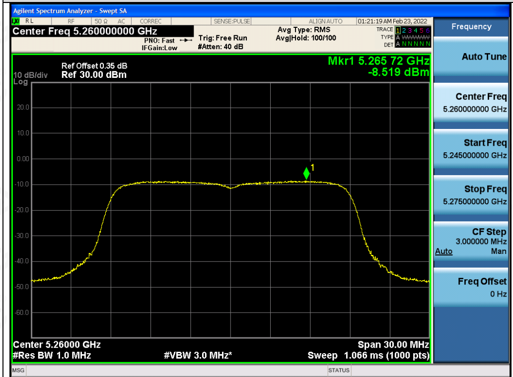
Test_Graph_802.11n20_ANT2_5260_MCS0_PSD
