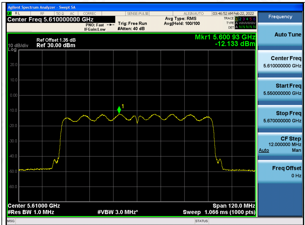
Test_Graph_802.11ac80_ANT1_5610_MCS9_PSD
